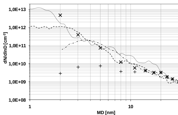
Fig. 4 Size distribution function obtained by AFM image analysis compared to those measured with the DMA. (+ not corrected; × corrected for collection efficiency).
