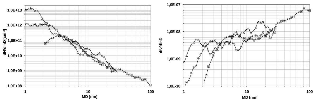
Fig. 2 Number (left) and volume (right) size distribution functions measured with the DMA. ( \Delta DR \sim 3 \cdot 10^4 ; \circ DR \sim 4 \cdot 10^3 ; \square DR \sim 1 \cdot 10^3 ).
