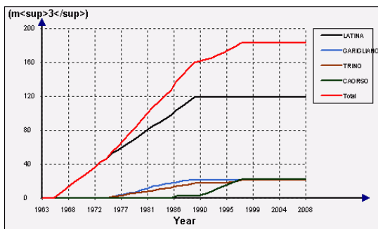
Figura 20: HLW in stock
