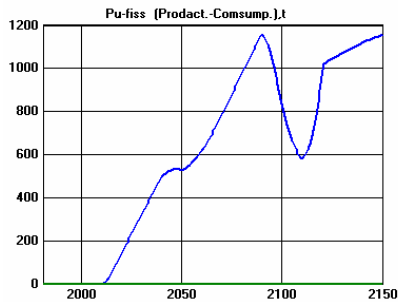
Figure 3: R-2: Production- consumption of fissile Pu for a 33% SFR-R share up to 2100
