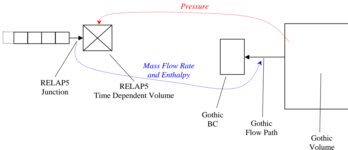
Figure 1. Arrangement of the initial coupling routine for the transfer of variables related to a water blowdown
