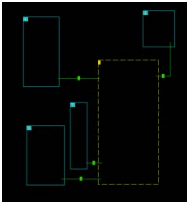
Figure 2. Arrangement of Gothic volumes, flow paths and boundary conditions corresponding to two RELAP5 junctions connected to Gothic
