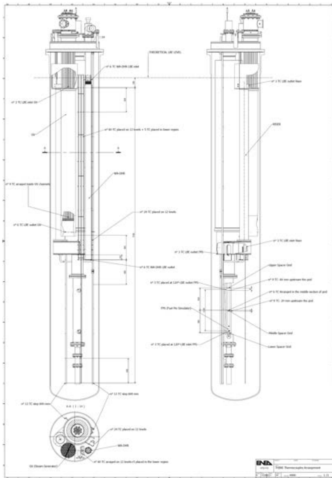
Figure 35. Sketch of the upgrade ICE test section with the installed instrumentations.
