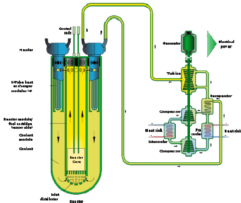
Figure 1 – Sketch of Lead Fast Reactor.
