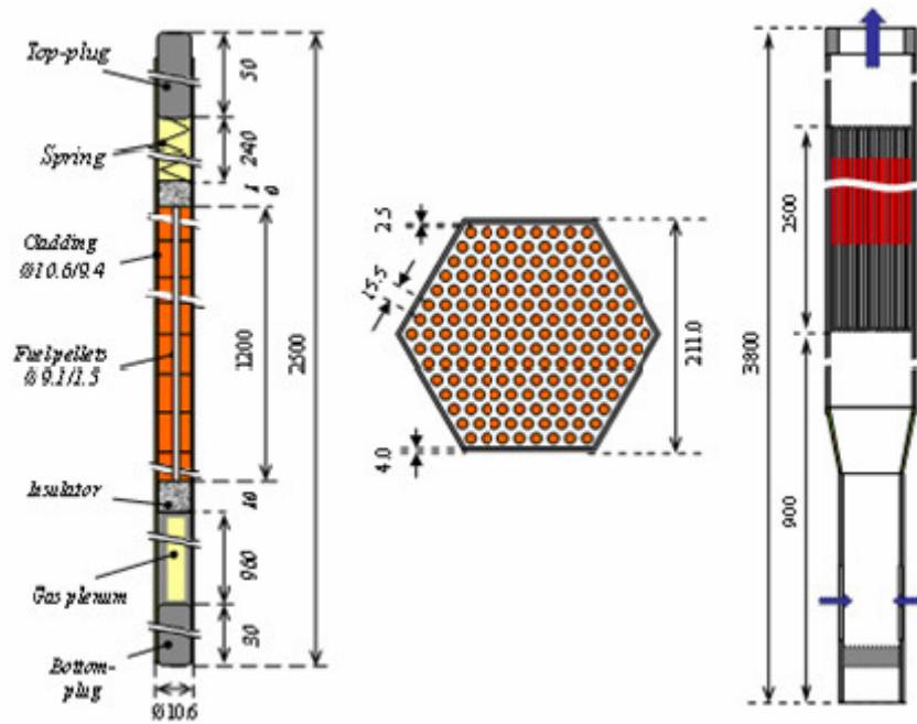
Figure 3 – Schematic view of fuel rod and sub-assembly
