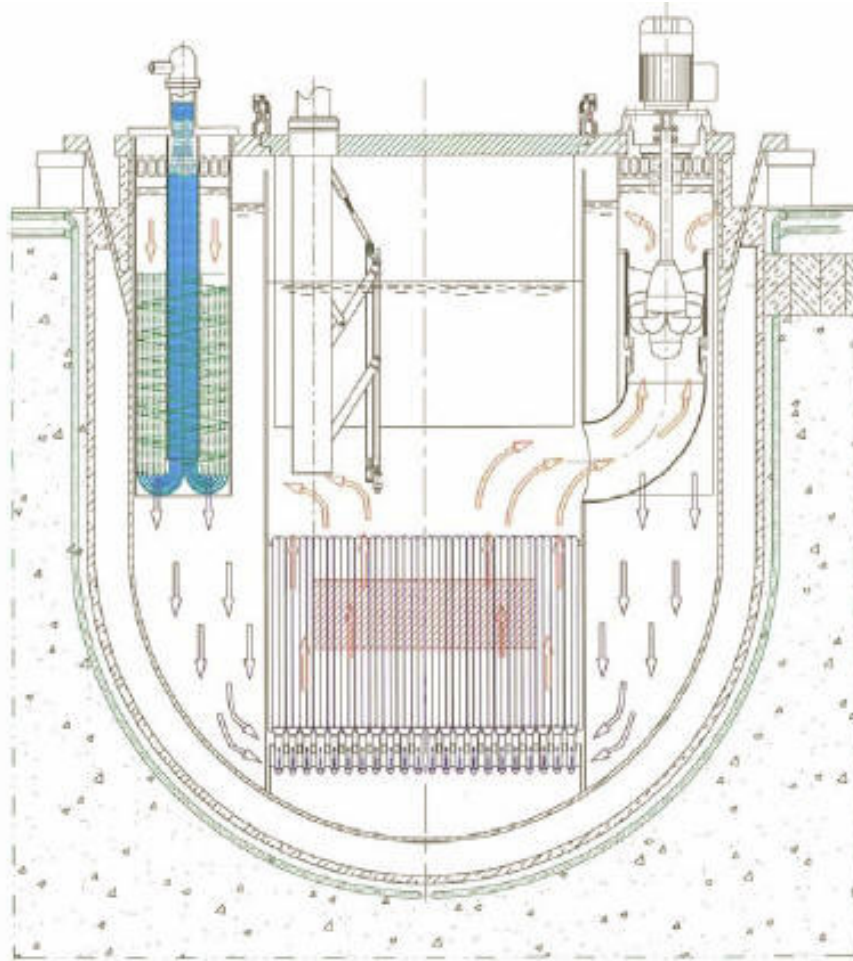
Figure 2 - Overview of the ELSY Reactor Vessel and main flow path
