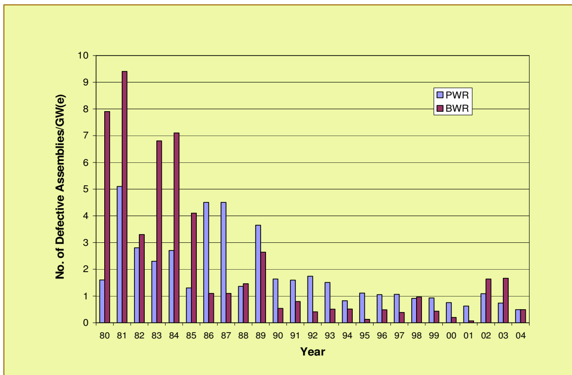
Figure 5 – Fuel failure trends
