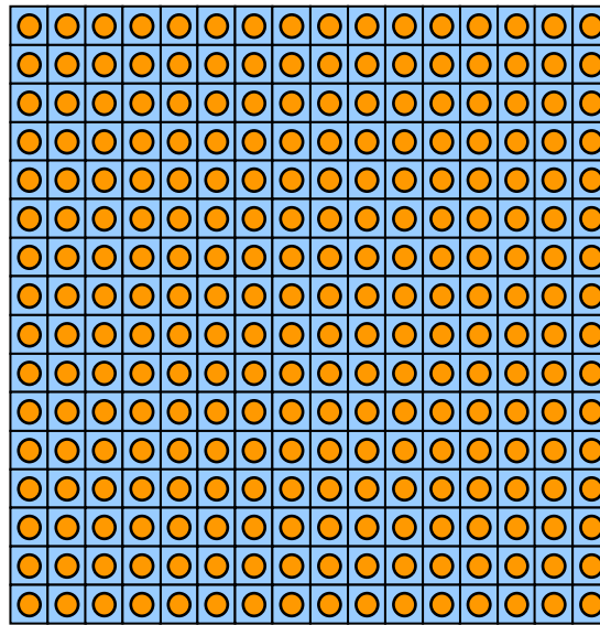
Fig. 2 – Sketch of a fuel bundle scheme for a water reactor.
