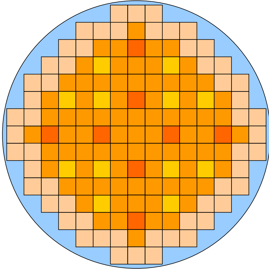
Fig. 3 – Schematics of full core geometry.
