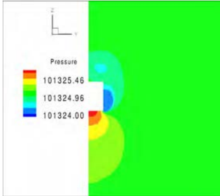
Figure 4: Flow past a cube: color map of pressure in a plane x-z, and y=0.
