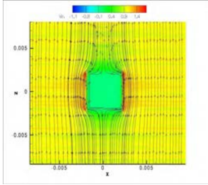
Figure 5: Flow past a cube: color map of axial velocity component and streamtraces in a plane x-z, and y=0 .
