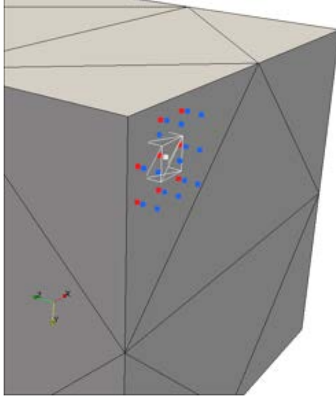
Figure 3: Example of points cloud used for the interpolation of scalar variables. White bullet: the centroid of the cutted cell; white line: volume of fluid of the cutted cell; red bullets: the interpolation points used for the boundary condition; blue bullets: the surrounding volume of fluid centroids.
