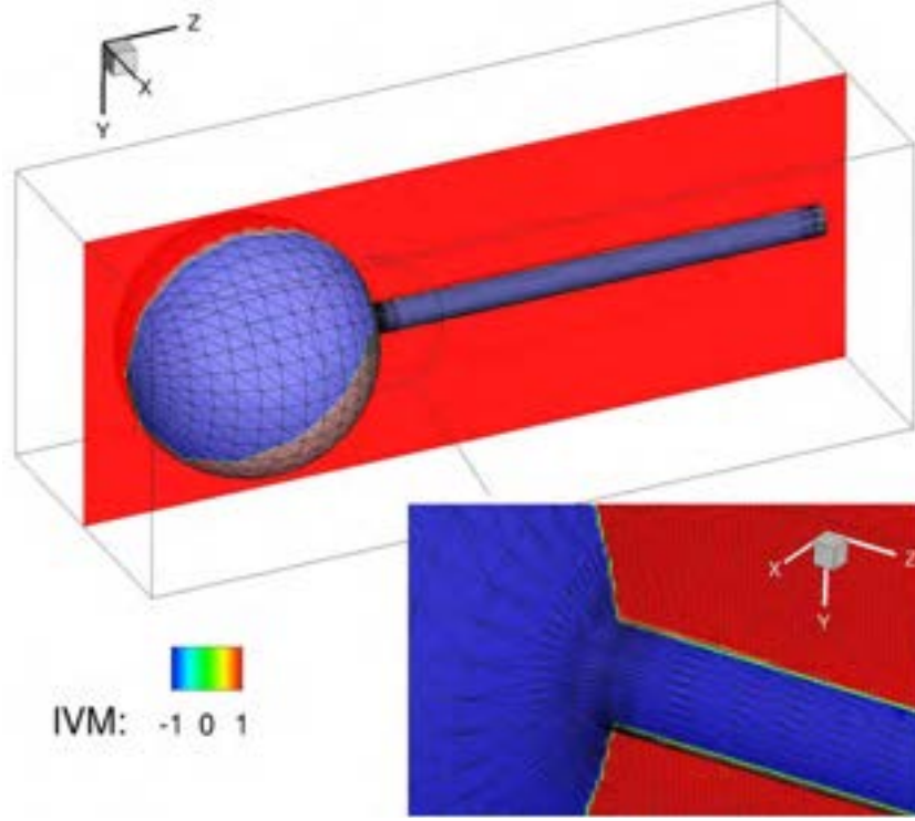
Figure 1: Top: A three-dimensional Cartesian grid illustrating the three types of cells in the cut-cell approach. The red region ( IVM = 1 ) denotes the fluid cells which lie entirely outside the internal boundary, whereas the blue cells ( IVM = -1 ) denote the solid cells which lie entirely inside the internal boundary. The green cells ( IVM = 0 ) correspond to the cut-cells which are intersected by the internal boundary; Bottom: zoomed-in-view of the immersed boundary region where computational cartesian grid is shown.
