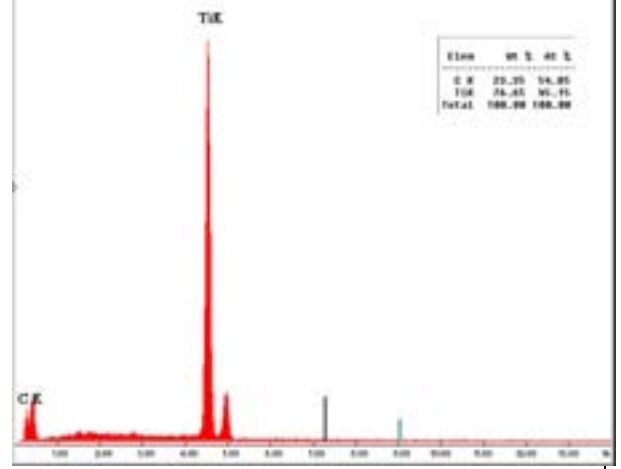
14-EDS 04 – SEM – 20kV – count 1900 – sec= 60
