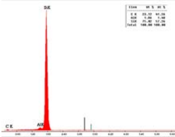
13-EDS 03 – SEM – 20kV – count 1900 – sec= 60
