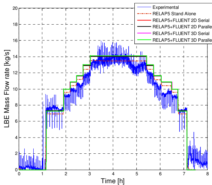
Figure 9: LBE mass flow rate results for Test 206
