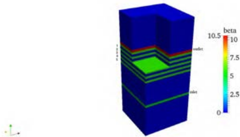
Figure 2.26: Case B. Spatial distribution of the pressure drop coefficient \beta .
