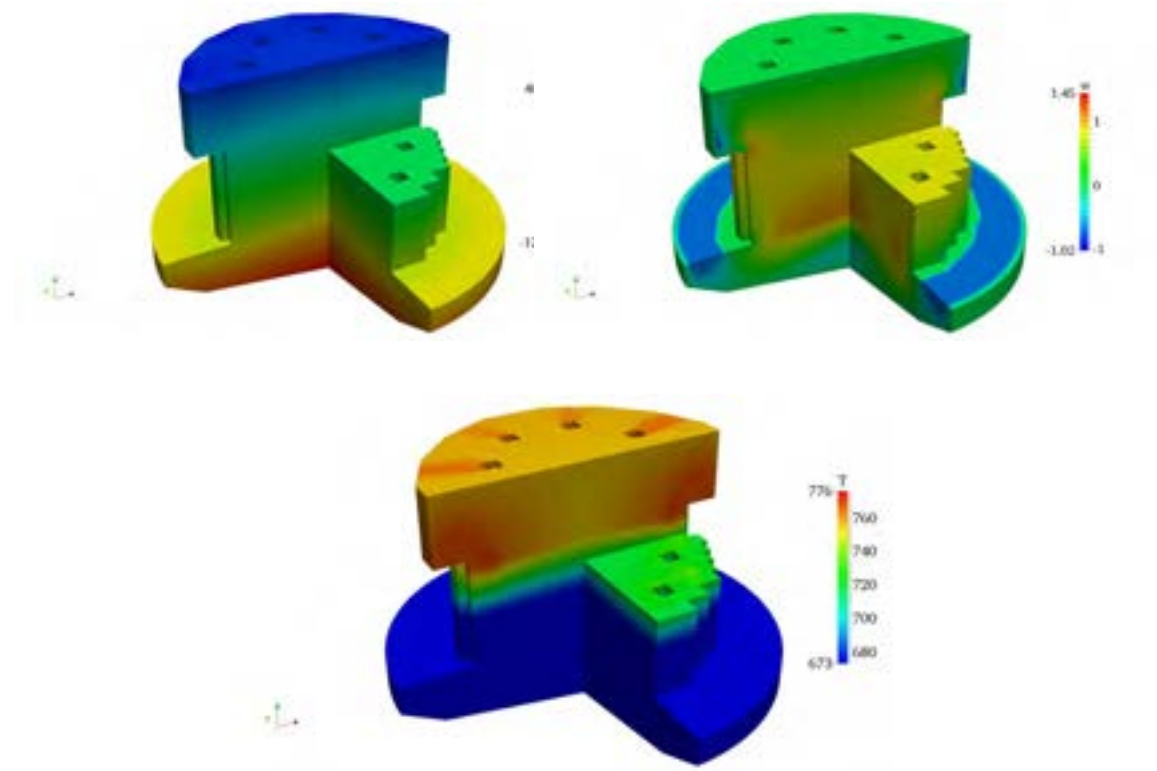
Figure 2.35: FEMLCORE module. Temperature, pressure and velocity field at working conditions.
