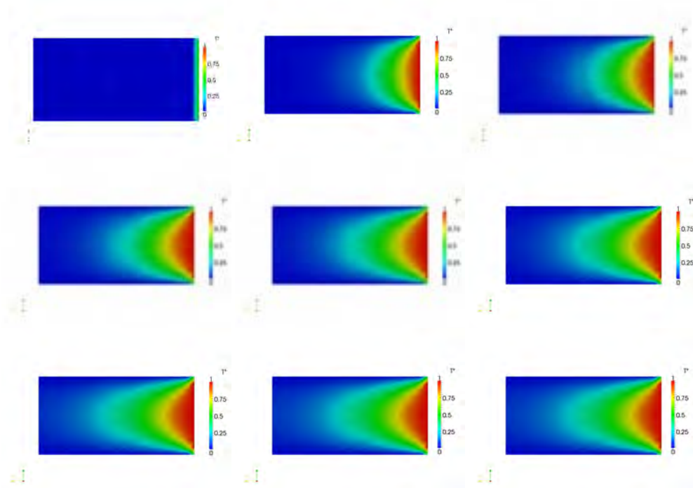
Figure 2.5: Solution evolution over the coupled domain.
