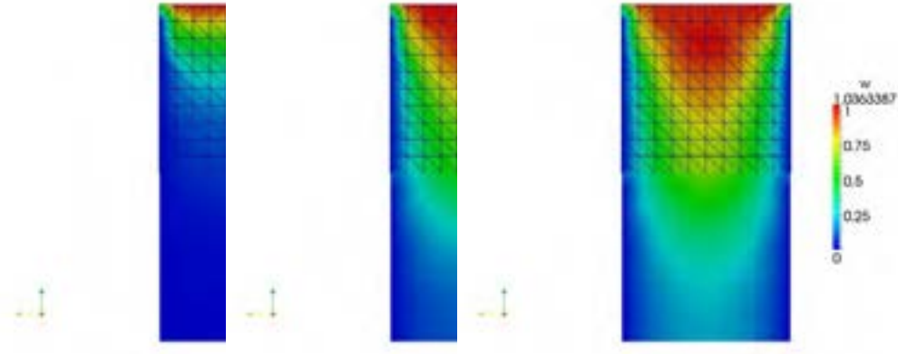
Figure 2.10: Solution evolution over the coupled domain.
