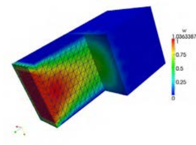
Figure 2.9: Solution over the coupled domain.
