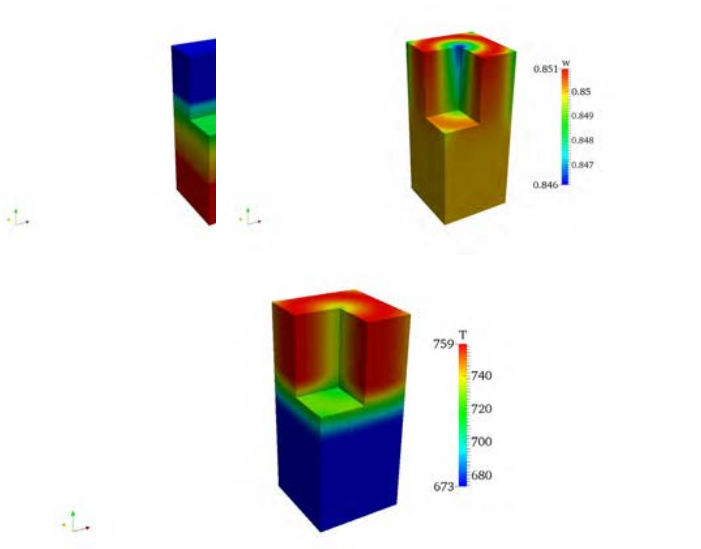
Figure 2.32: Case C. Pressure, velocity and temperature fields. Tests with inlet filtration velocity w = 0.85 \text{ m/s} , variable fluid properties and with all pressure drops.
