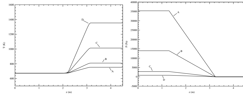
Figure 2.23: Case A. Temperature (left) and pressure (right) profiles along the segment \overline{ST} . Line A: inlet velocity w = 0.85 \text{ m/s} ; Line B: inlet velocity w = 0.5 \text{ m/s} ; Line C: inlet velocity w = 0.2 \text{ m/s} ; Line D: inlet velocity w = 0.1 \text{ m/s} .
