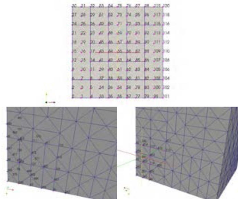
Figure 2.7: Numbering of the same surface in MEDMem mesh (top) and in libMesh as \Omega_1 (left bottom) and as \Omega_2 (right bottom).
