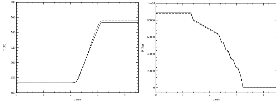
Figure 2.29: Case C. Comparison of temperature (left) and pressure (right) profiles along the line \overline{ST} . Dashed line: simulation with temperature dependent properties, solid line: simulation with constant properties.
