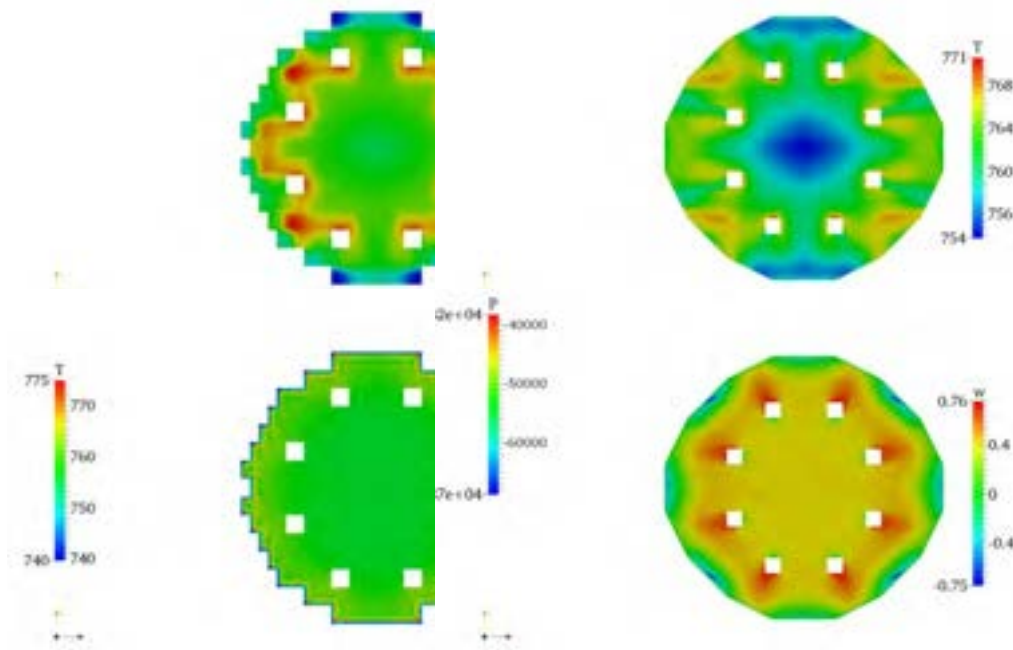
Figure 2.37: FEMLCORE module. Stationary solution of the temperature and velocity fields on sections a and b in the case of operation at nominal power.
