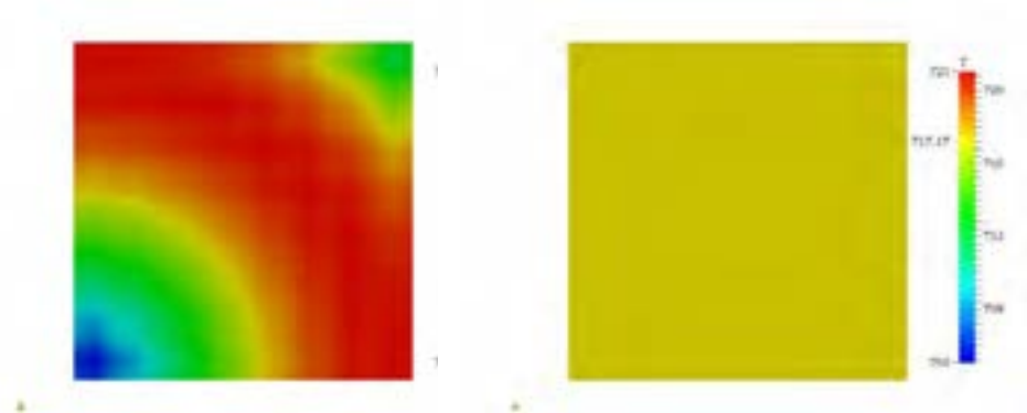
Figure 2.30: Case C. Comparison of temperature distributions on section a . On the left temperature dependent physical property case with q_g = q_g(\mathbf{x}) . On the right temperature constant physical properties case with q_g = \text{const} .
