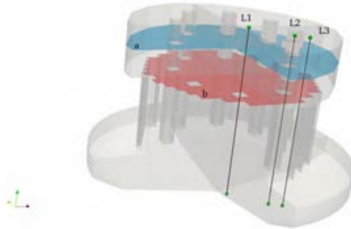
Figure 2.33: FEMLCORE module. Placement of figures and charts. Cross-sectional portion of a at z = 3.9 \text{ m} ; Cross section b at z = 3.244 \text{ m} ; line L1 at x = y = 0.2 \text{ m} ; line L2 at x = y = 1 \text{ m} ; line L3 at x = 1.323 \text{ m} and y = 1.176 \text{ m} .
