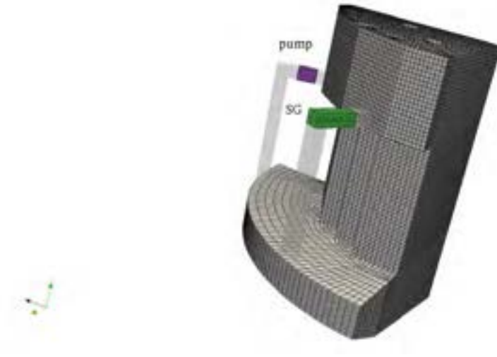
Figure 2.34: LibMesh module. Location of the pump and steam generator in the computational primary loop.
