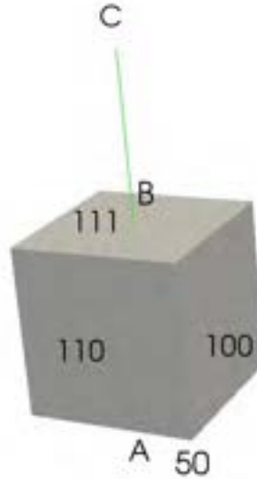
Figure 2.18: Coupling 3D-1D geometry. Domain \Omega_1 \cup \Gamma_2(BCline) .
