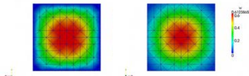
Figure 2.8: Solution over the coupled interface as \Omega_1 (left) and as \Omega_2 (right).
