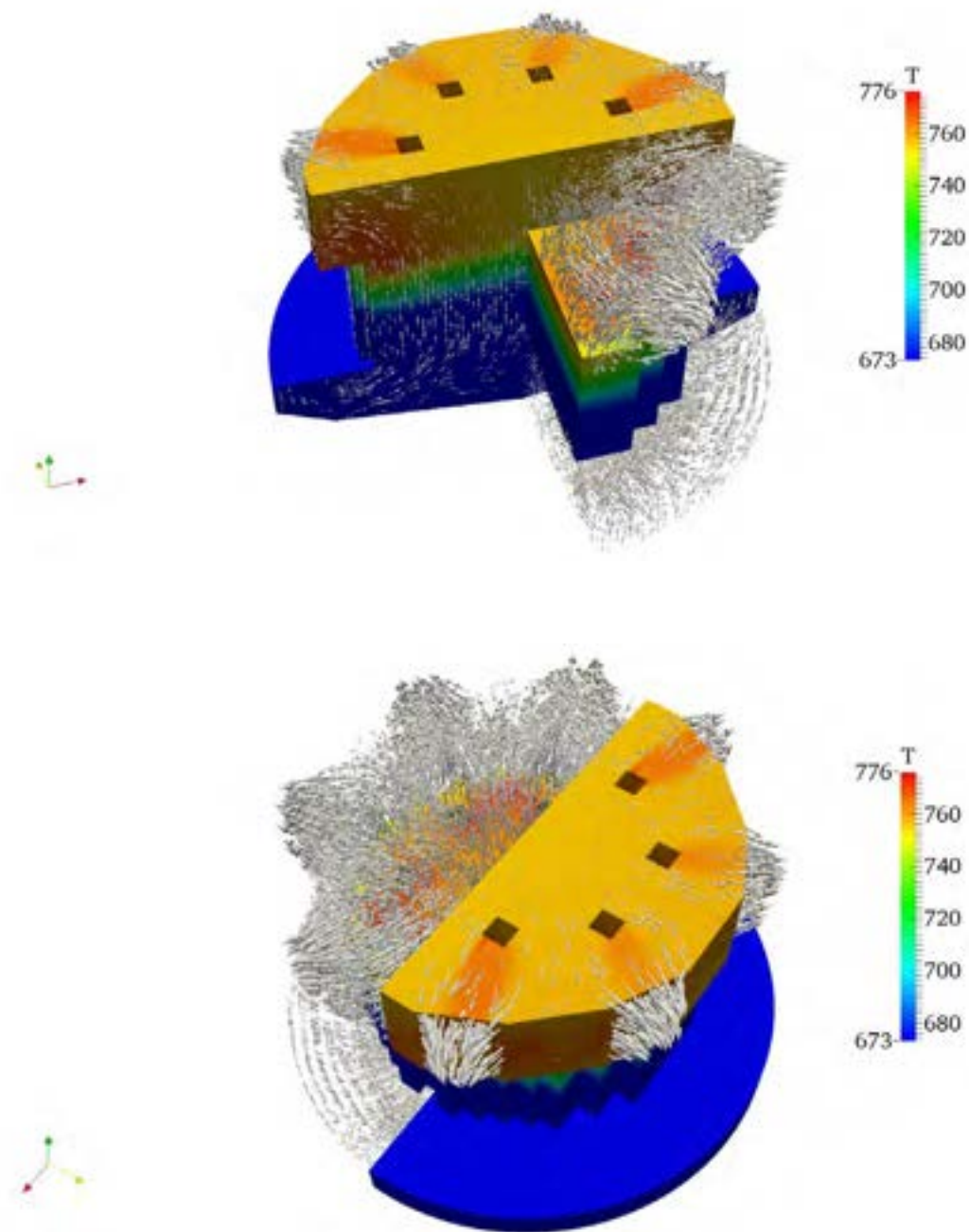
Figure 2.36: FEMLCORE module. Vectorial representation of the velocity and temperature field for the stationary solution at nominal power.
