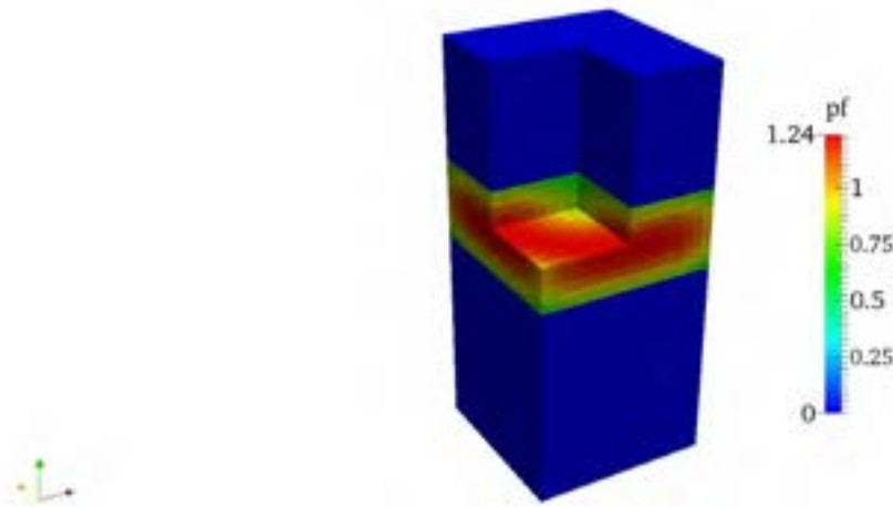
Figure 2.27: Case C. Spatial distribution of the power factor pf .
