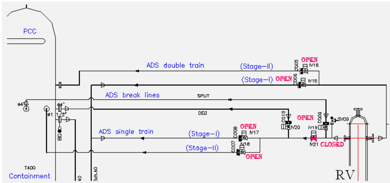
Figure 4.4: SPES3 ADS lines – Flow Sheet – Transient conditions
