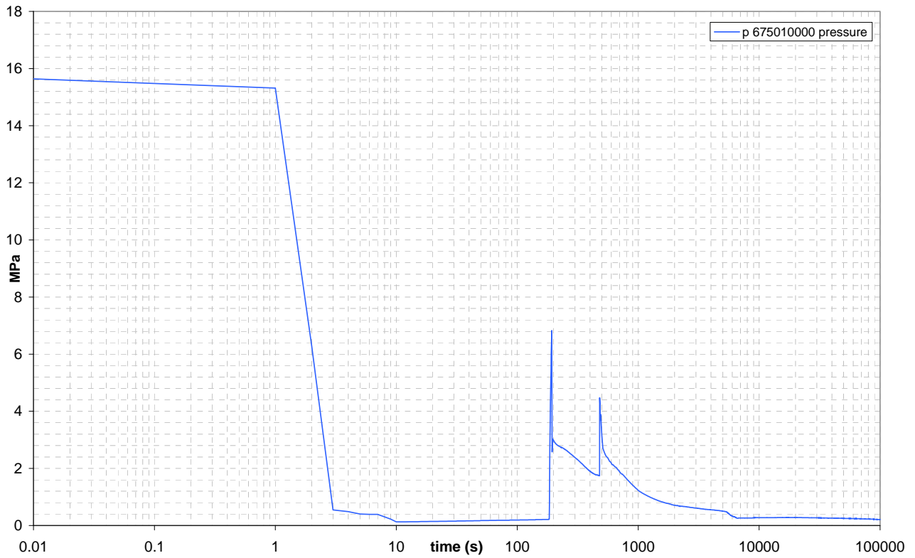
Figure 5.3: DVI DEG BREAK LINE pressure UPSTREAM
