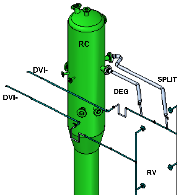
Figure 4.5: SPES3 DVI break line system
