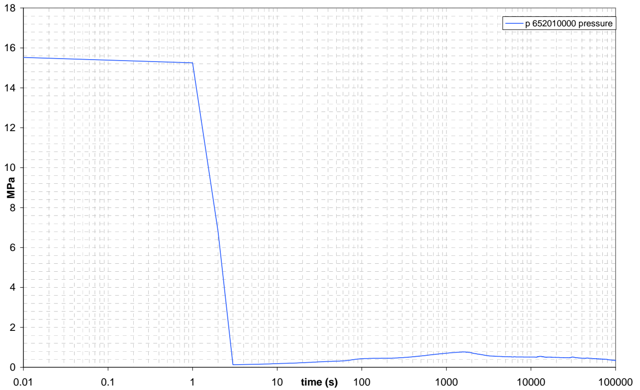
Figure 5.31: EBT DEG BREAK LINE pressure UPSTREAM
