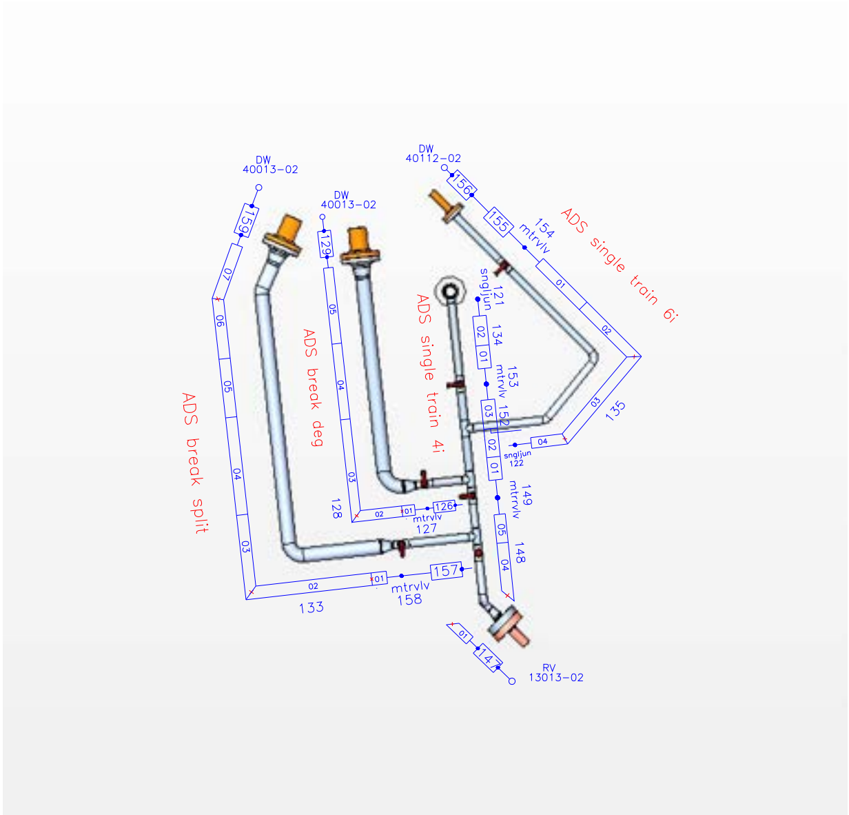
Figure 4.16: SPES3 ADS single train and ADS break line nodalization (top view)
