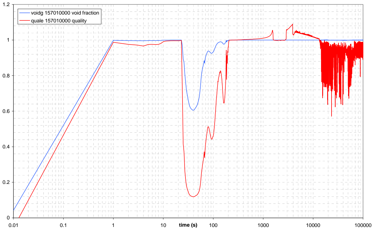
Figure 5.71: ADS ST SPLIT BREAK LINE void fraction and quality UPSTREAM
