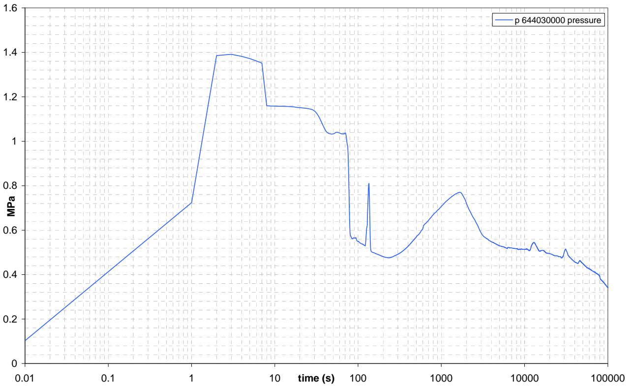
Figure 5.45: EBT SPLIT BREAK LINE pressure DOWNSTREAM
