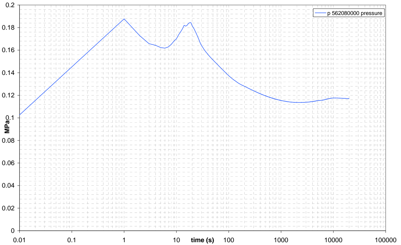
Figure 5.107: FL-B DEG BREAK LINE pressure DOWNSTREAM
