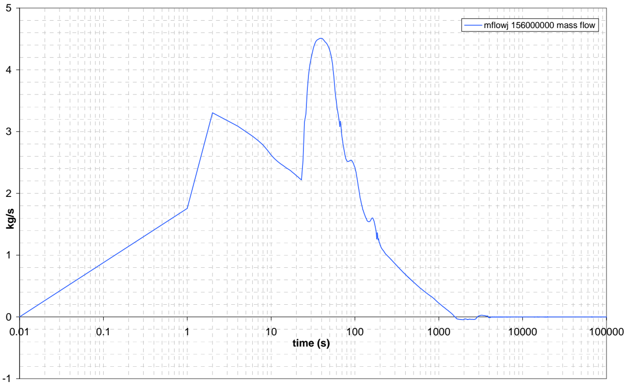
Figure 5.67: ADS ST SPLIT BREAK LINE mass flowrate
