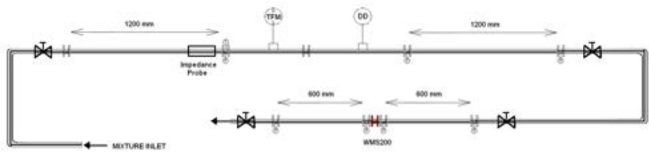
Fig. 7: Schema Test Section
