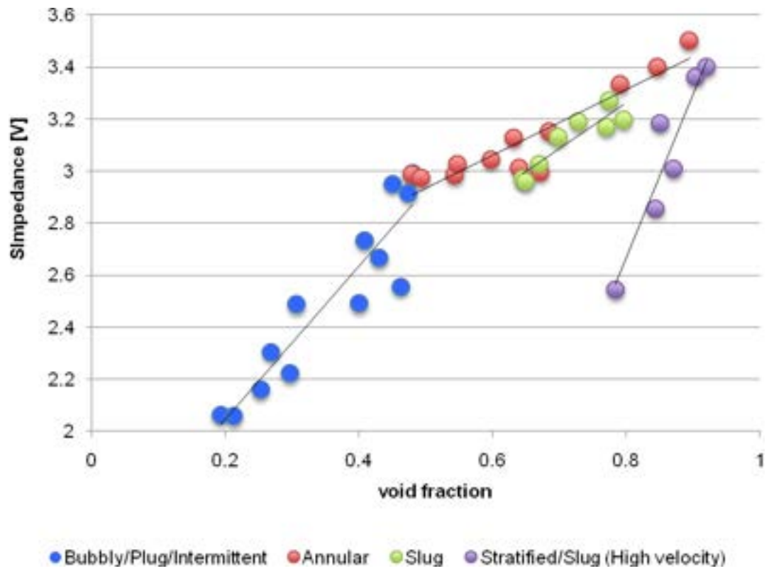
Fig. 34. Impedance [V] vs. Alpha (void fraction)
