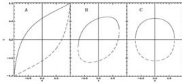
Figura 1.1: eigenvalues of M_1 , \frac{\lambda^+}{c} (full line) and -\frac{\lambda^-}{c} (dashed line) according to f = F_r/(cE_r) .
