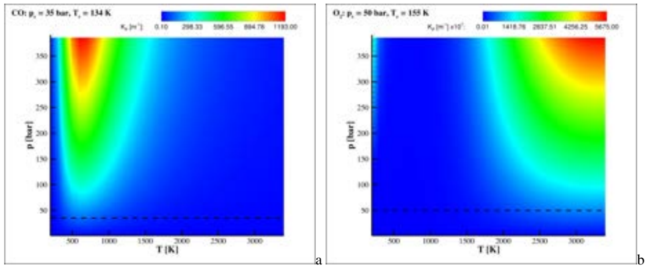
Figura 2.2: a) \text{CO} and b) \text{O}_2 Planck mean absorption coefficient as a function of temperature [K] and pressure [bar].
