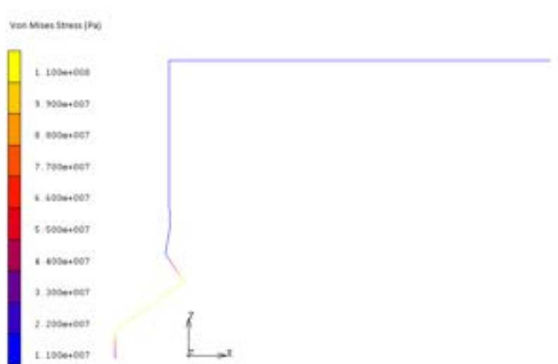
Figure 17 Stress distribution along the hot leg at time t=7.68 sec
