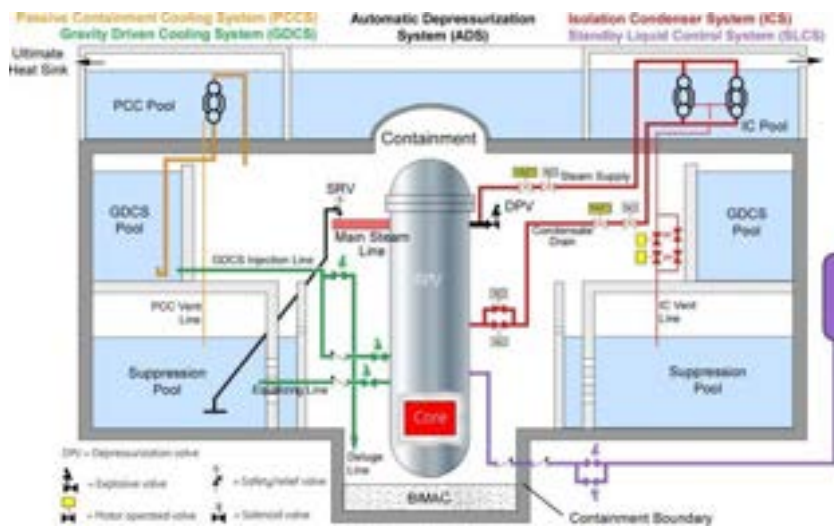
Figure 2 Passive safety systems of the ESBWR
