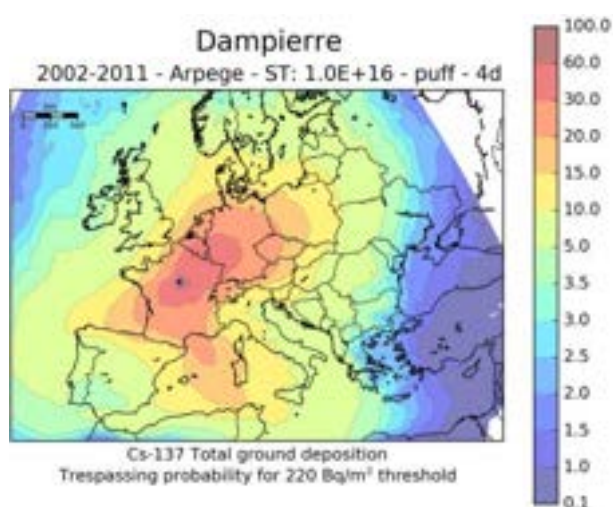
Fig. 19. Trespassing probability (%) for 220 Bq/m², 2002-2011 years, 1E16 Bq, “puff” - 4 days.
