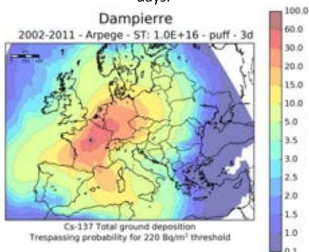
Fig. 21. Trespassing probability (%) for 220 Bq/m², 2002-2011 years, 1E16 Bq, “puff” - 3 days.
