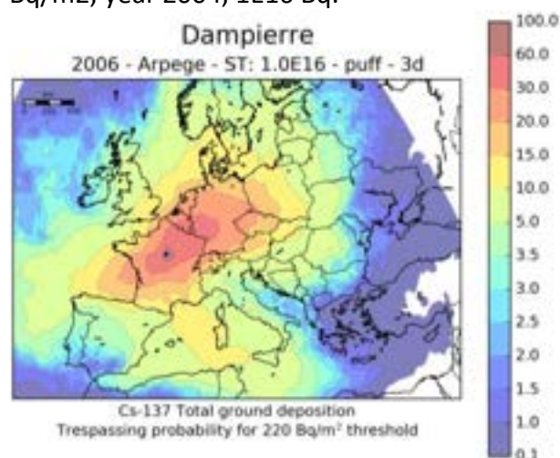
Fig. 11. Trespassing probability (%) for 220 Bq/m 2 , year 2006, 1E16 Bq.
