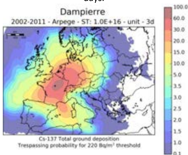
Fig. 22. Trespassing probability (%) for 220 Bq/m², 2002-2011 years, 1E16 Bq, “unit” - 3 days.
