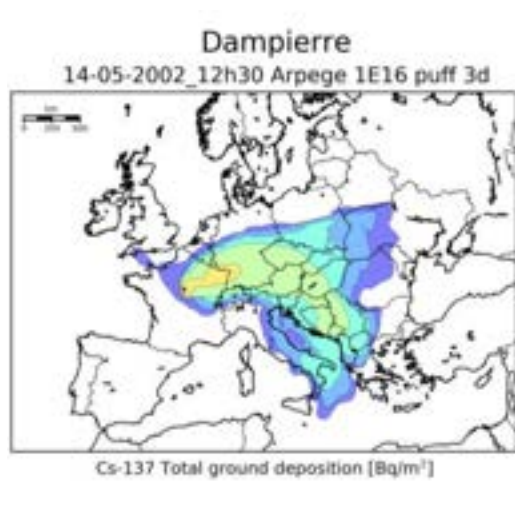
Fig. 26. ^{137}\text{Cs} total ground deposition for an accident starting on 14 May 2002, 3 days.
