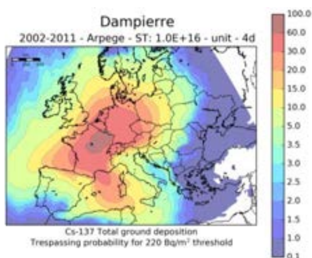
Fig. 20. Trespassing probability (%) for 220 Bq/m², 2002-2011 years, 1E16 Bq, “unit” - 4 days.
