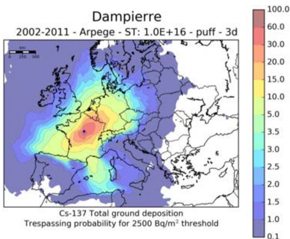
Fig. 6. Trespassing probability (%) for 2500 Bq/m 2 , 2002-2011 years, 1E16 Bq.
