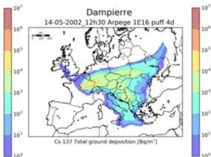
Fig. 27. ^{137}\text{Cs} total ground deposition for an accident starting on 14 May 2002, 4 days.
