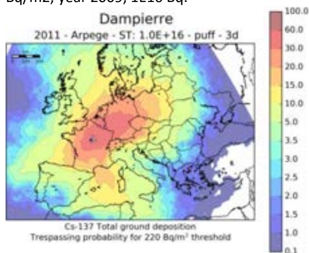
Fig. 16. Trespassing probability (%) for 220 Bq/m 2 , year 2011, 1E16 Bq.
