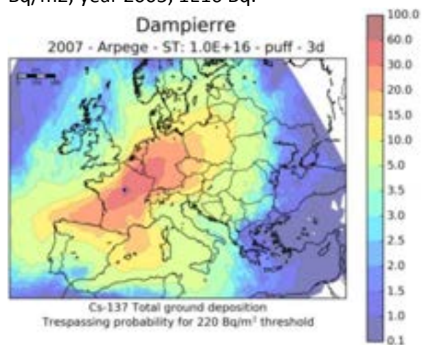
Fig. 12. Trespassing probability (%) for 220 Bq/m 2 , year 2007, 1E16 Bq.
