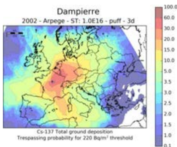
Fig. 7. Trespassing probability (%) for 220 Bq/m 2 , year 2002, 1E16 Bq.
