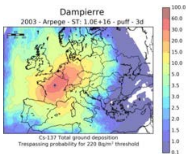
Fig. 8. Trespassing probability (%) for 220 Bq/m 2 , year 2003, 1E16 Bq.
