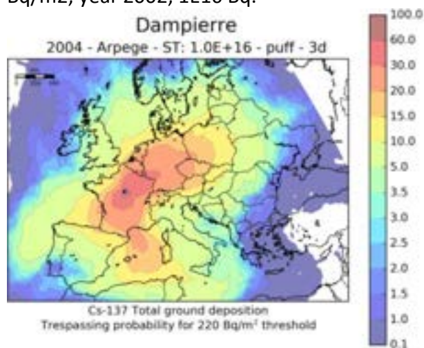
Fig. 9. Trespassing probability (%) for 220 Bq/m 2 , year 2004, 1E16 Bq.
