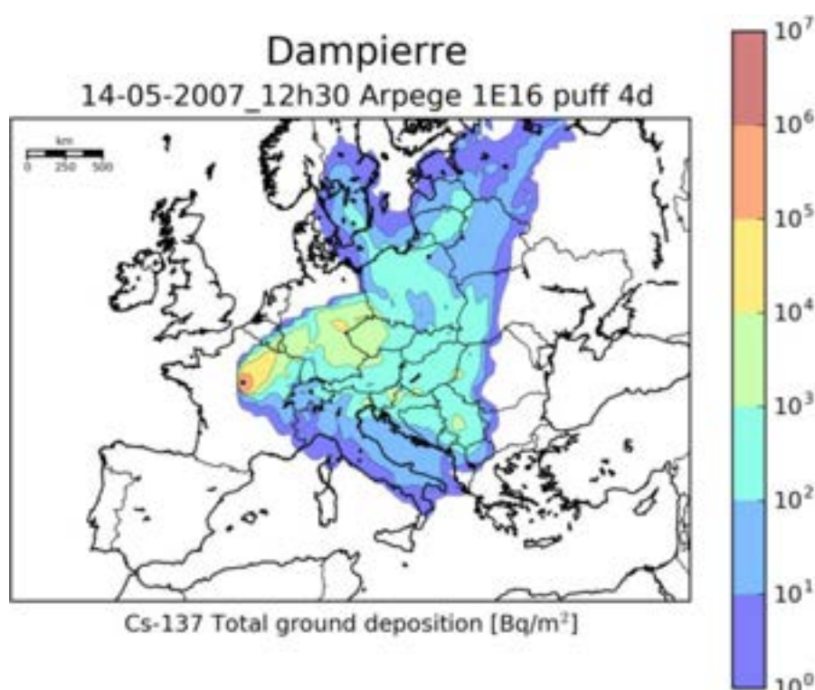
Fig. 28. ^{137}\text{Cs} total ground deposition for an accident starting on 14 May 2007.
