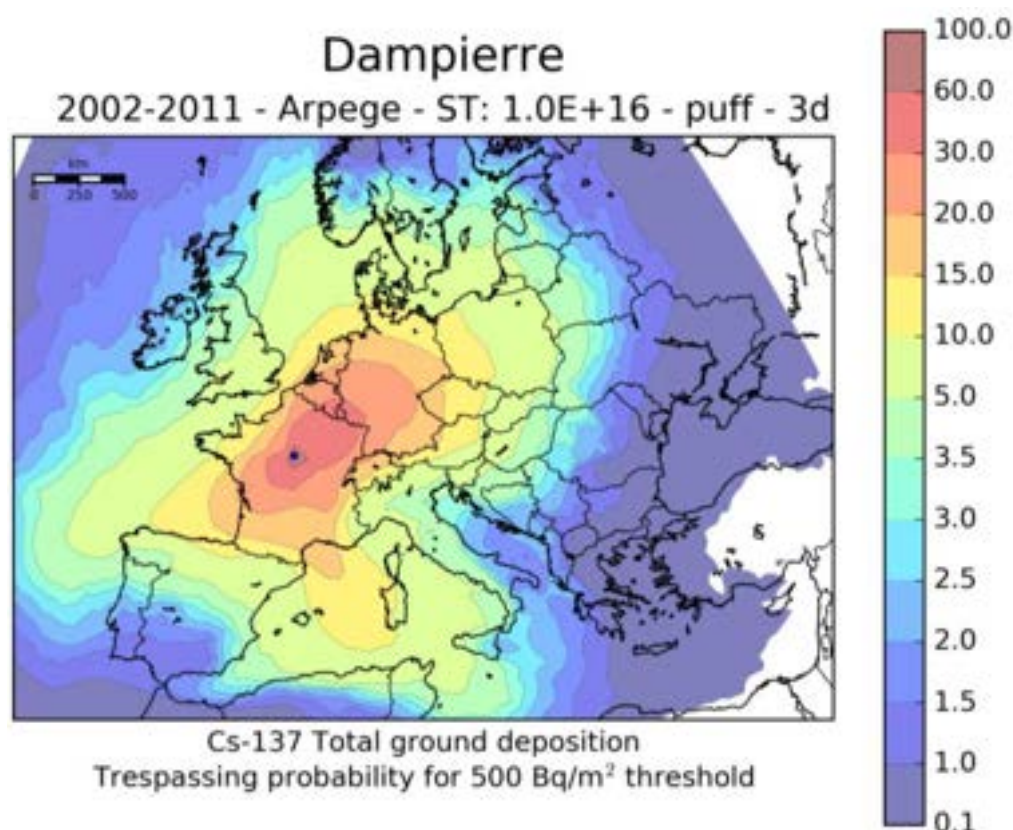
Fig. 5. Trespassing probability (%) for 500 Bq/m 2 , 2002-2011 years, 1E16 Bq.
