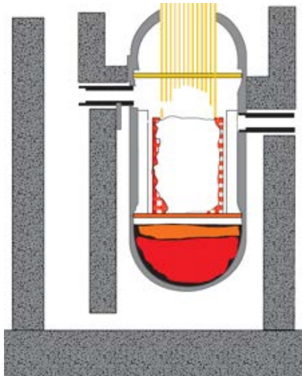
Figure 3: IVCR - Configuration of the vessel with a melt pool in the bottom head and the cooling of the outer wall of the vessel with two-phase flow along the vessel [10].
