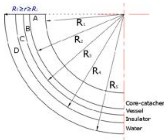
Figure 6: Analytical model with thermal insulator (instead of adiabatic boundary condition)
