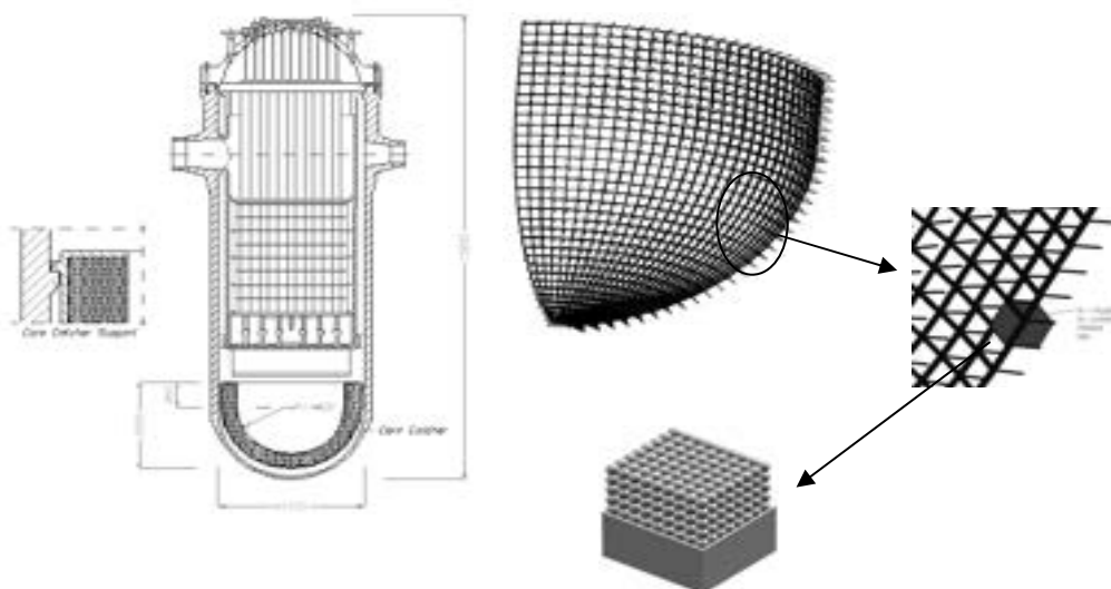
Figure 5: Overview of the proposed internal core catcher (left figure) and of the frame structure made of SiC-SiC ceramic matrix composite with box filled by alumina pebble bed (right figure) for a RPV of 1000 MWe PWR [11].
