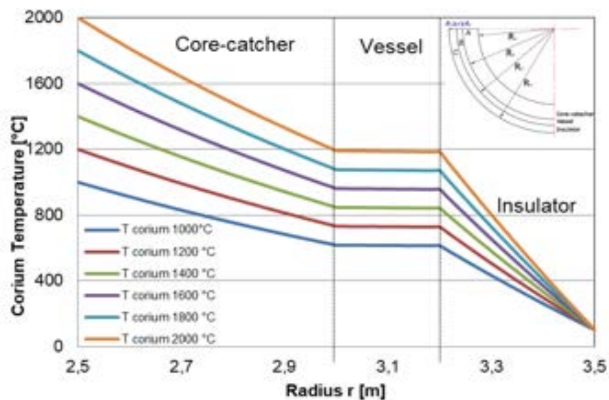
Figure 9: Radial temperature variation in the hemispherical bottom head for T(R_4) = 100^{\circ}\text{C} .
