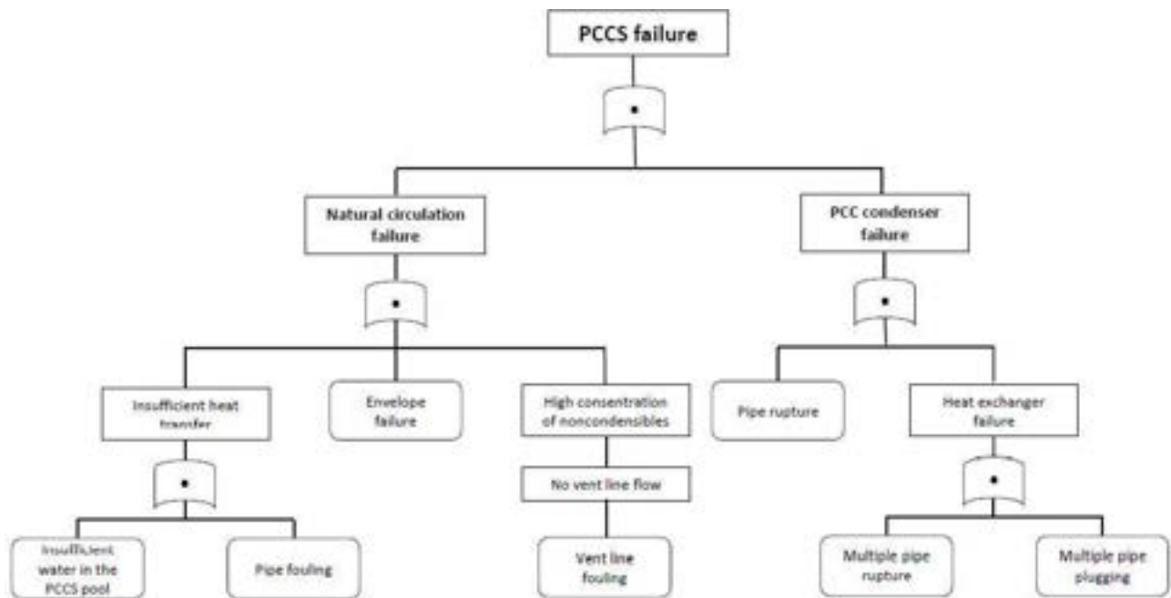
Figure 2: Fault tree for PCCS
