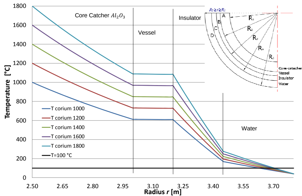
Figure 7: Radial temperature trend in the hemispherical bottom head.
