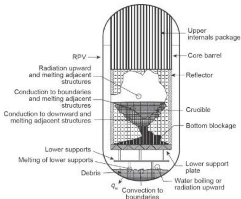
Figure 4: Core meltdown and melt-relocation (to the bottom head) scenarios as during TMI-2 accident: material configuration and heat transfer processes at an intermediate state of melt progression, after initial major relocation and before final steady state [13].
