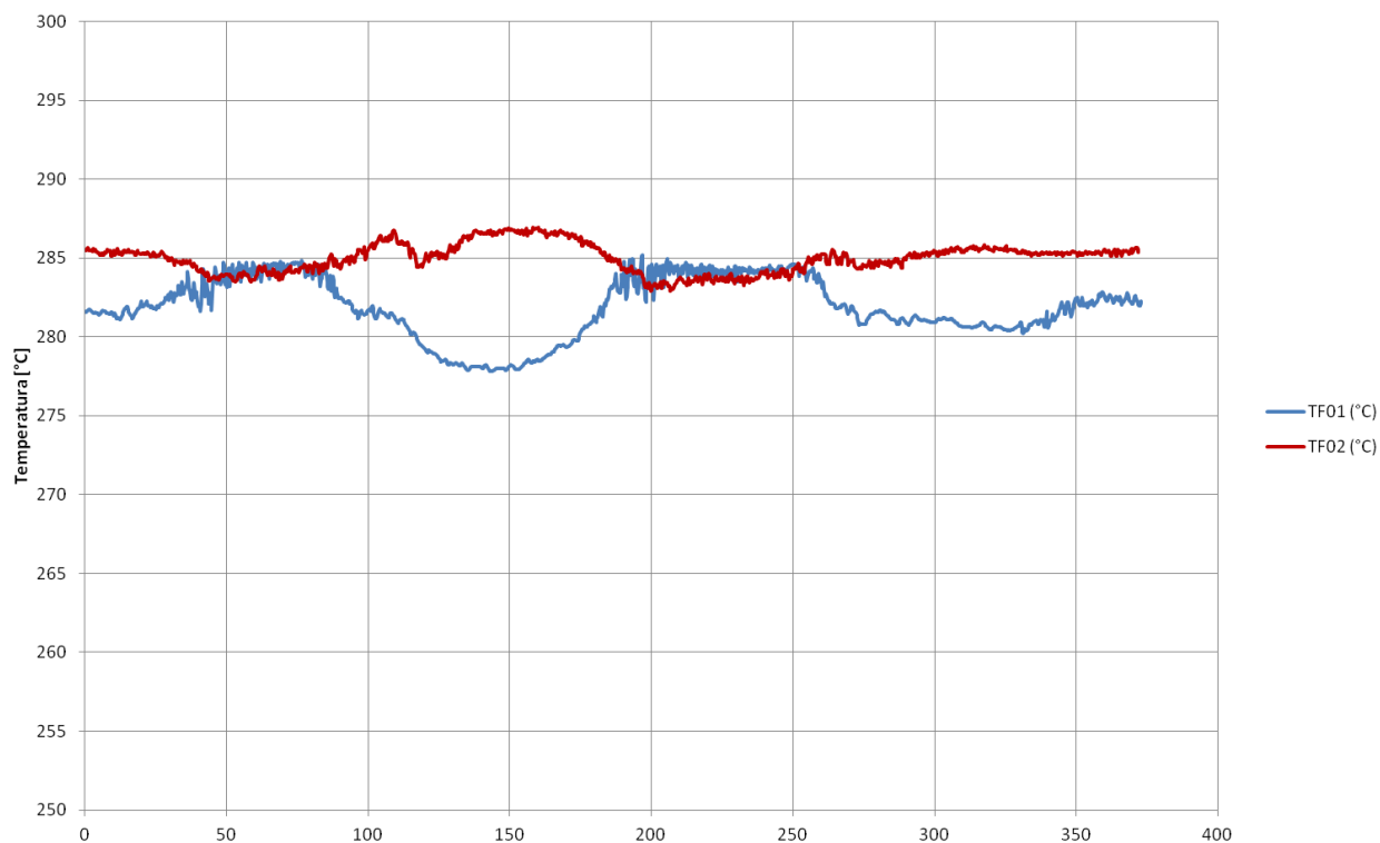
Temperature in/out vs. tempo - Test 2017
