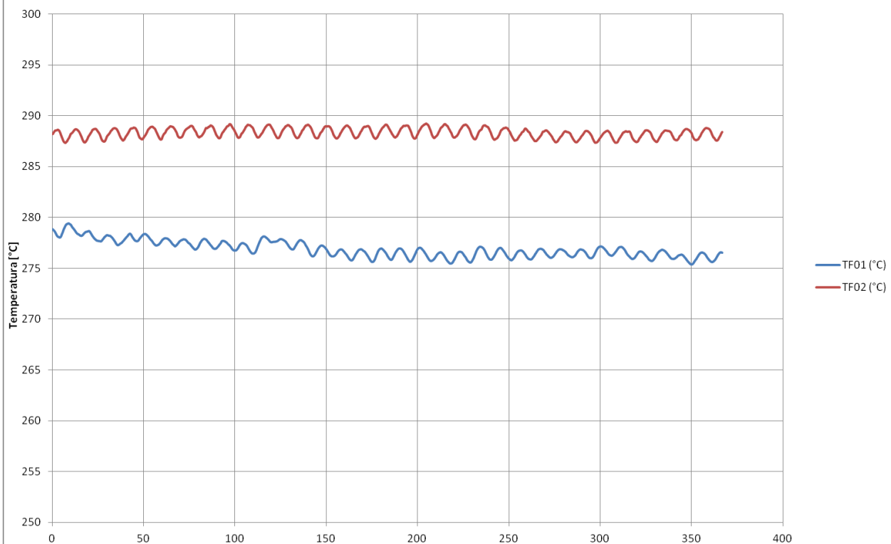
Temperature in/out vs. tempo - Test 2015
