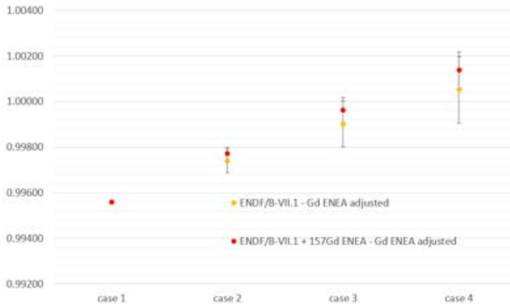
Figure 16) Comparison of standard ENDF/B-VII.1 and ENDF/B-VII.1 + ^{157}\text{Gd} ENEA: ENEA adjusted concentration
