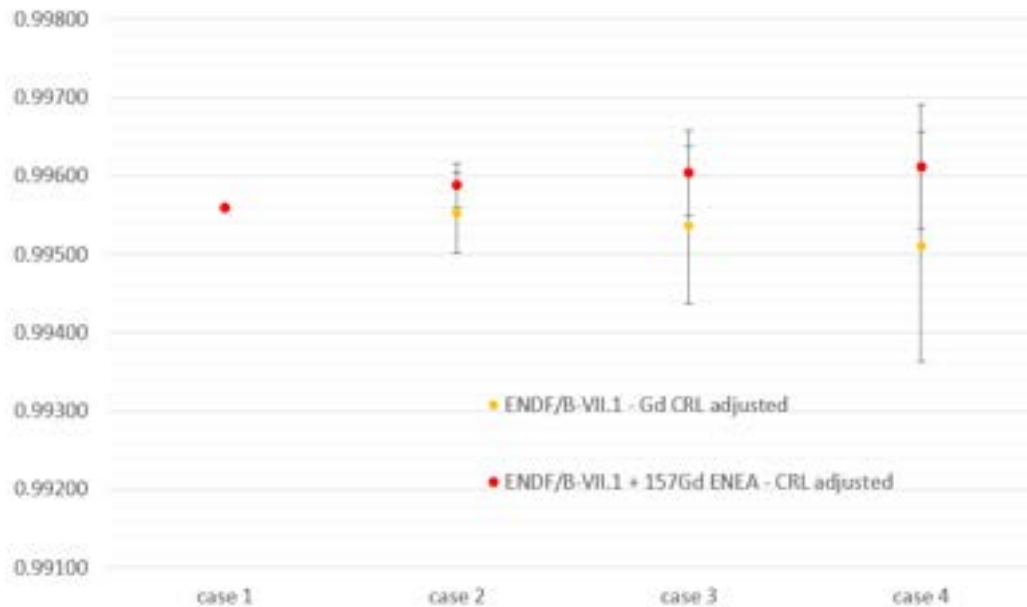
Figure 15) Comparison of standard ENDF/B-VII.1 and ENDF/B-VII.1 + ^{157}\text{Gd} ENEA: CRL adjusted concentration
