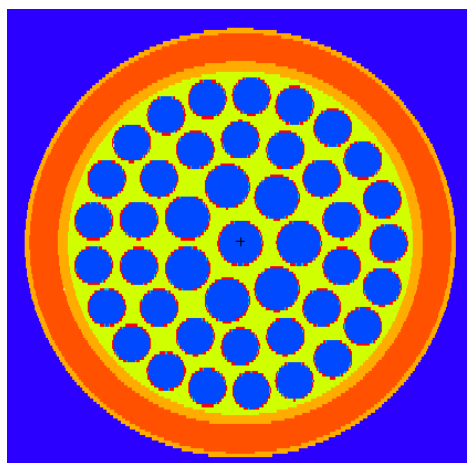
Figure 6) ZED-2 fuel bundle (pins and air inside)
