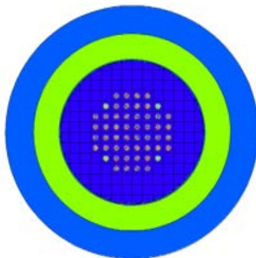
Figure 4) ZED-2 core: MCNP6.1 model (horiz.)
