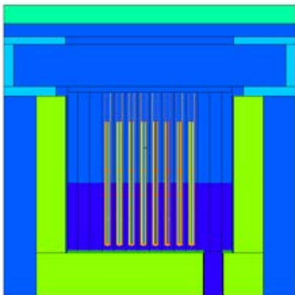
Figure 3) ZED-2 reactor: MCNP6.1 model (vertical)
