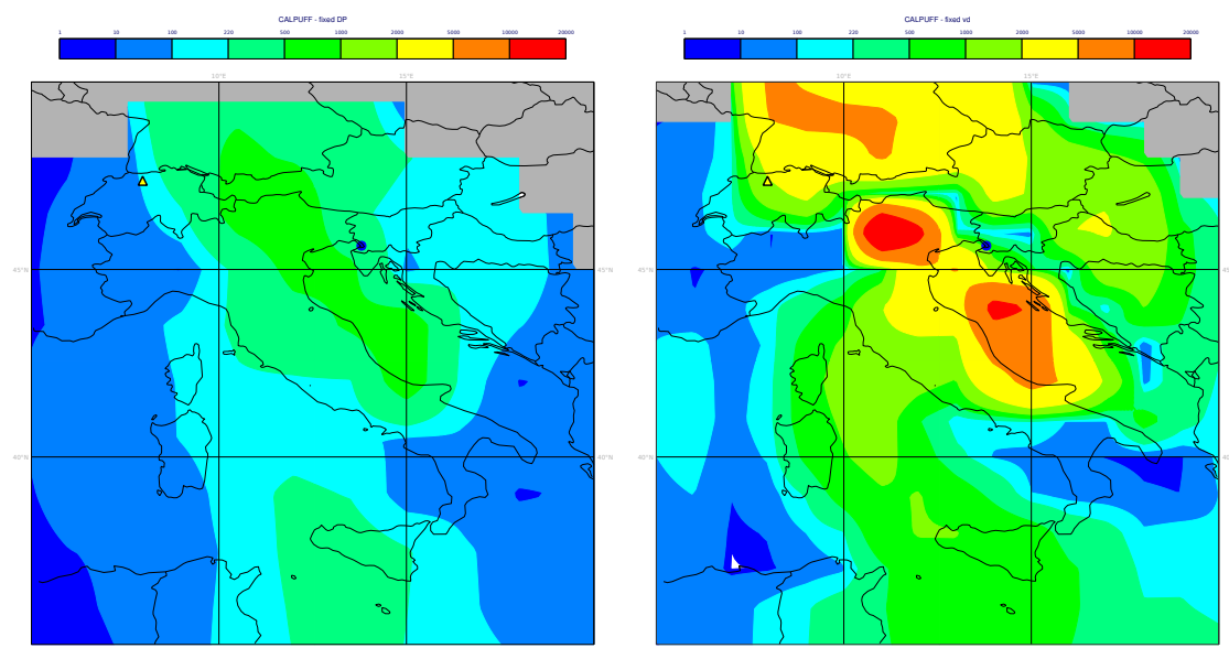
Figure 3.1: Comparison of CALPUFF final deposited Cs-137 in Bq/m 2 with different dry deposition models: fixed particle diameter (left) and fixed deposition velocity (right). ▲: Gösgen NPP, ●: Trieste.
