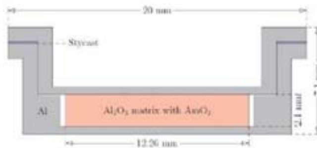
Figure 4. IRMM \text{AmO}_2 samples for the AMSTRAMGRAM program.
