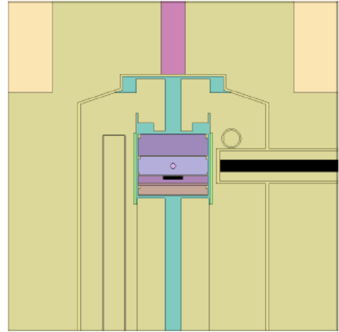
(b) - Serpent model
