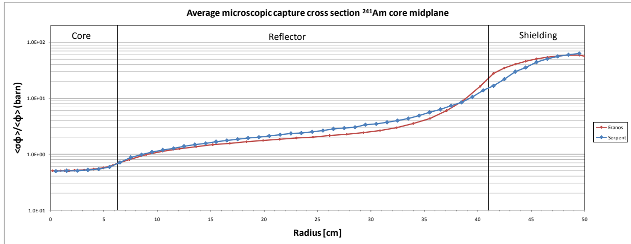
Figure3. \text{Am}^{241} microscopic capture cross section.
