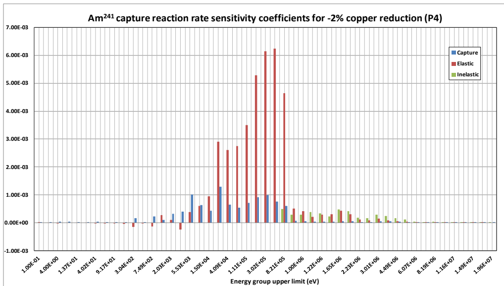
Figure 10: Am 241 (a) and Np 237 (b) capture reaction rate sensitivity coefficients in position P4.
