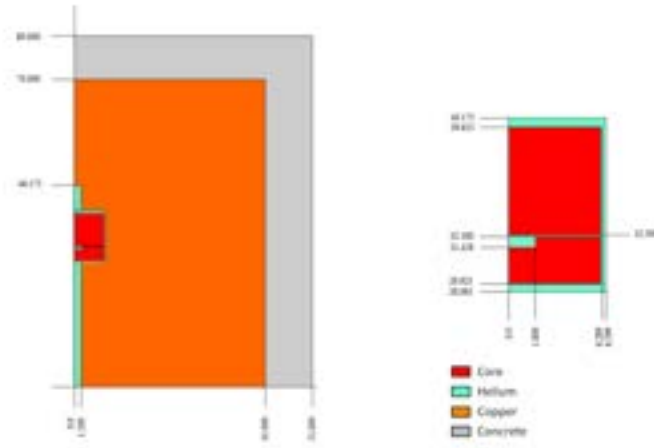
(a) - RZ ERANOS model
