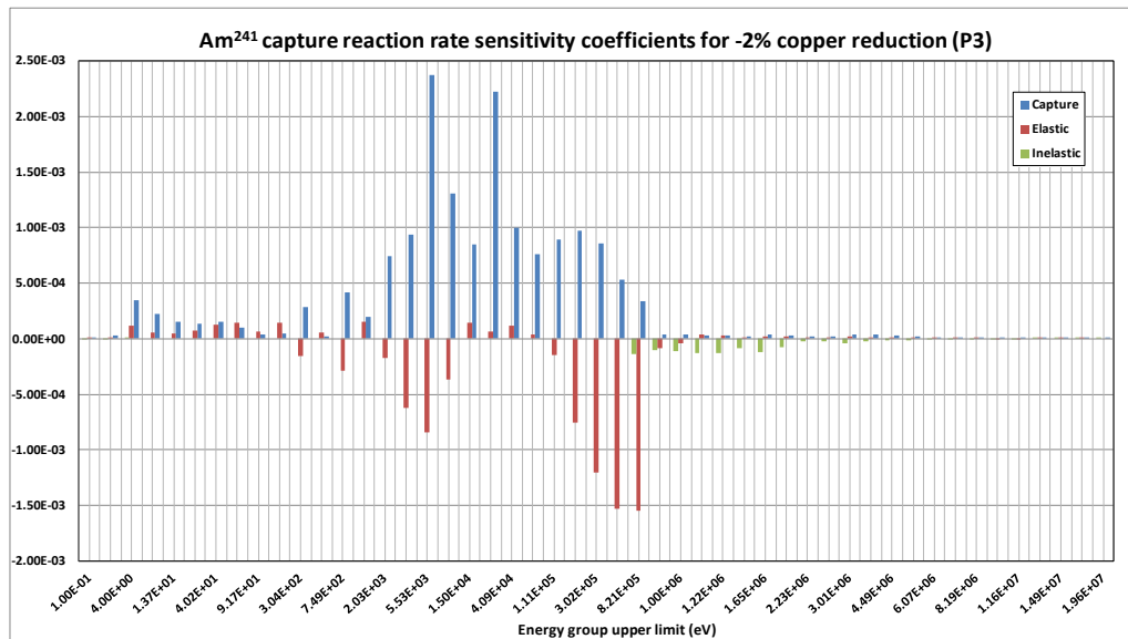
Figure 9: Am 241 (a) and Np 237 (b) capture reaction rate sensitivity coefficients in position P3.
