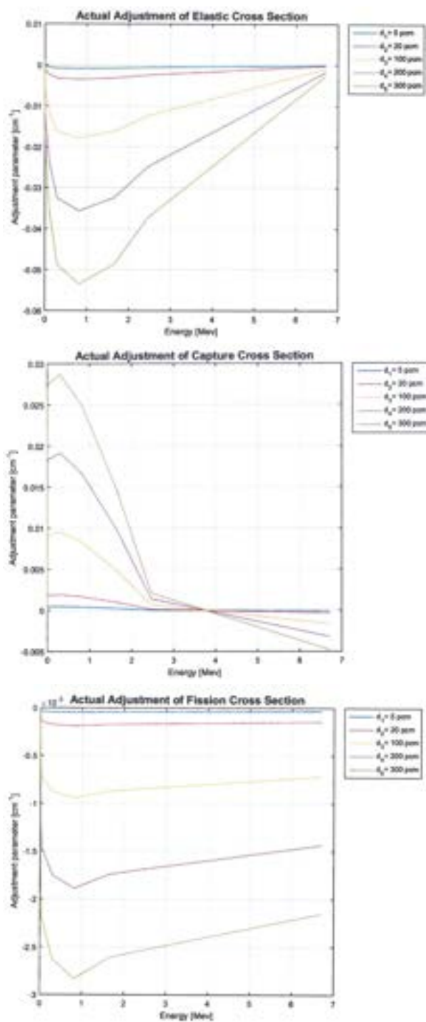
Figure 6. Adjustments for the elastic scattering, capture and fission cross sections of U-235.
