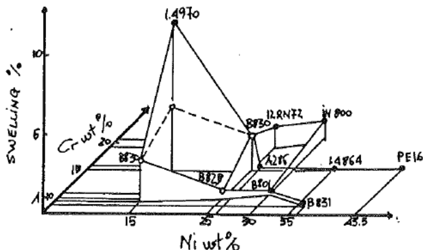
Fig. 3 Swelling ratio as function of Ni and Cr contents [2]
