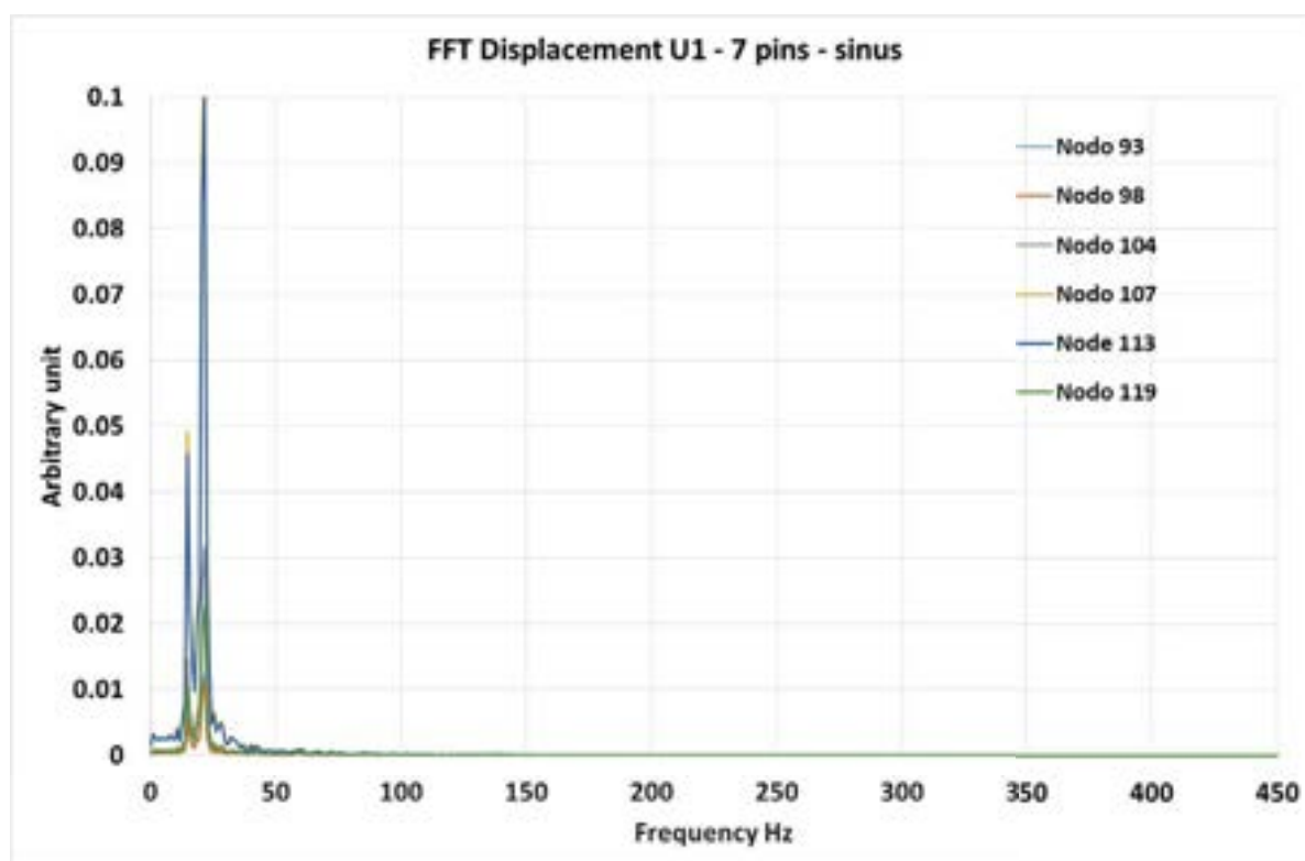
Figure 37. Fourier analysis of the displacement, direction1 .
