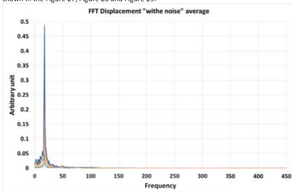
Figure 27. Fourier analysis of the displacement.
