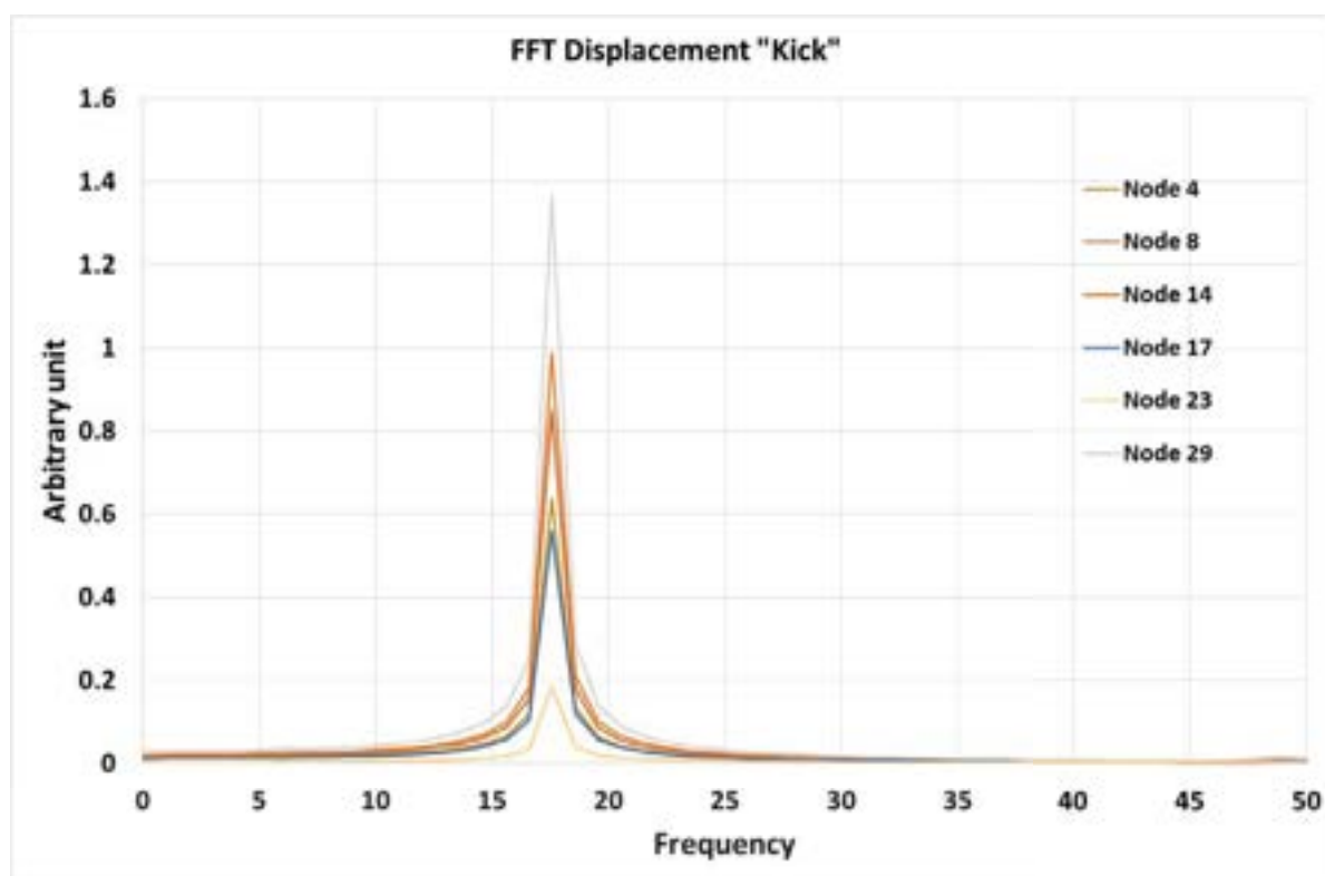
Figure 25. Fourier analysis of the displacement, enlarged scale.
