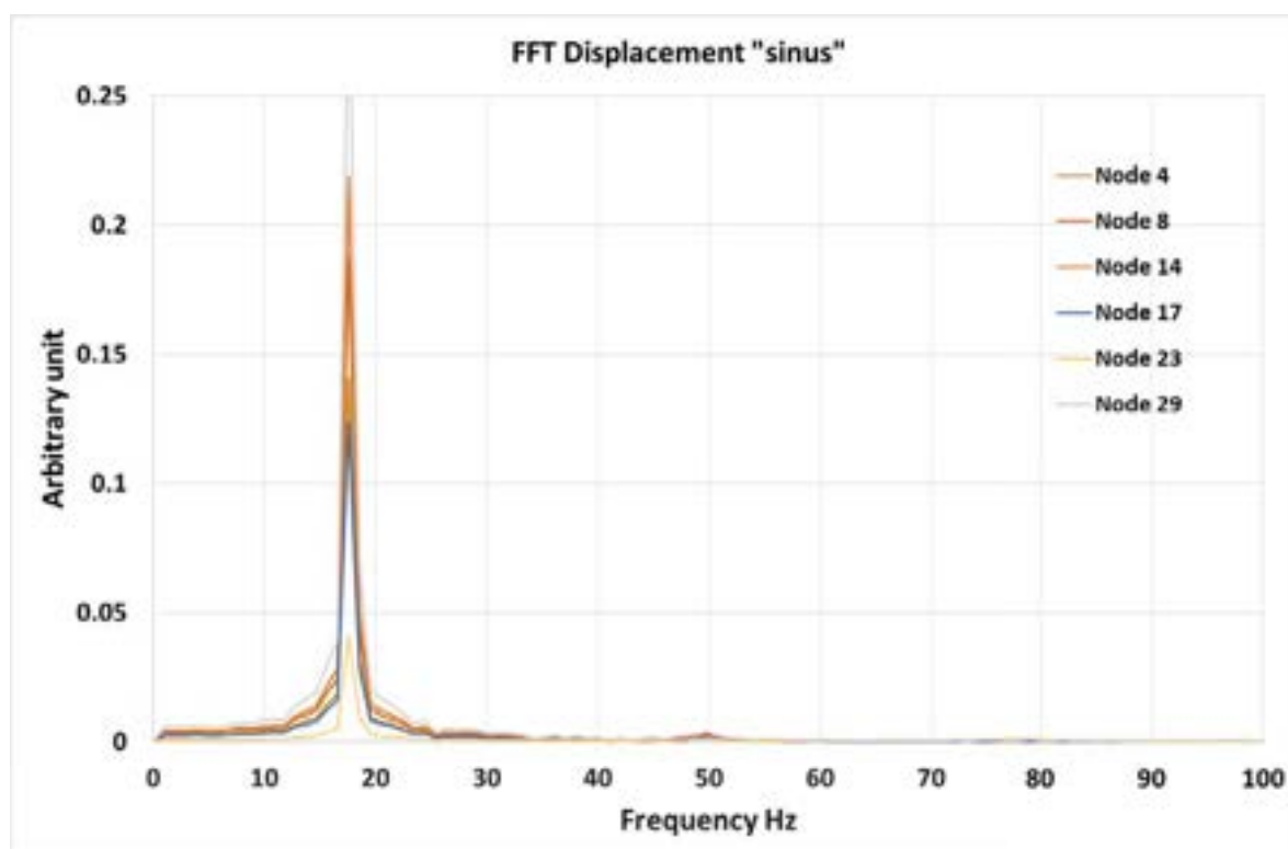
Figure 31. Fourier analysis of the displacement, enlarged scale.
