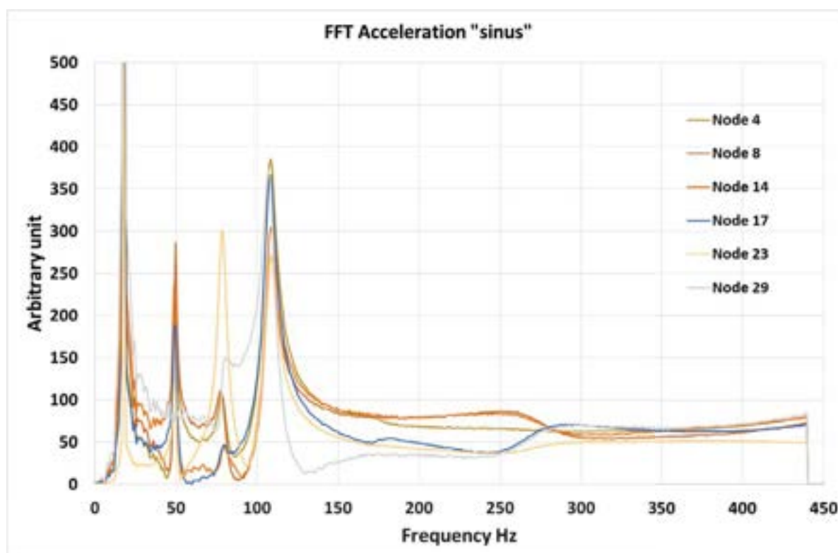
Figure 32. Fourier analysis of the acceleration
