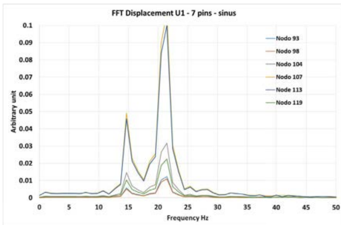
Figure 38. Fourier analysis of the displacement, direction 2, enlarged scale.
