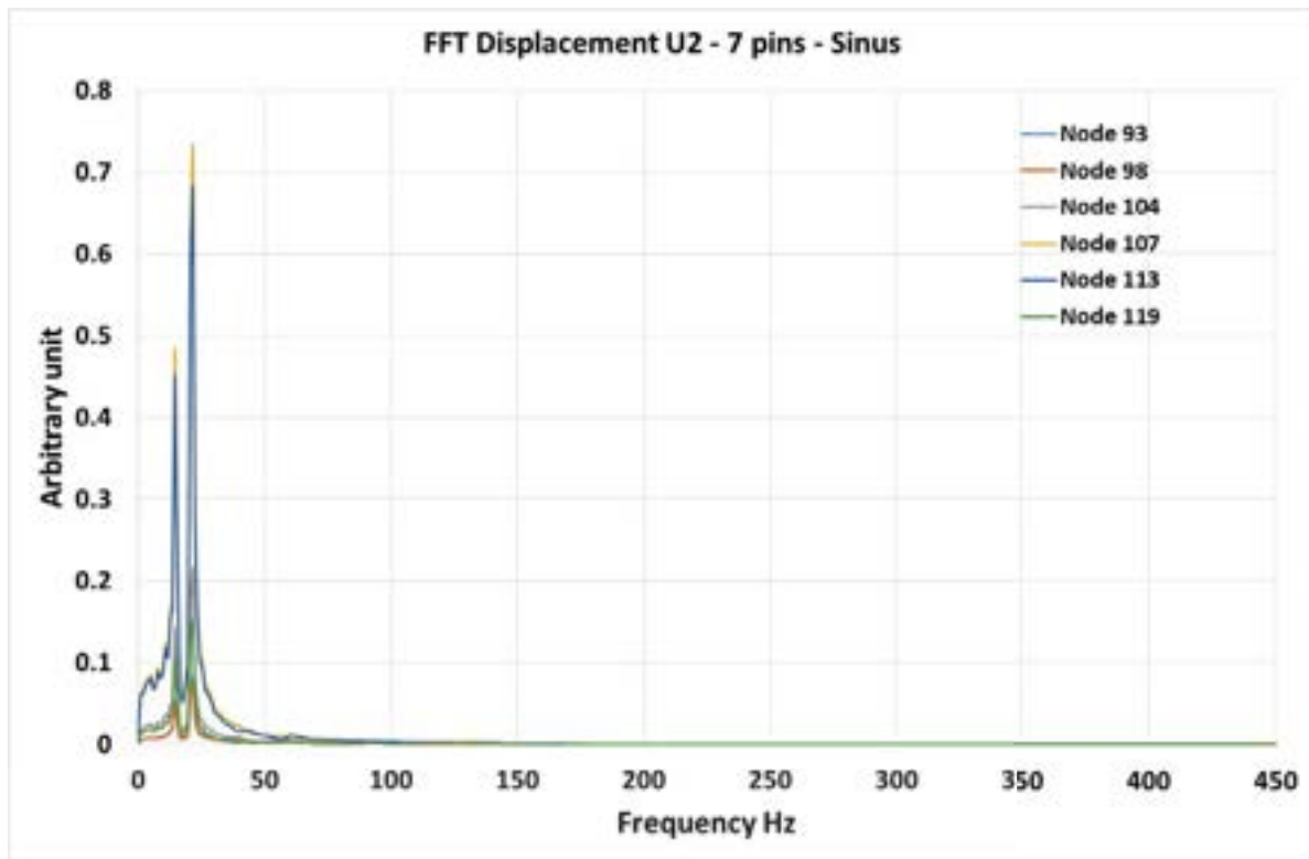
Figure 35. Fourier analysis of the displacement, direction 2.
