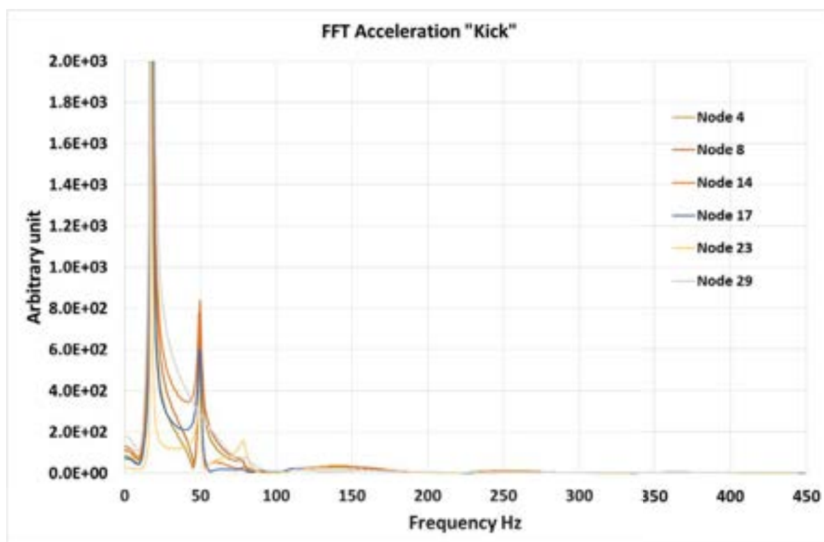
Figure 26. Fourier analysis of the acceleration.
