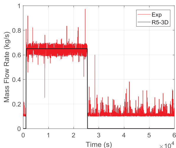
Fig. 2.13 – Feed-water mass flow rate
