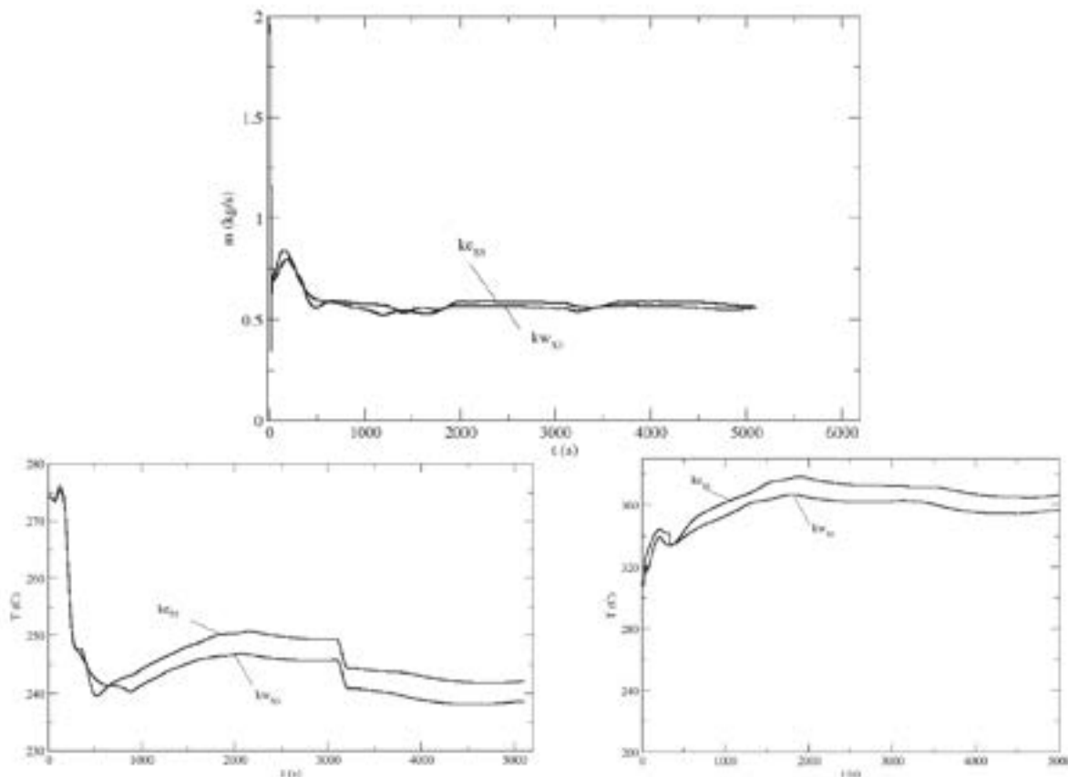
Fig. 4.21 - Mass flow rate (top) and temperature (bottom) at the reference points S3 and S4 for k-\omega ( k\omega ) and k-\epsilon ( k\epsilon ) turbulence models.
