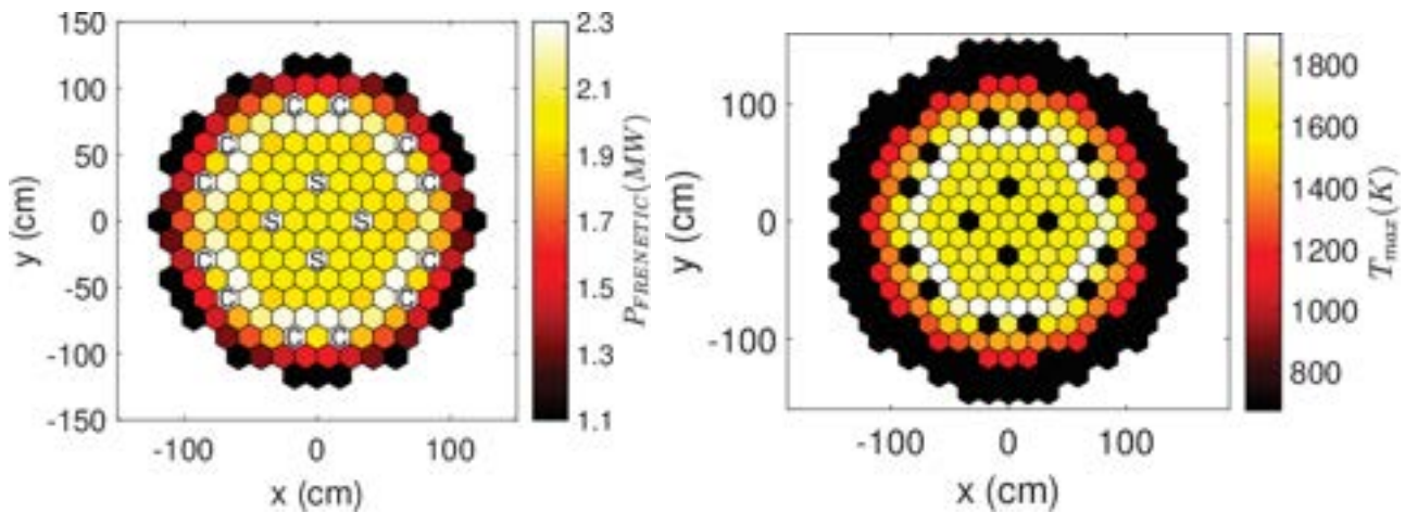
Fig. 5.22 – Radial power (left) and peak fuel temperature (right) distribution computed in the coupled FRENETIC simulations.
