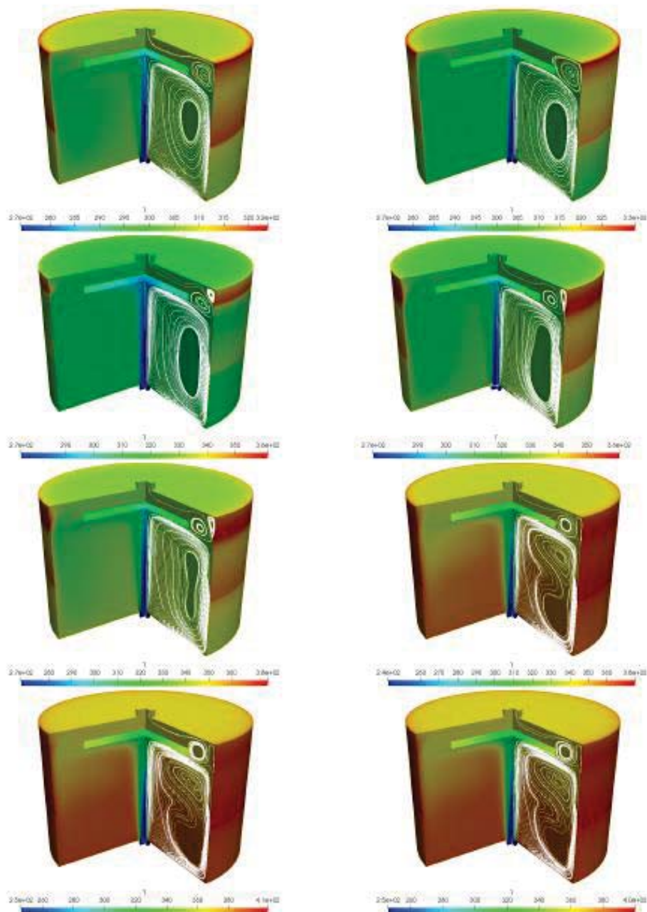
Fig. 4.19 - Temperature and streamline profiles over the 3D test component at time t=0, 4, 20, 80, 180, 580, 1780 and 2780 s by using two-equation \kappa-\omega turbulence model in OpenFoam.
