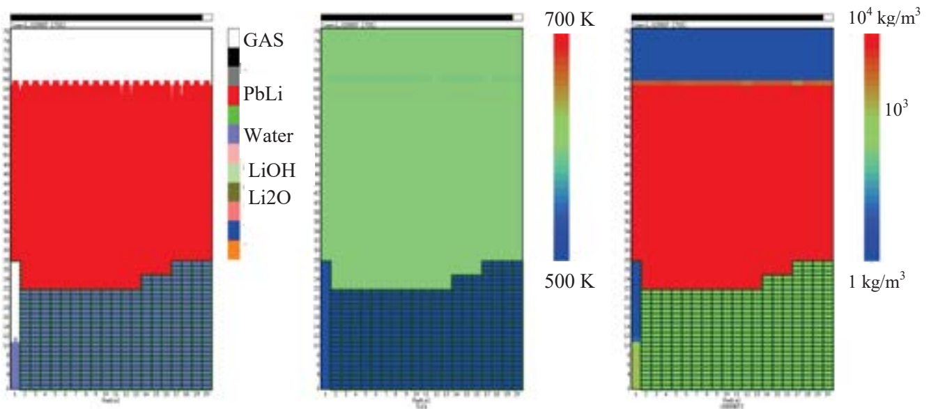
Fig. 7.14 – Time = 1.03 s (0.03 s after start of injection) - Fluids typology (LEFT), PbLi temperature (CENTER) and Fluids density (RIGHT)
