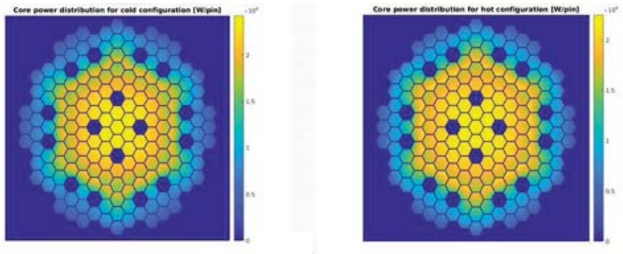
Fig. 5.3 – Serpent radial power map at mid-height in the core at cold condition ( T=673K ), associated to k_{eff}=1.01027\pm3pcm (left); Serpent radial power map at hot condition ( T=1073K ), associated to k_{eff}=1.00772\pm3pcm (right).
