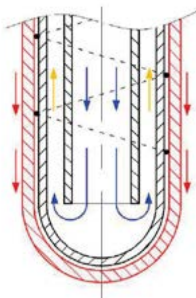
Fig. 2.5 – HX bayonet tube
