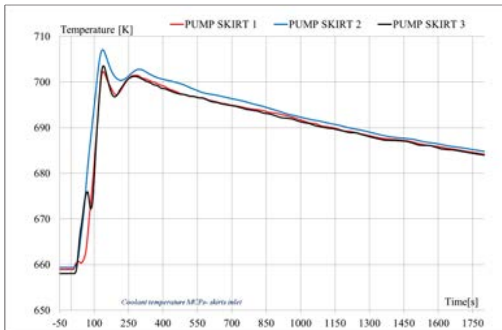
Fig. 3.19 – Primary pumps inlet temperatures
