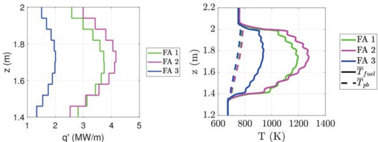
Fig. 5.21 – Linear power calculated by FRENETIC for three selected FAs (left) and axial temperature profiles for fuel and coolant in the same FAs (right)
