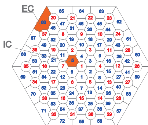
Fig. 2.11 – Nodalization scheme: FPS
