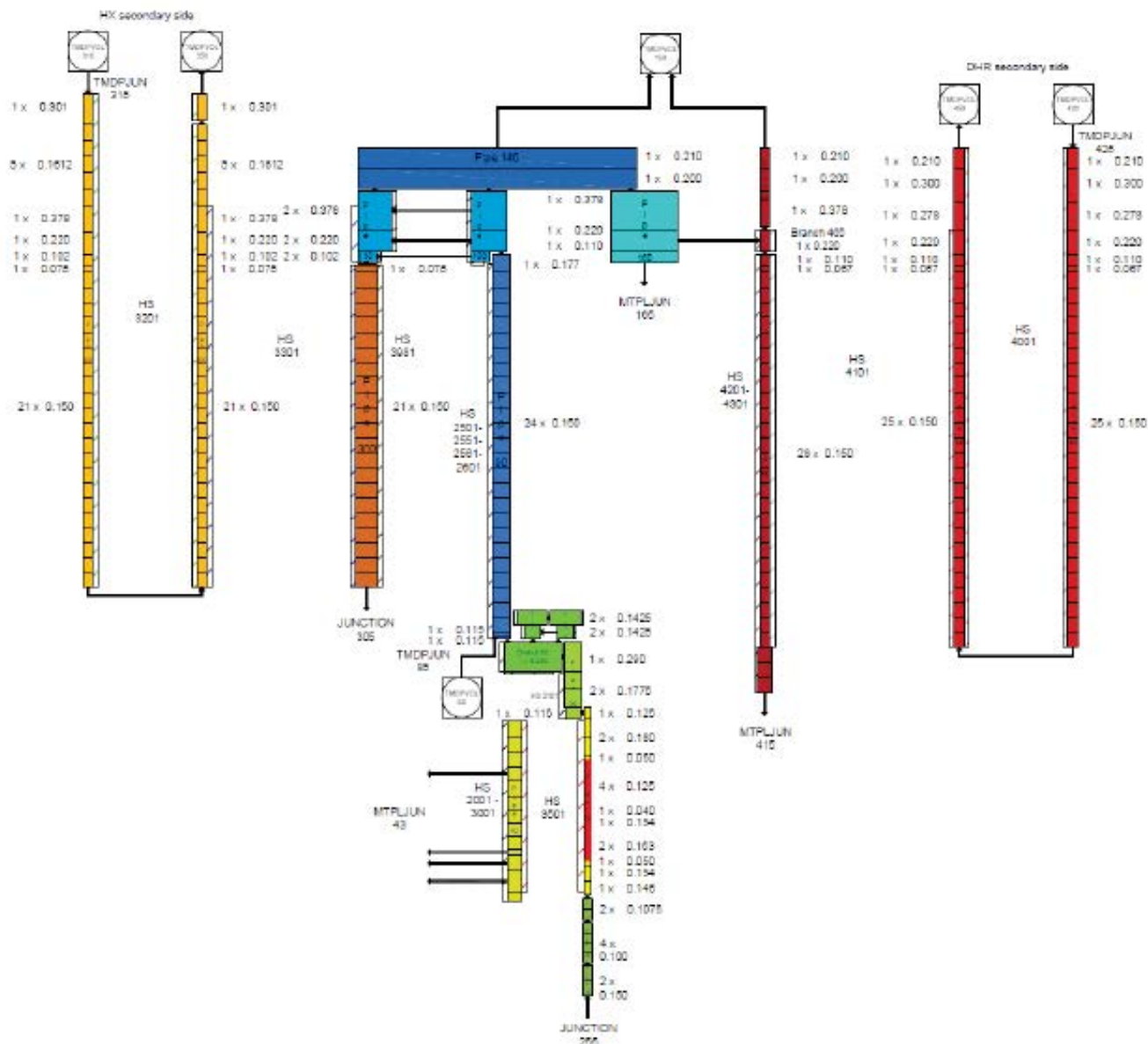
Fig. 2.9 – Nodalization scheme: mono-dimensional model
