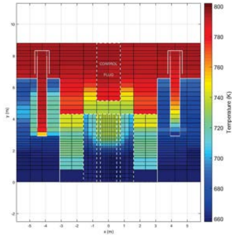
Fig. 3.18 – Transient conditions
