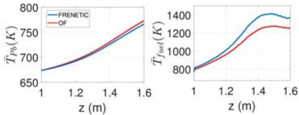
Fig. 5.11 – Axial temperature profile for the coolant (left) and the fuel (right) along the central FA calculated by FRENETIC and OpenFOAM (OF in the legend).
