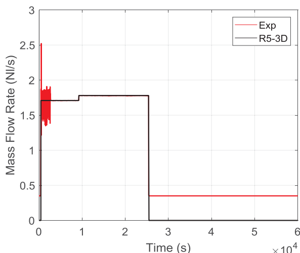
Fig. 2.14 – Argon injection
