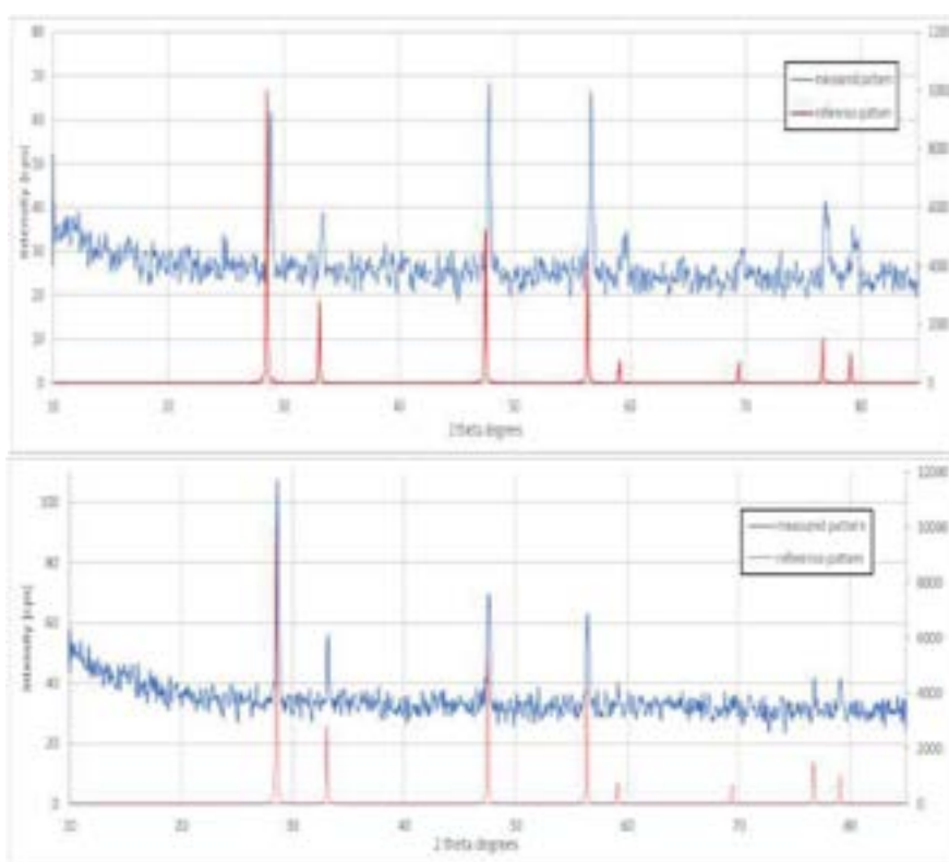
Fig. 8.6 – XRD patterns of \text{Ce}_2\text{O} pellet after reactivity experiment with Pb at 550°C (top) and 750°C (bottom).
