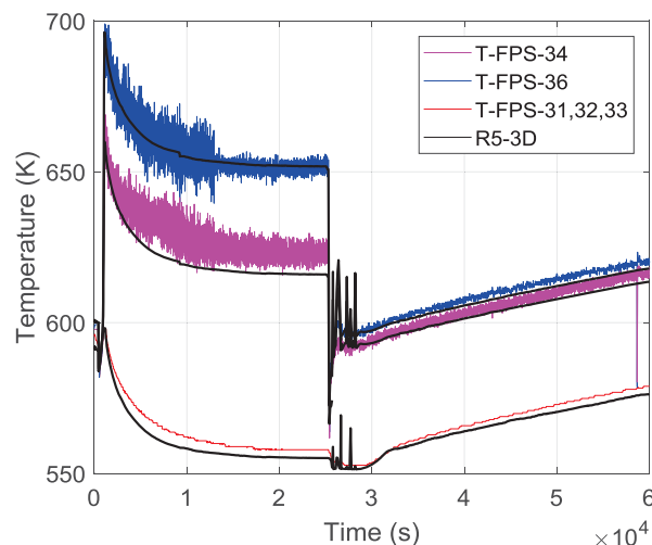
Fig. 2.17 – FPS inlet/outlet temperature
