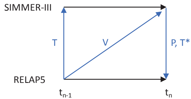
Fig. 7.1 – Data exchange configuration
