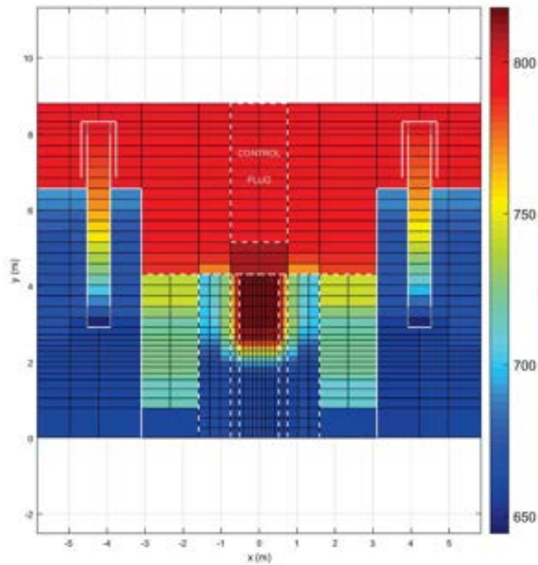
Fig. 3.14 – Steady state conditions
