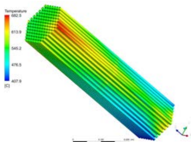
Fig. 9.12 Pin temperature distribution for case2, double sector blockage at the lower spacer grid.
