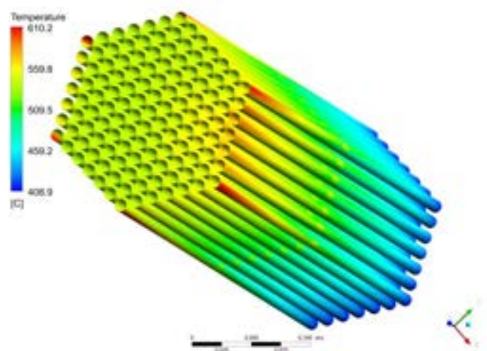
Fig. 9.10 Temperature distribution in the clad for case 1.
