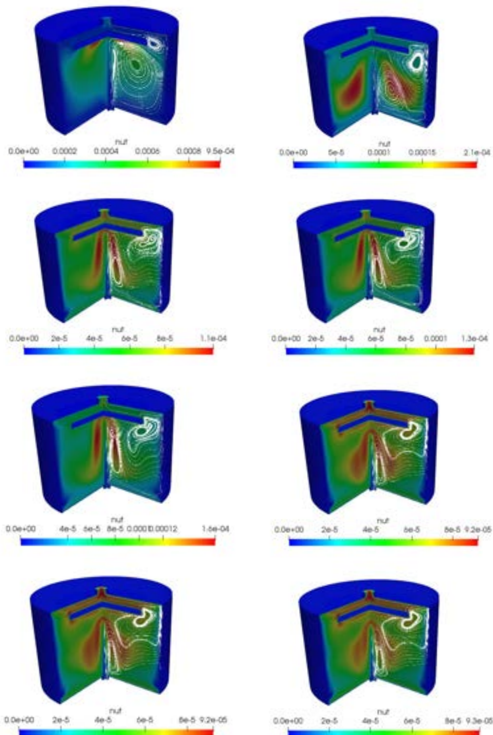
Fig. 4.20 - Turbulent viscosity \nu_t and streamline profiles over the 3D test component at time t = 0, 4, 20, 80, 180, 580, 1780 and 2780 s by using two-equation \kappa-\omega turbulence model in OpenFOAM.
