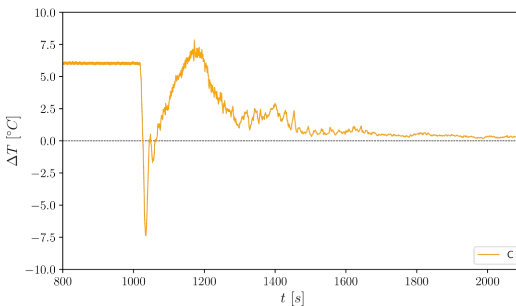
Fig. 4.10 - Different profile between outlet and steel disk temperature values for case C.
