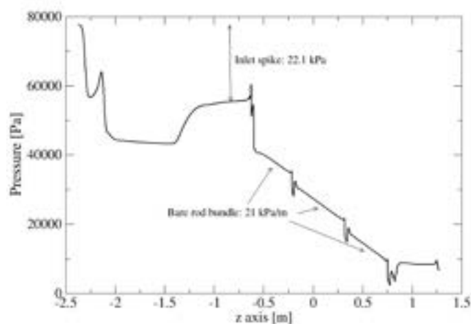
Fig. 9.7 Cross-section averaged pressure distribution along the streamwise direction for case 0.
