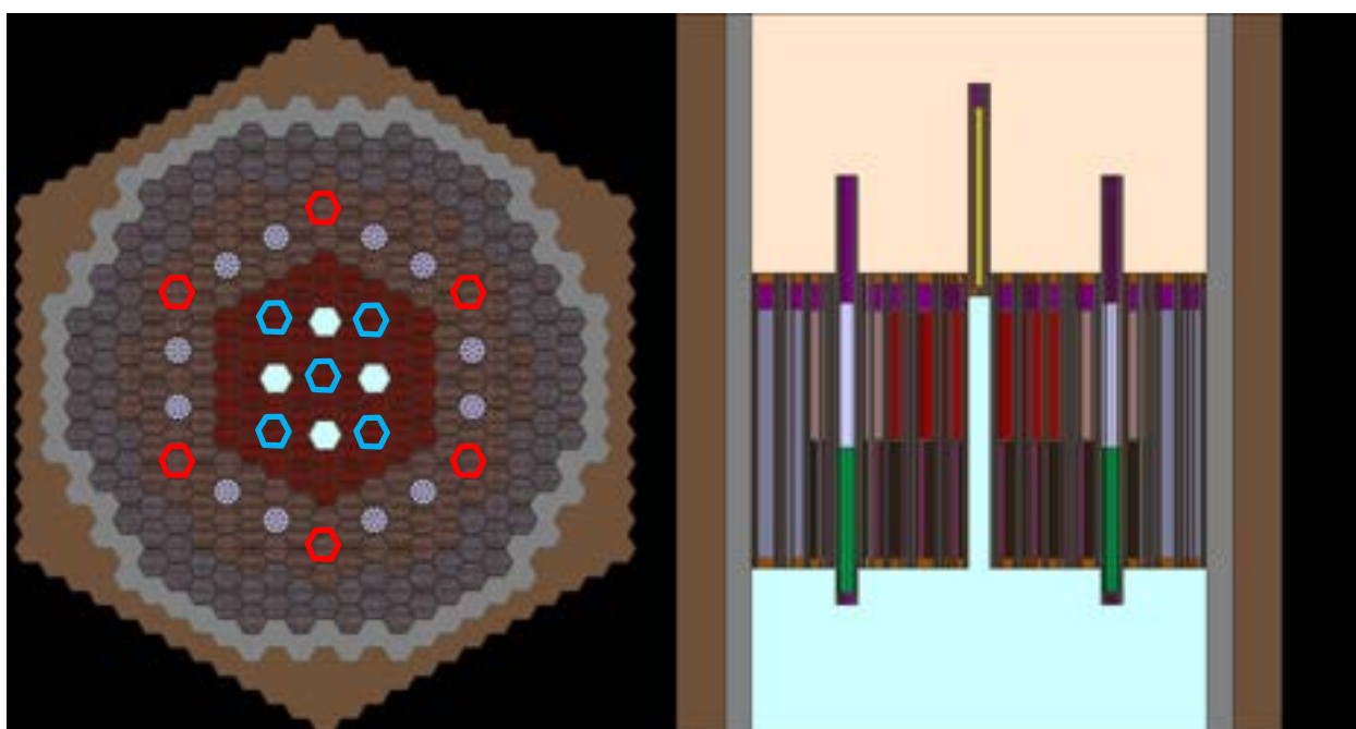
Fig. 5.3 Radial (left) and axial (right) view of the ALFRED configuration simulated in Serpent.
