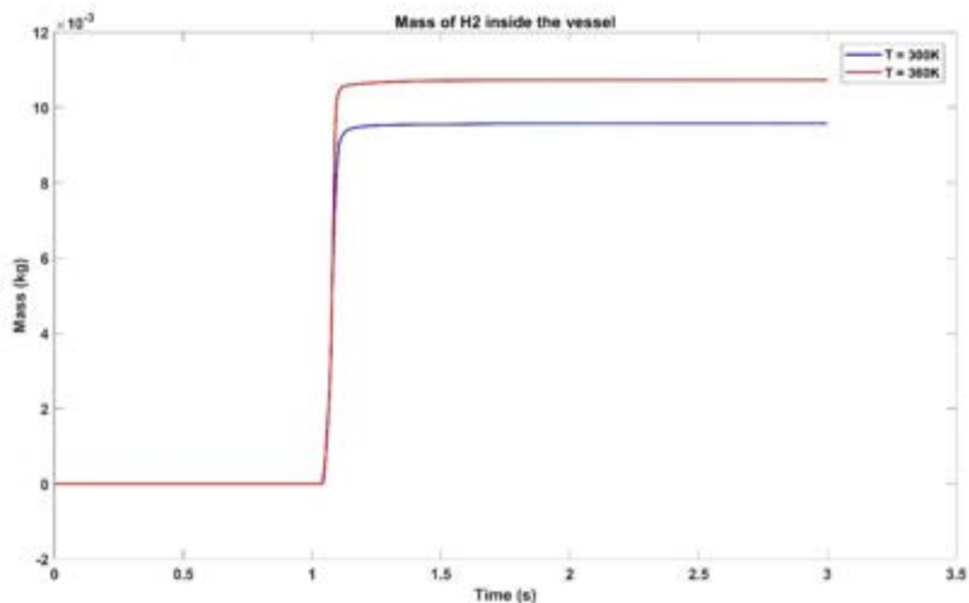
Fig. 7.5 – Time evolution of hydrogen mass inside the vessel
