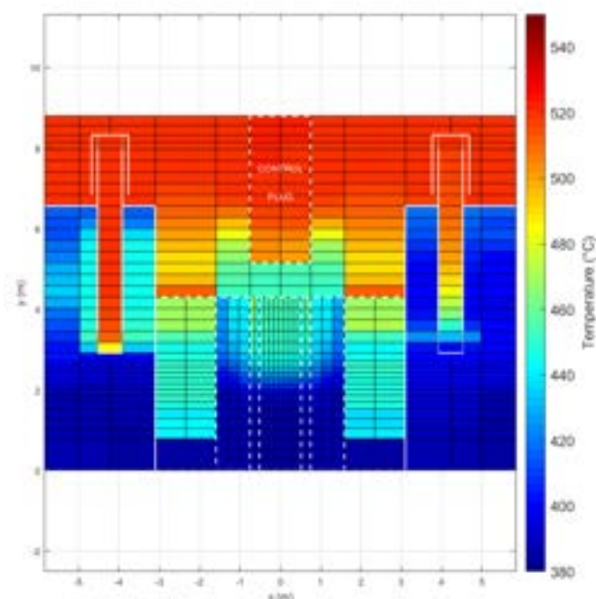
Fig. 3.18 – Transient conditions
