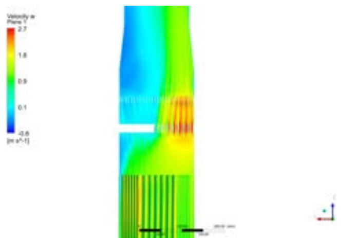
Fig. 9.16 Streamwise velocity contours in the blockage region for case9 (double sector upper blockage).
