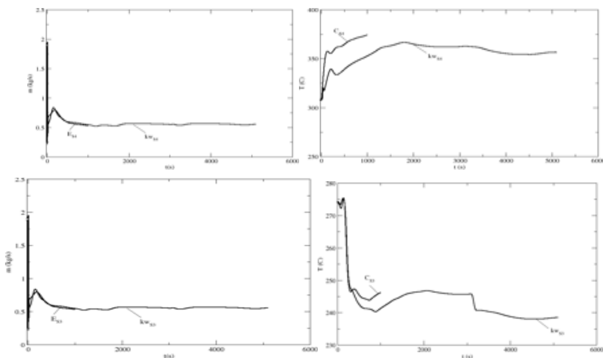
Fig. 4.15 - Cathare standalone simulation. Computed mass flow rate m (left) and temperature (right) at the points S3-S4 of the central leg as a function of time t , from [4.9].
