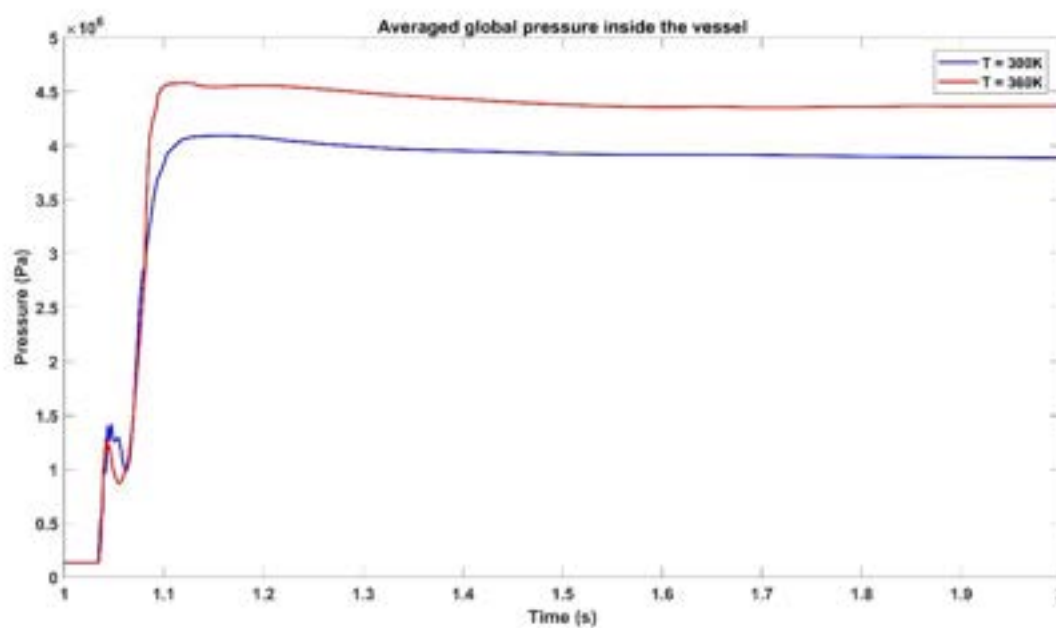
Fig. 7.3 – Time evolution of global pressure in the vessel
