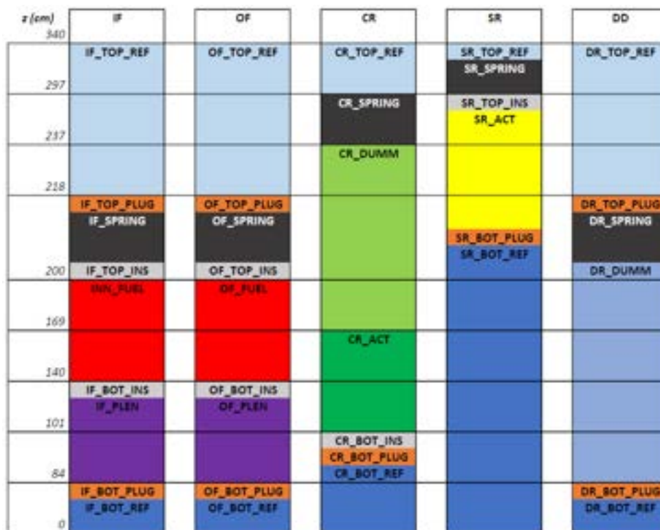
Fig. 5.4: core configuration with rod position adjusted to reach a condition closer to criticality.
