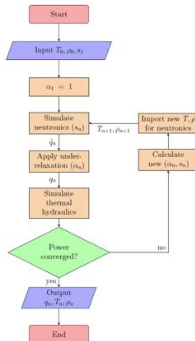
Fig. 6.3 – The stochastic approximation coupling algorithm
