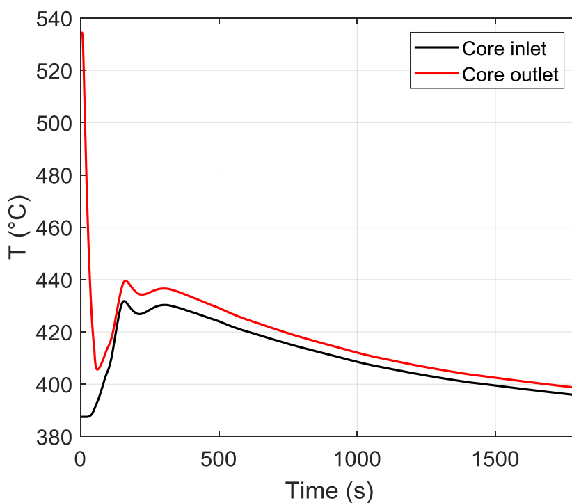
Fig. 3.21 – Core temperature
