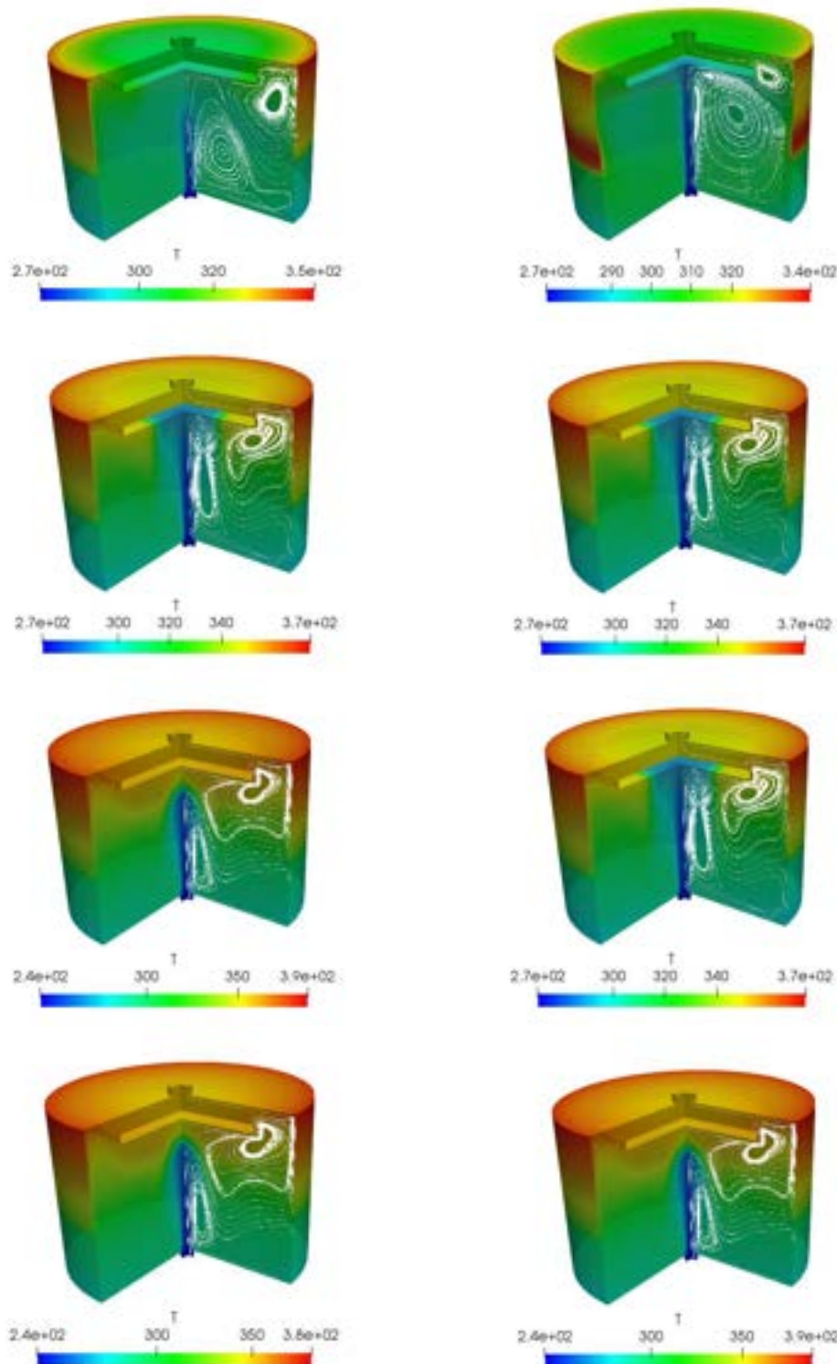
Fig. 4.19 - Temperature T and streamline profiles over the 3D test component at time t = 0, 4, 20, 80, 180, 580, 1780 and 2780 s by using two-equation \kappa\omega turbulence model in OpenFOAM.
