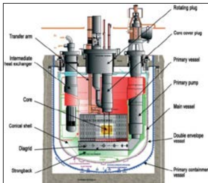
Fig. 3.1 – Reactor block
