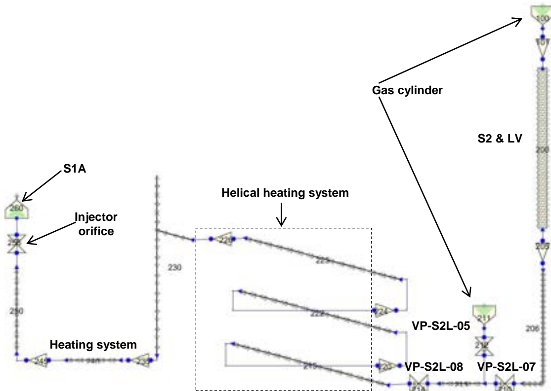
Fig. 30 – RELAP5/Mod3 nodalization of LIFUS5/Mod3 injection line.
