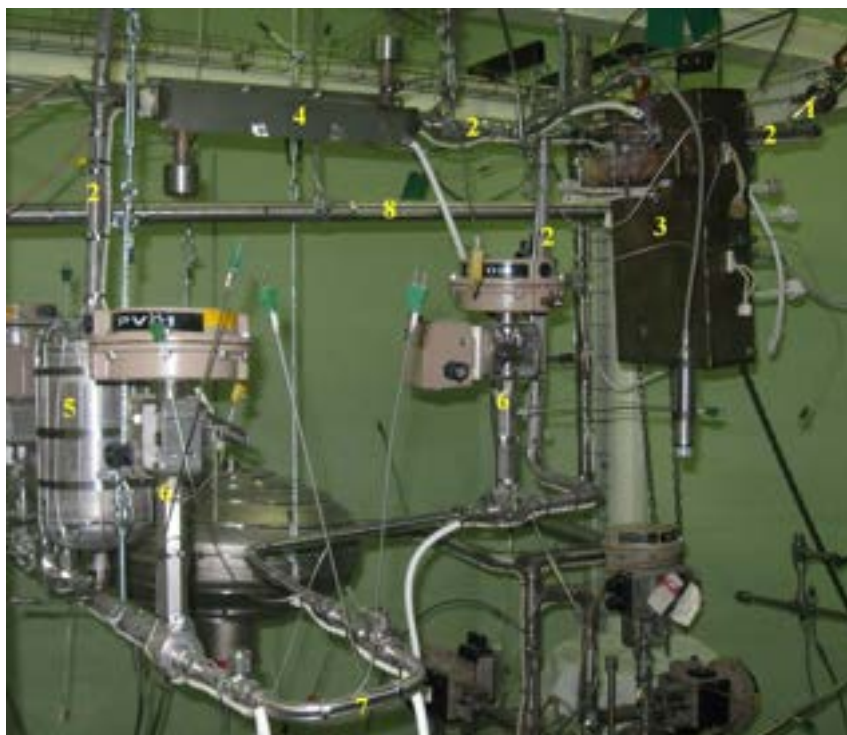
Figure 2: Overview of the purification loop. 1 : regulating valve (connection to the main loop); 2 : purification loop pipe; 3 : Resistivity Meter; 4 : Air cooler upstream of the Cold Trap; 5 : Cold Trap; 6 : pneumatic valves to permit/exclude Lithium circulation in the sampling tube; 7 : Sampling “U” tube (Sampler 1); 8 : pipeline of the main Lifus 6 loop (behind purification pipe, in the figure)
