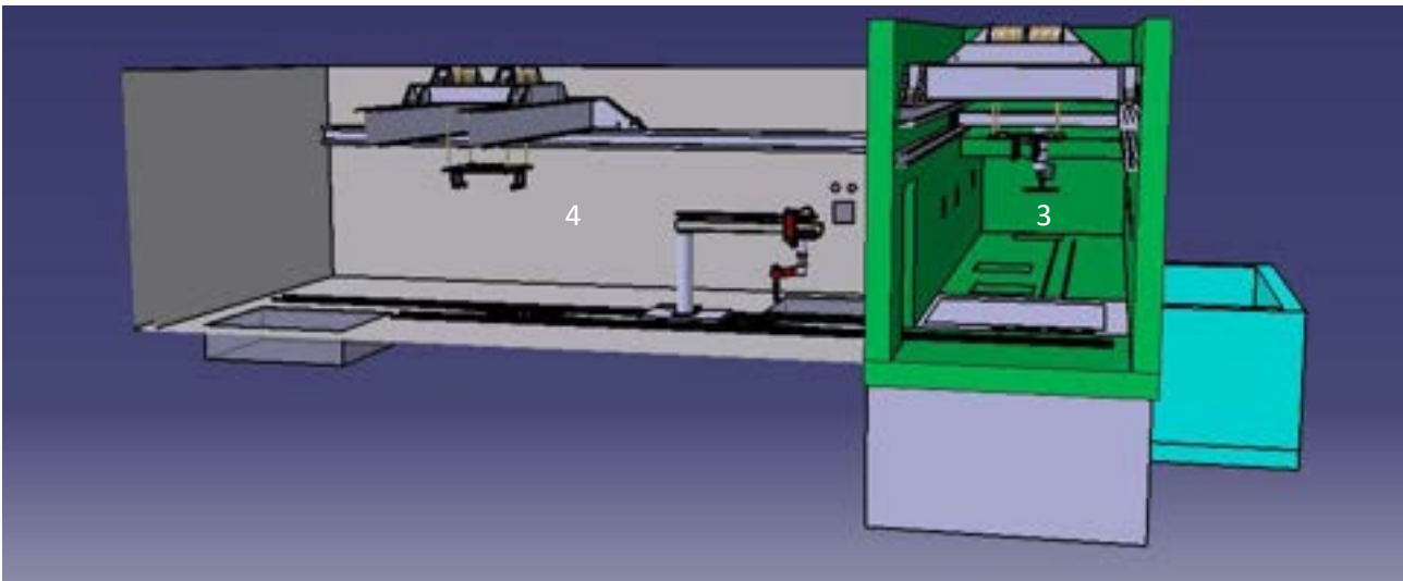
Fig. 7 AC modifications (Section view)
