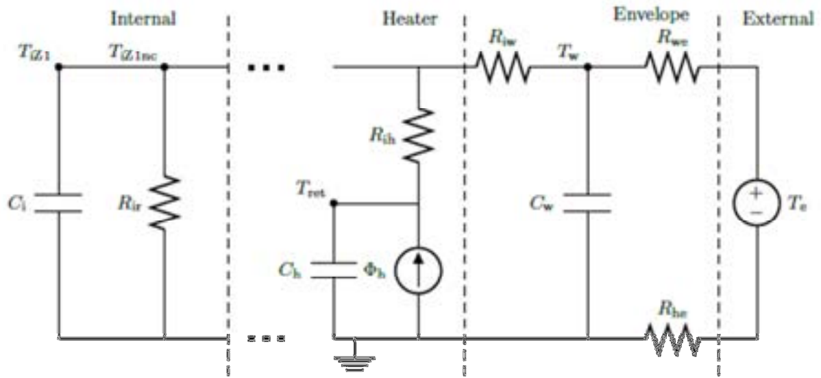
Figura 2.38 circuito T_i T_w T_{ret} T_{inc} T_{flow}
