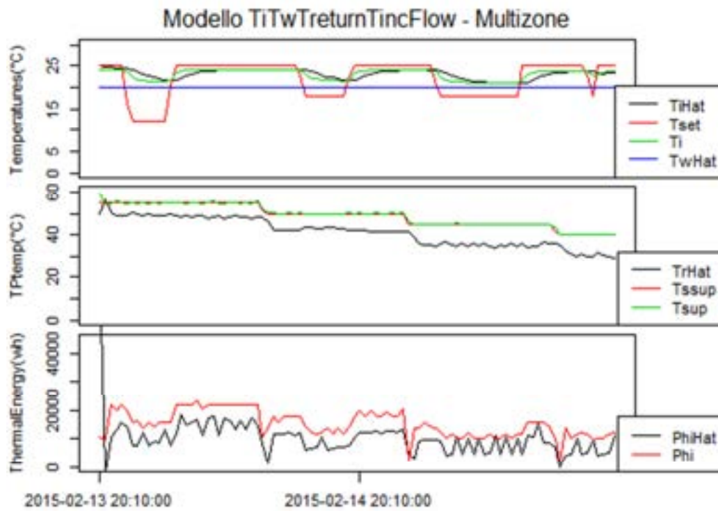
Figura 2.39 circuito T_iT_wT_{return}T_{inc}Flow
