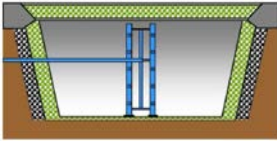
Figure 19: Cross sectional drawing of a PTES and picture of a PTES construction in Marstal (PlanEnergi 2012).
