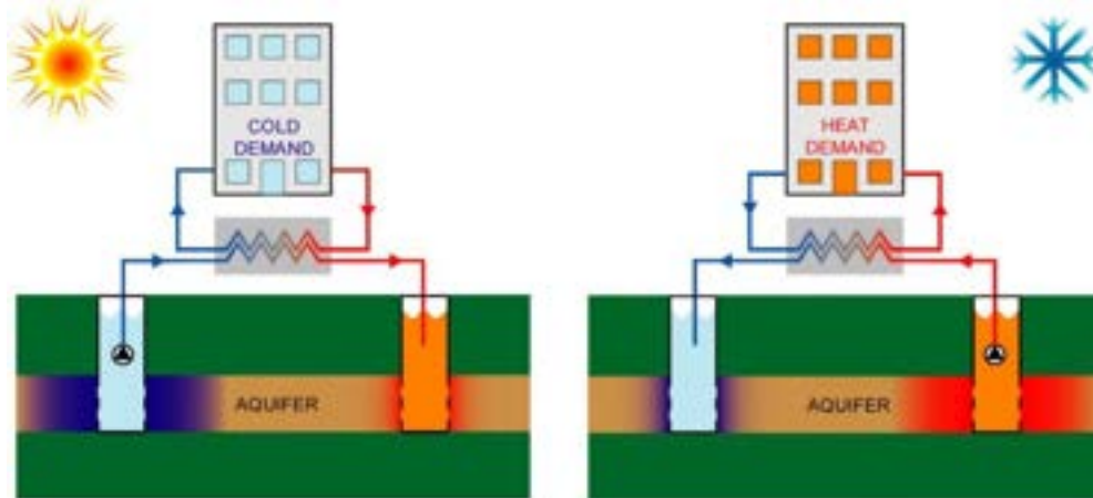
Figure 13: Aquifer Thermal Energy Storage concept [20].
