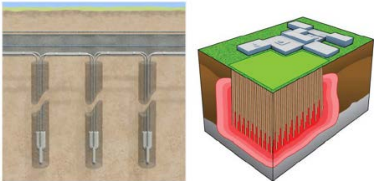
Figure 21: Cross sectional drawing of a BTES and Three-dimensional drawing of BTES www.bbeatty.com/geothermal.php
