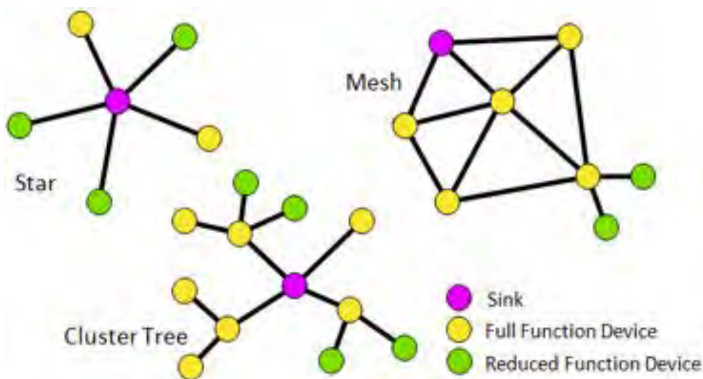
Figura 29 Topologie WSN
