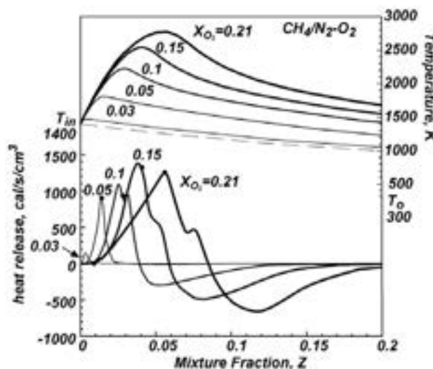
Fig. 3 Temperature (upper part) and heat release rate (lower part) versus mixture fraction, parametric on X_{O_2} at T_o = 300\text{K} , T_{in} = 1400\text{K} and p = 10\text{bar} .
