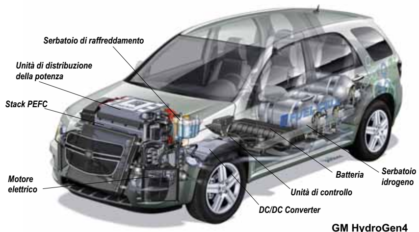
GM HydroGen4
