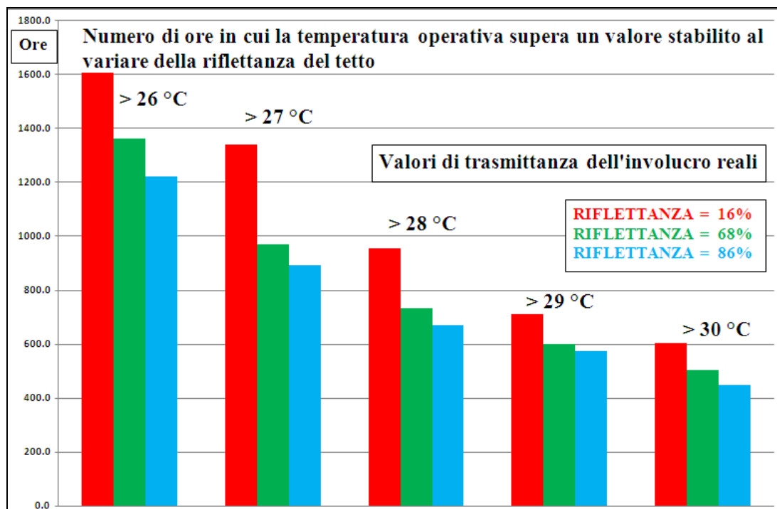
Figura 16: Temperature operative, isolamento reale
