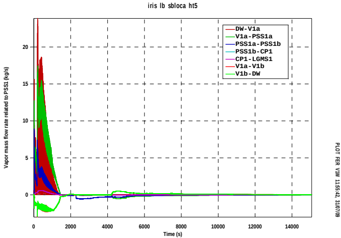
Fig.A9. 21 IRIS PSS1 vapor mass flowrate
