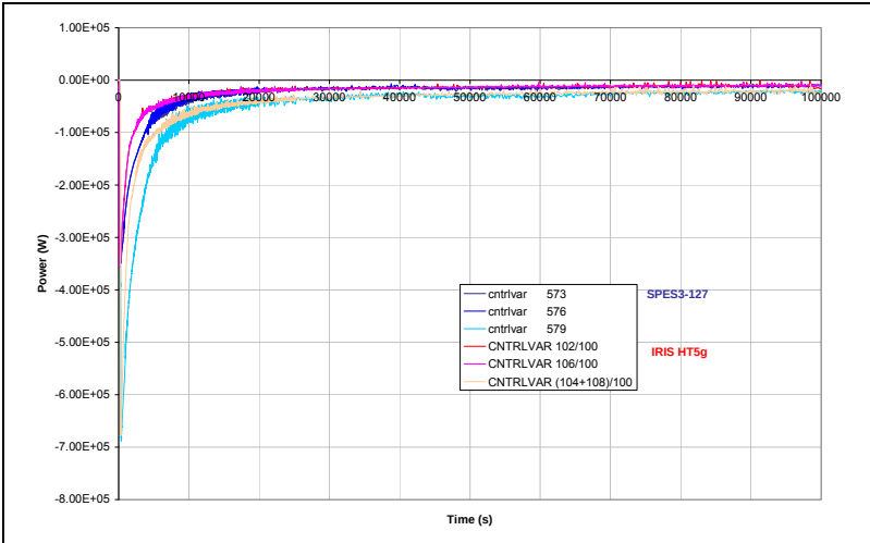
Fig.A13. 15 SPES3-127 and IRIS HT5g EHRS power
