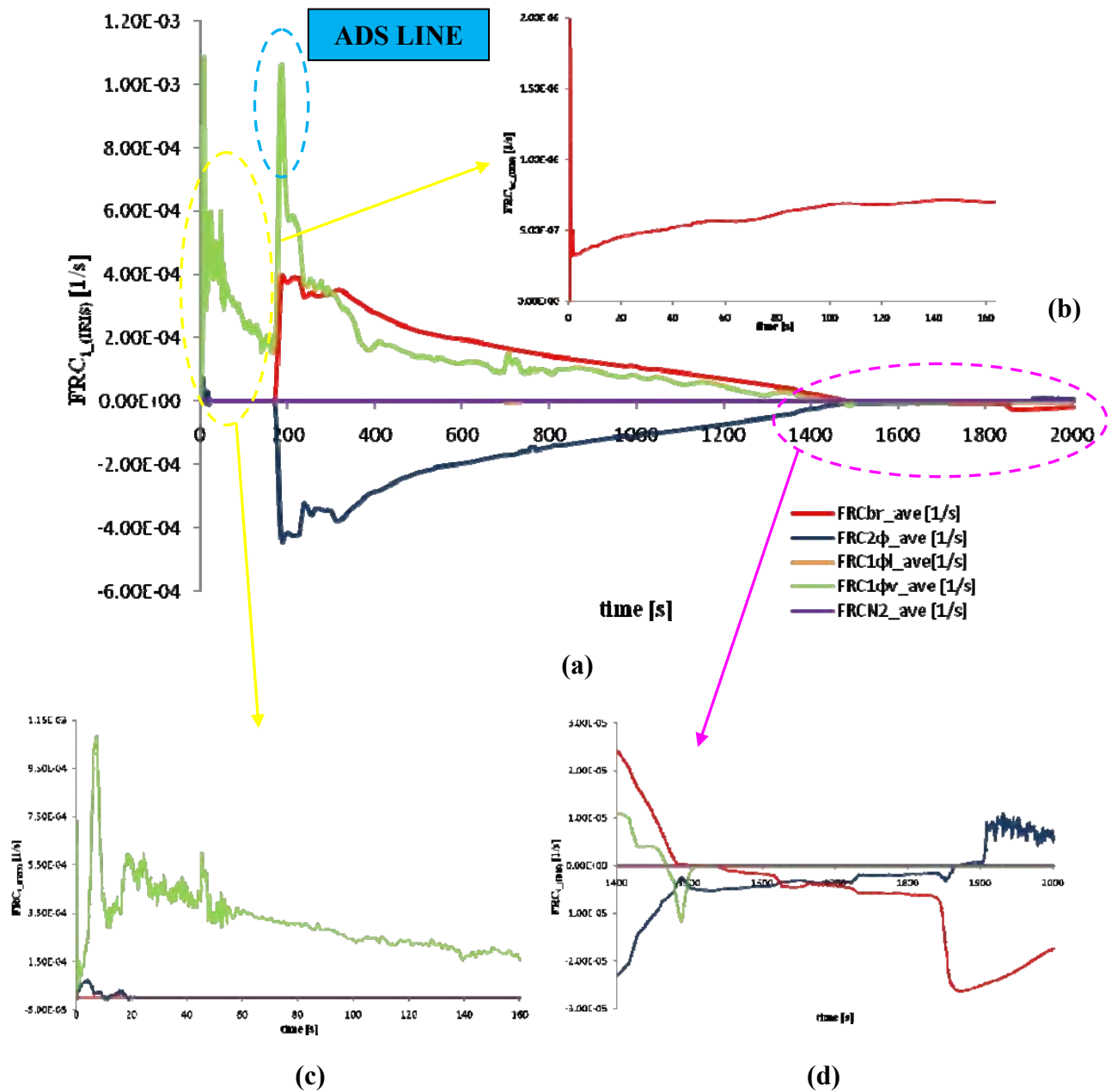
Fig.A13. 23 : (a) FRCs' trend in IRIS BPE (b) zoom on the FRC br and (c) on FRC 1φv and FRC 2φ for the first 160 s of IRIS DVI-SBLOCA transient, (d) zoom from 1400 s to 2000s
