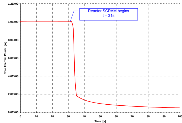
Fig.A13. 46 Reactor Power vs Time
