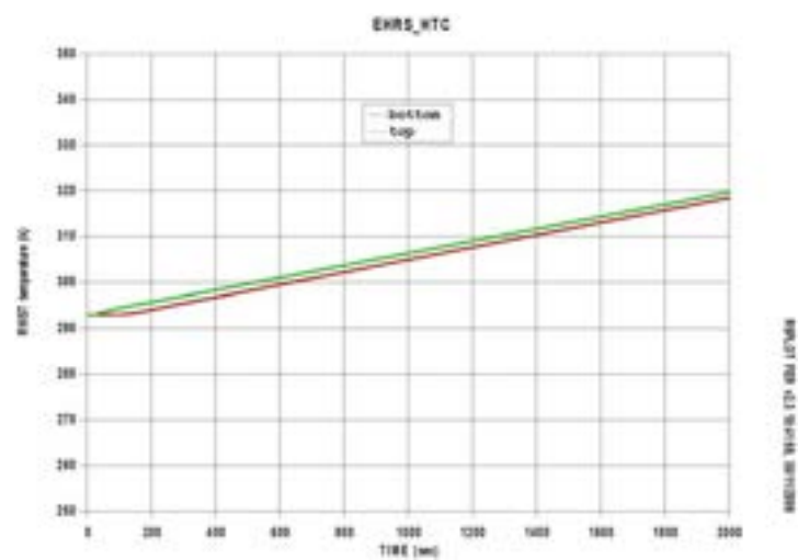
Fig.A13. 2 EHRS-RWST IRIS stand alone model RWST temperature
