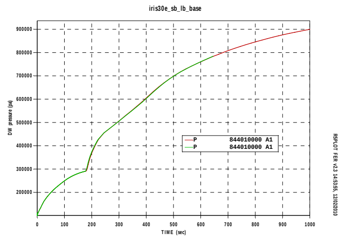
Fig.A17. 4 DW pressure
