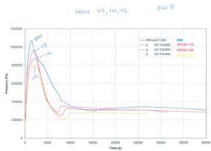
Fig.A8. 3 SPES3-119, 120, 122 and IRIS DW pressure
