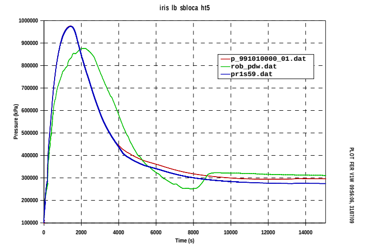
Fig.A9. 15 IRIS DW pressure
