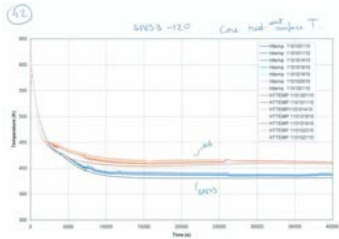
Fig.A8. 45 SPES3-120 core heting rod outer surface temperature
