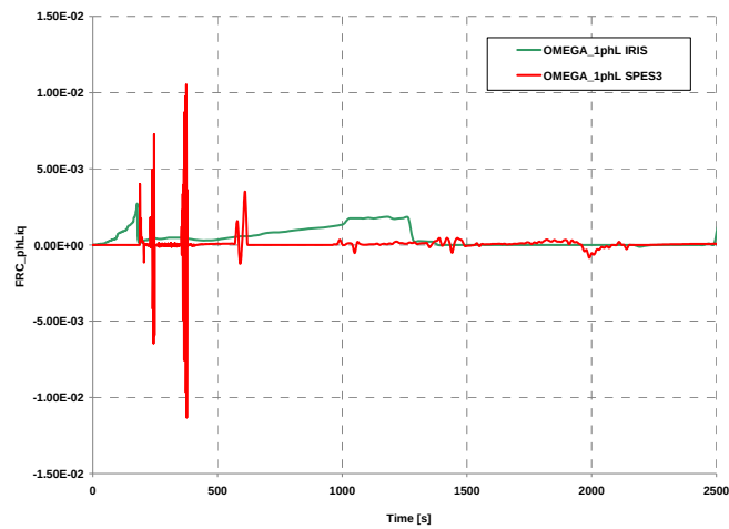
Fig.A13. 93 Omega 1pL IRIS vs SPES3
