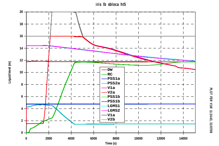
Fig.A9. 17 IRIS containment tank liquid level
