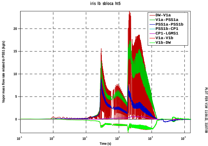
Fig.A9. 22 IRIS PSS1 vapor mass flowrate
