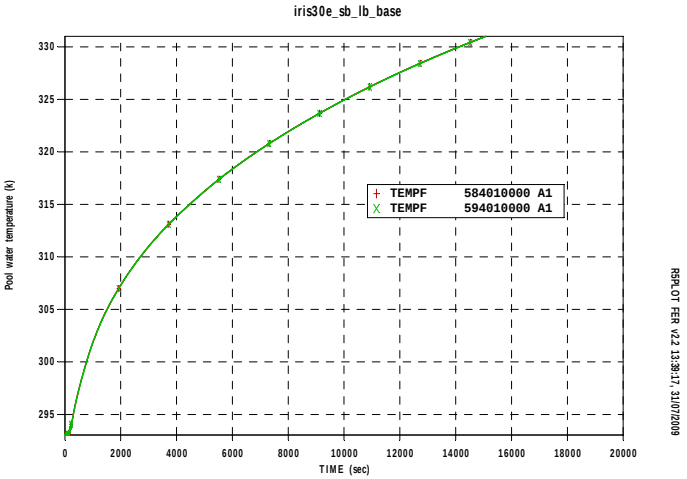
Fig.A9. 13 IRIS RWST water temperature
