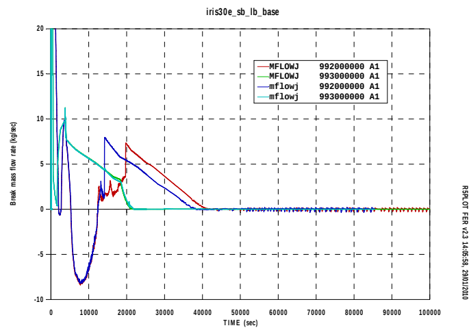
Fig.A16. 4 LGMS mass flow
