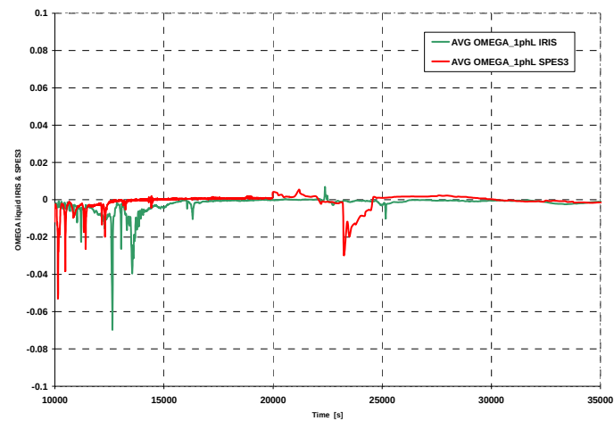
Fig.A13. 119 AVG OMEGA liquid phase IRIS & SPES3 vs time
