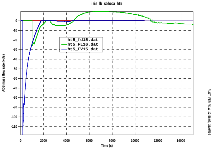
Fig.A9. 27 IRIS ADS mass flowrate
