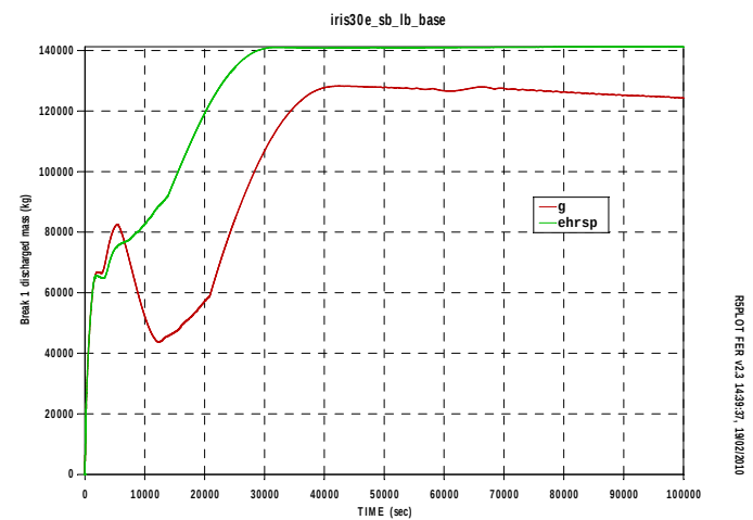
Fig.A18. 7 Break discharged mass
