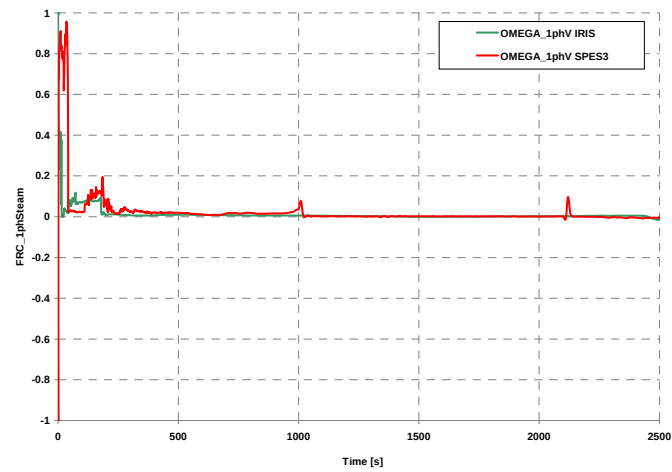
Fig.A13. 94 Omega 1pV IRIS vs SPES3
