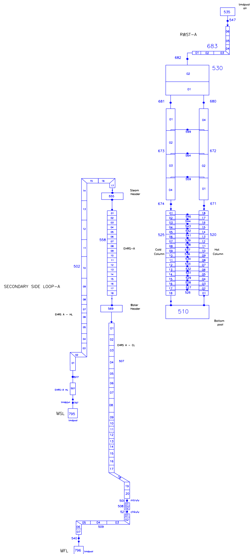
Fig.A12. 1 SPES3 EHRW-RWST stand alone RELAP model
