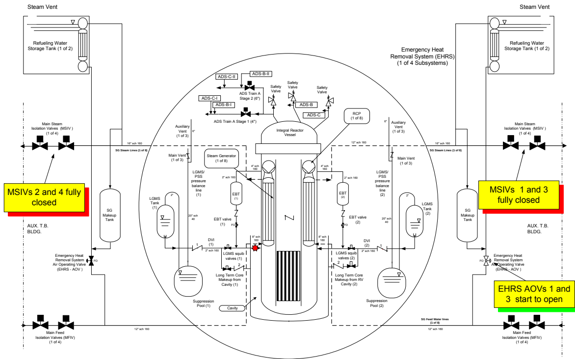
Fig.A13. 51 EHR-AOV 1-3 starts opening
