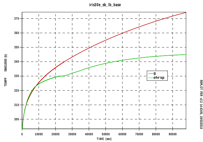
Fig.A18. 9 RWST liquid temperature
