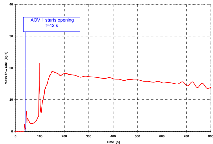
Fig.A13. 52 mass flow rate vs time
