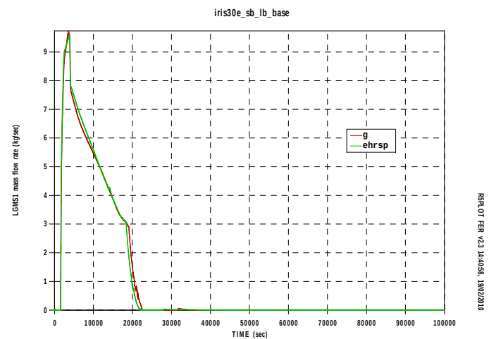
Fig.A18. 8 LGMS mass flowrate
