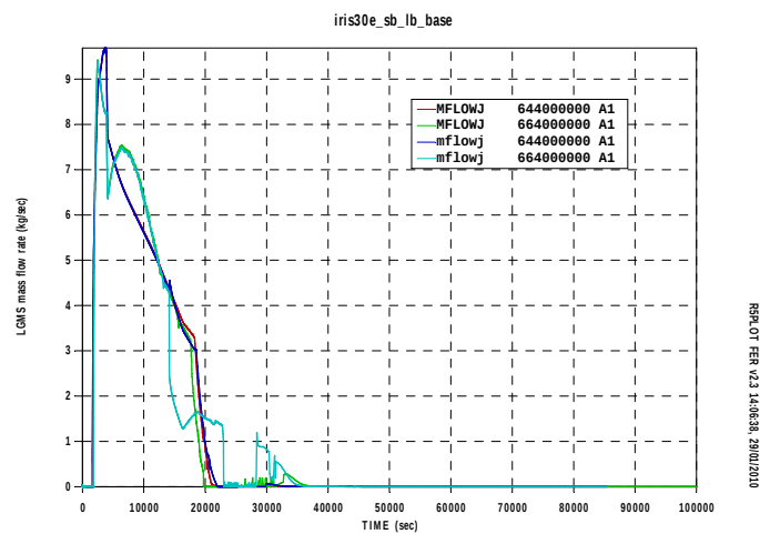
Fig.A16. 5 LGMS delivered mass
