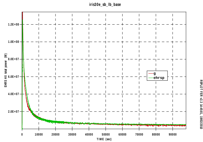
Fig.A18. 11 EHRX HX total power
