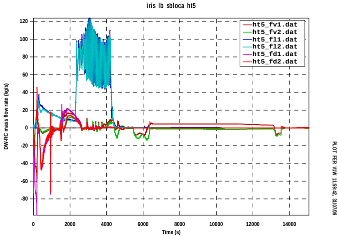
Fig.A9. 23 IRIS DW-RC mass flowrate
