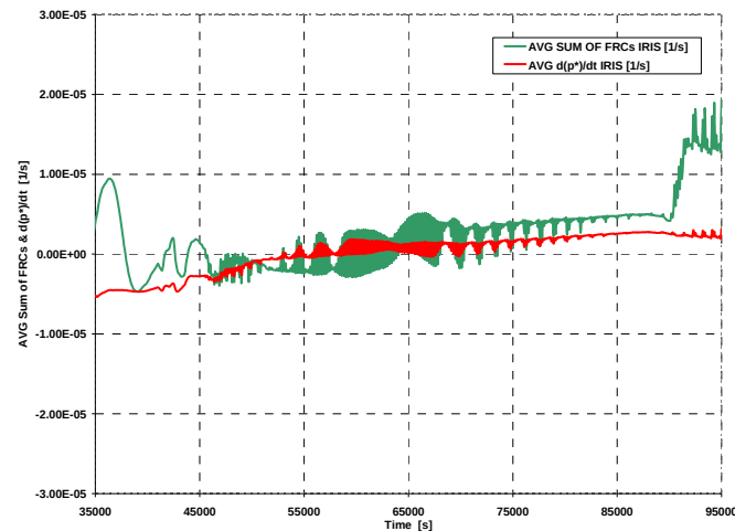
Fig.A13. 105 AVG sum of FRCs 1 AVG d(p*)/dt IRIS vs time
