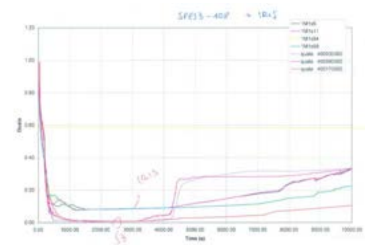
Fig.A8. 1 SPES3-108 and IRIS DW non-condensable quality
