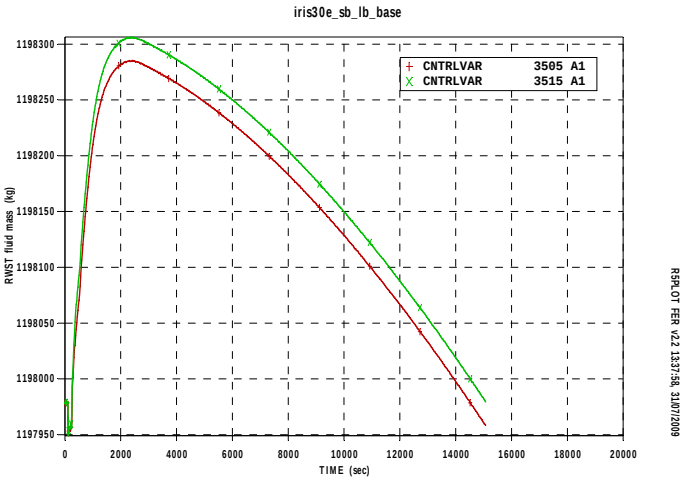
Fig.A9. 12 IRIS RWST fluid mass
