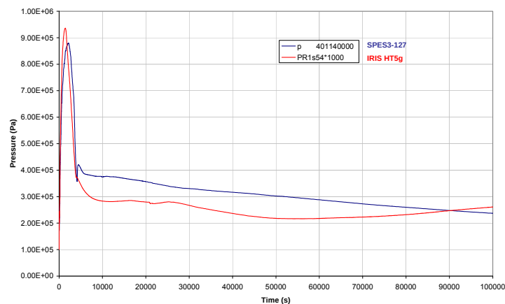
Fig.A10. 1 DW pressure
