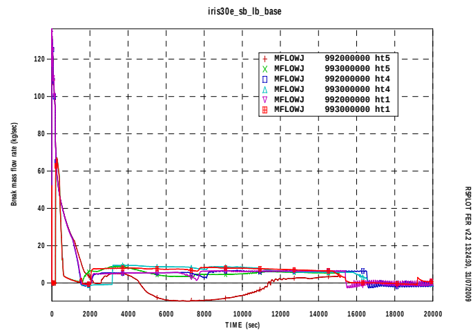
Fig.A9. 2 IRIS break mass flow
