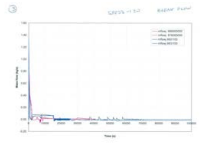
Fig.A8. 6 SPES3-120 break flow
