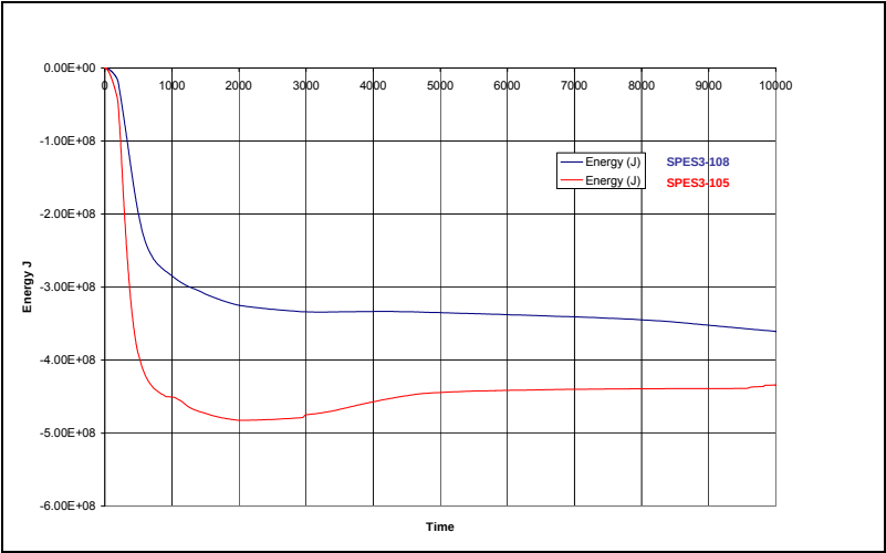
Fig.A4. 3 Energy to DW heat structures
