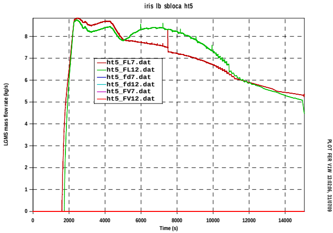
Fig.A9. 29 IRIS LGMS mass flowrate
