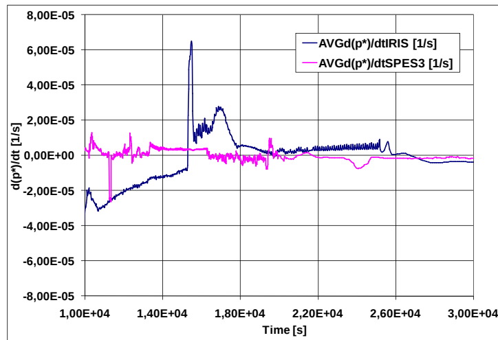
Fig.A13. 29 Average dimensionless pressure gradient in IRIS and SPES3 vs time
