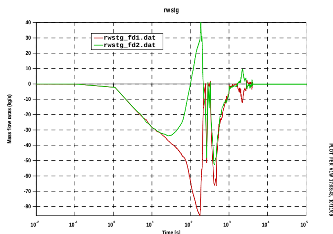
Fig.A10. 11 Containment connection mass flowrates
