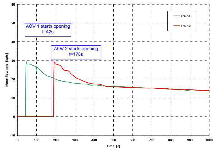
Fig.A13. 57 EHRIS Train 1 and 2 Mass flow rate vs time
