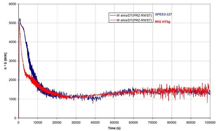
Fig.A10. 8 RWST temperatures
