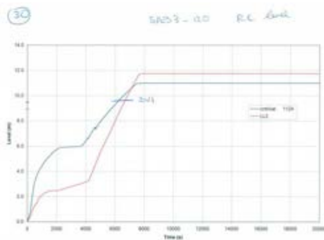
Fig.A8. 33 SPES3-120 RC level
