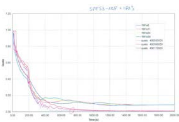
Fig.A8. 2 SPES3-108 and IRIS DW non-condensable quality (short term)
