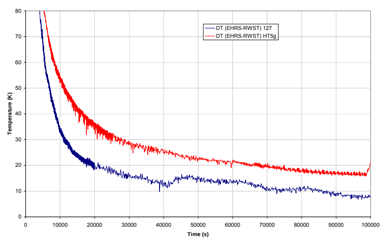
Fig.A10. 4 T (EHRS) – T (RWST)
