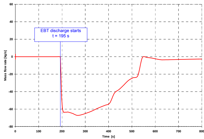
Fig.A13. 62 EBT mass flow rate vs time
