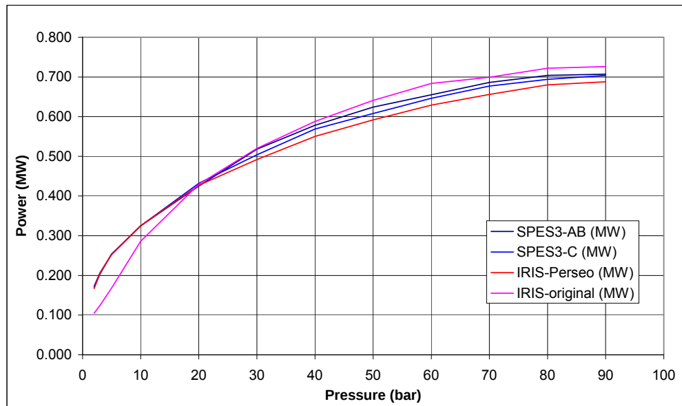
Fig.A17. 1 EHRS-RWST stand alone models SPES3 and IRIS exchanged power parametric comparison
