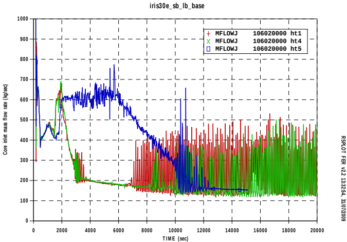
Fig.A9. 8 IRIS core inlet mass flow
