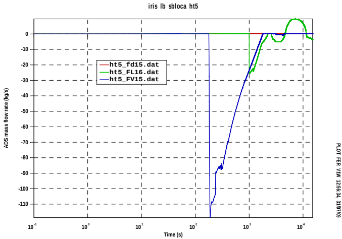
Fig.A9. 28 IRIS ADS mass flowrate
