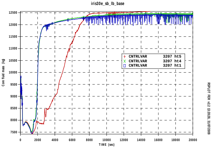
Fig.A9. 6 IRIS core fluid mass
