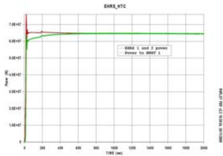
Fig.A13. 1 EHRS-RWST IRIS stand alone model EHRS and RWST power
