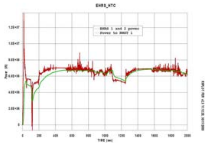
Fig.A13. 3 EHRWST IRIS stand alone model EHRWST and RWST power
