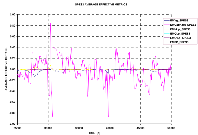
Fig.A15. 12 SPES3 averaged effective metrics from 25000s up to 50000s
