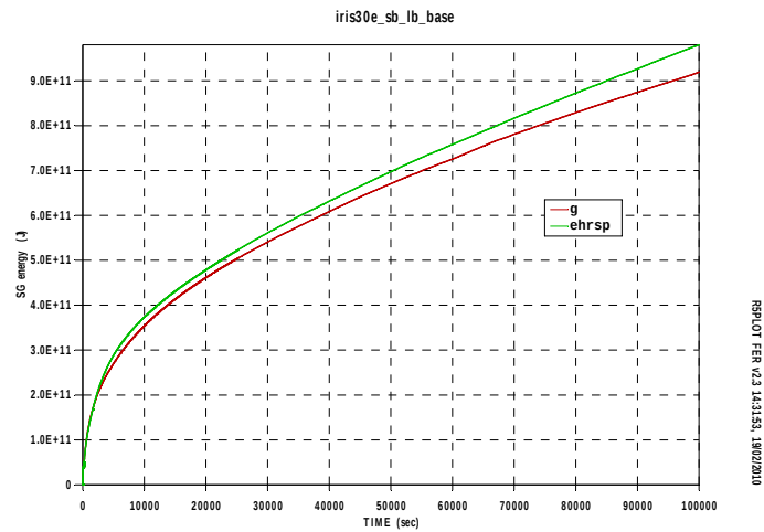
Fig.A18. 3 SG energy
