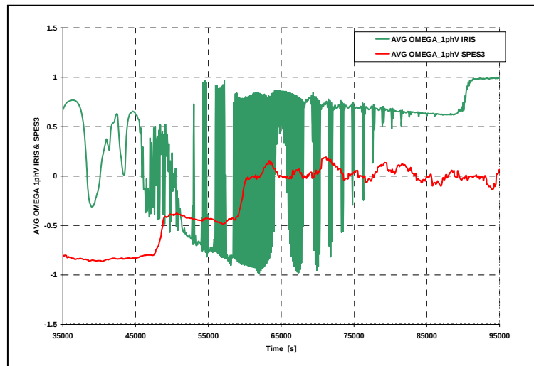
Fig.A13. 123 AVG OMEGA vapor phase IRIS & SPES3 vs time
