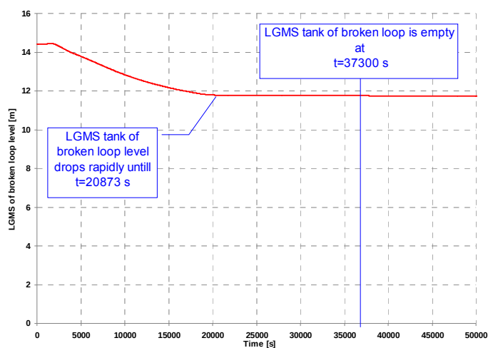
Fig.A13. 74 LGMS (broken loop) level vs time
