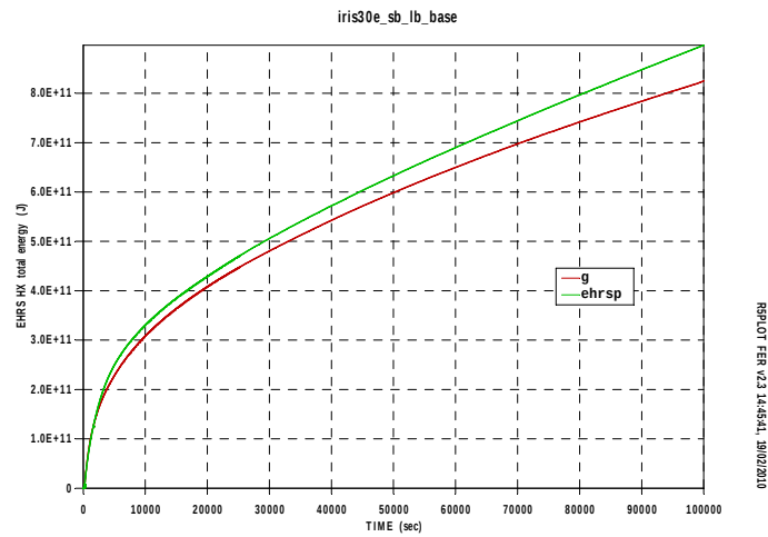
Fig.A18. 10 EHRX HX total enery
