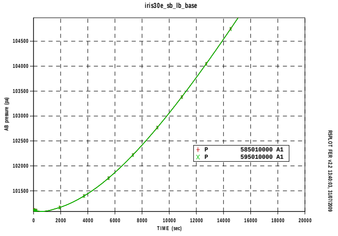
Fig.A9. 14 IRIS RWST pressure
