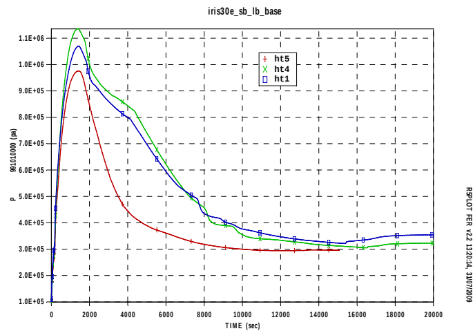
Fig.A9. 1 IRIS DW pressure
