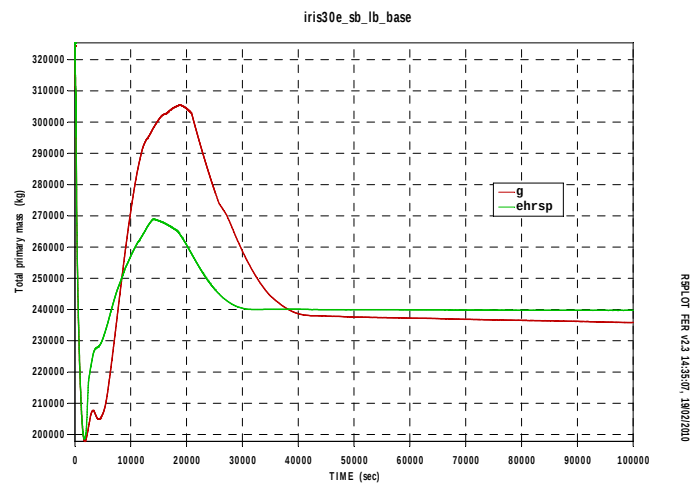
Fig.A18. 4 Total primary mass
