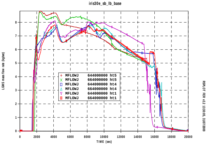
Fig.A9. 7 IRIS LGMS to DVI mass flow
