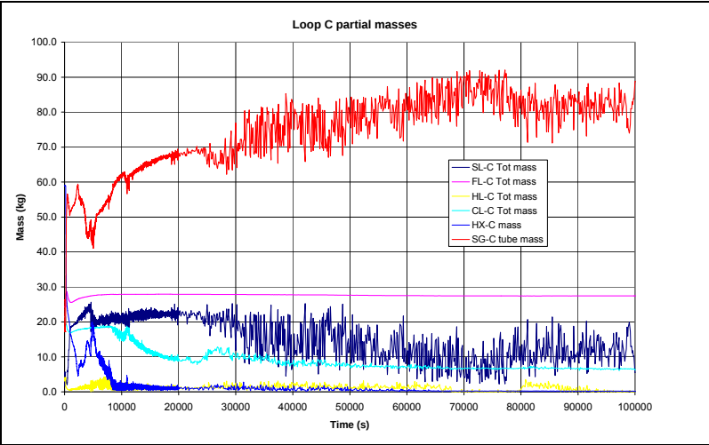
Fig.A14. 4 Loop C partial mass
