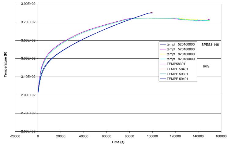
Fig.A19. 1 RWST liquid temperature
