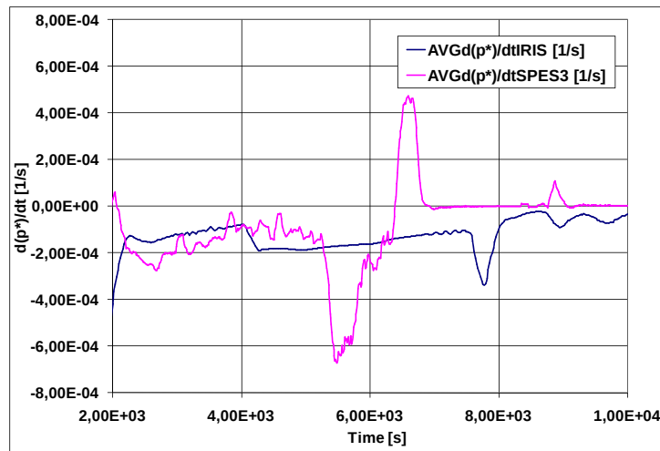
Fig.A13. 28 Average dimensionless pressure gradient in IRIS and SPES3 vs time
