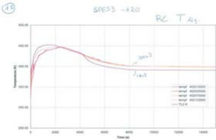
Fig.A8. 18 SPES3-120 RC liquid temperature
