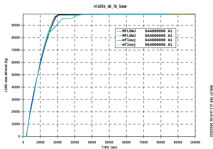
Fig.A16. 6 Mass from cavity
