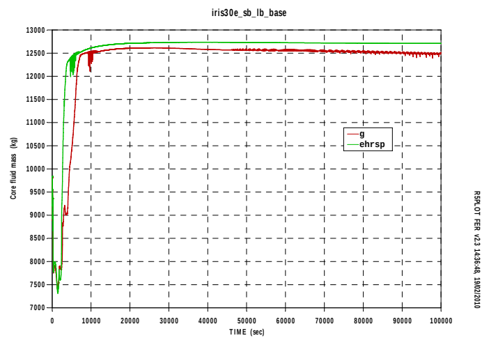
Fig.A18. 5 Core fluid mass
