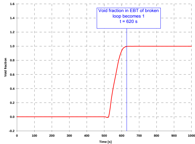
Fig.A13. 65 void fraction vs time
