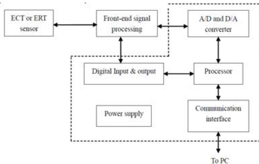
Fig. 87: Block diagram of ECT or ERT system
