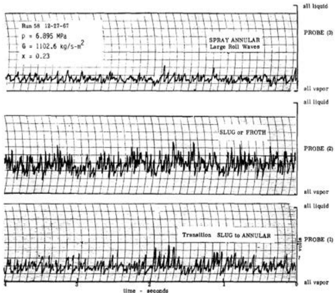
Fig. 107: Electric probe signals displaying different flow regimes (Rouhani et Sohal (1982) from Bergles et al. (1968))
