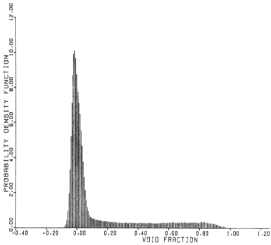
Fig. 109: PDF of bubbly flow (Jones and Zuber (1975)).
