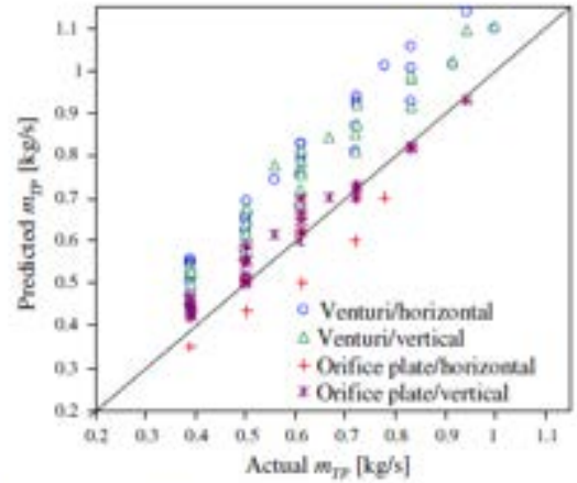
Fig. 12. Comparison between experimental two-phase mass flow rate and that predicted according to Zhang et al. [5].
