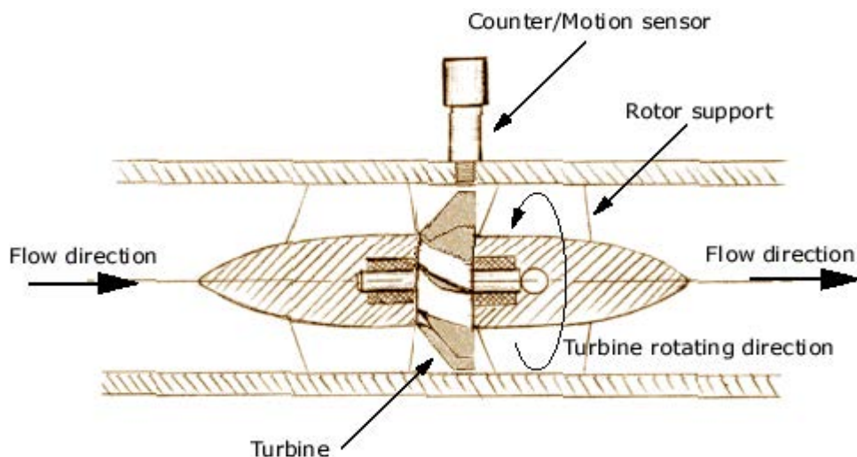
Fig. 6: Axial turbine flowmeter
