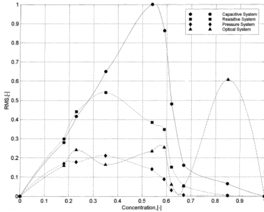
Fig. 115: Comparison of RMS values of each signal obtained from four methods at different flow pattern (Keska (1998))
