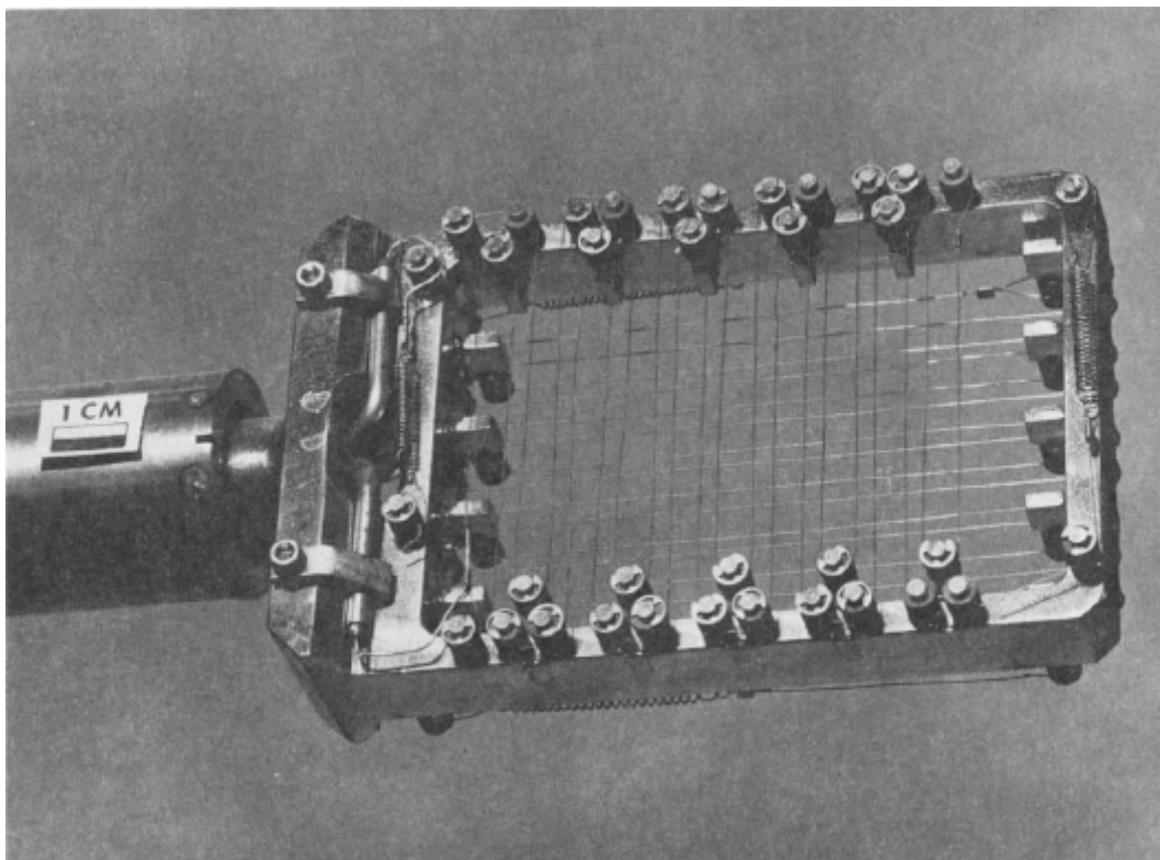
Fig. 81: String probe used by Hardy et al. (1983)
