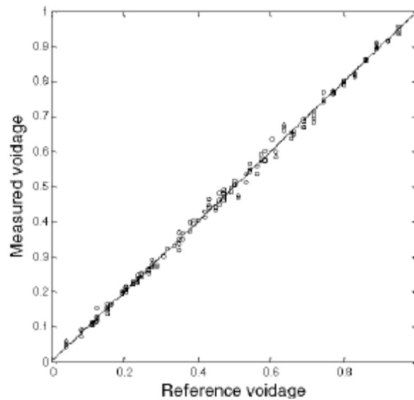
Fig. 100: Comparison between measured and reference void fraction (Li et all (2008))
