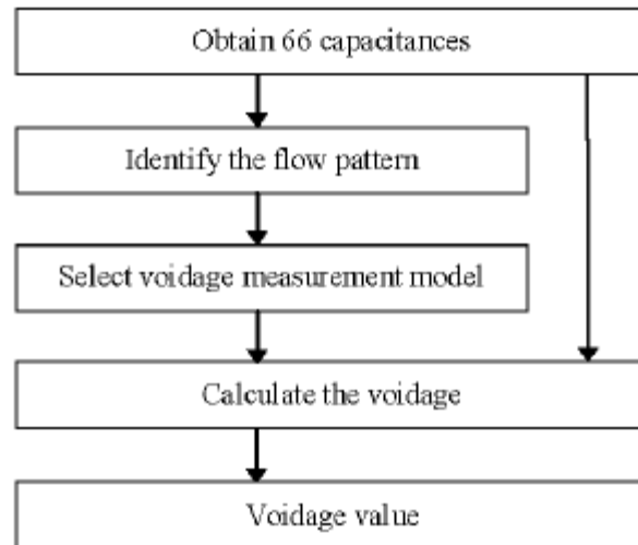
Fig. 99: Voidage measurement process (Li et all (2008))
