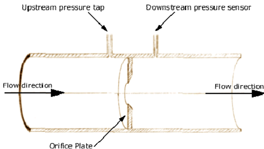
Fig. 29: Orifice Flowmeter
