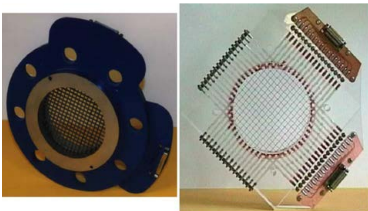
Figura 19: Wire mesh sensor
