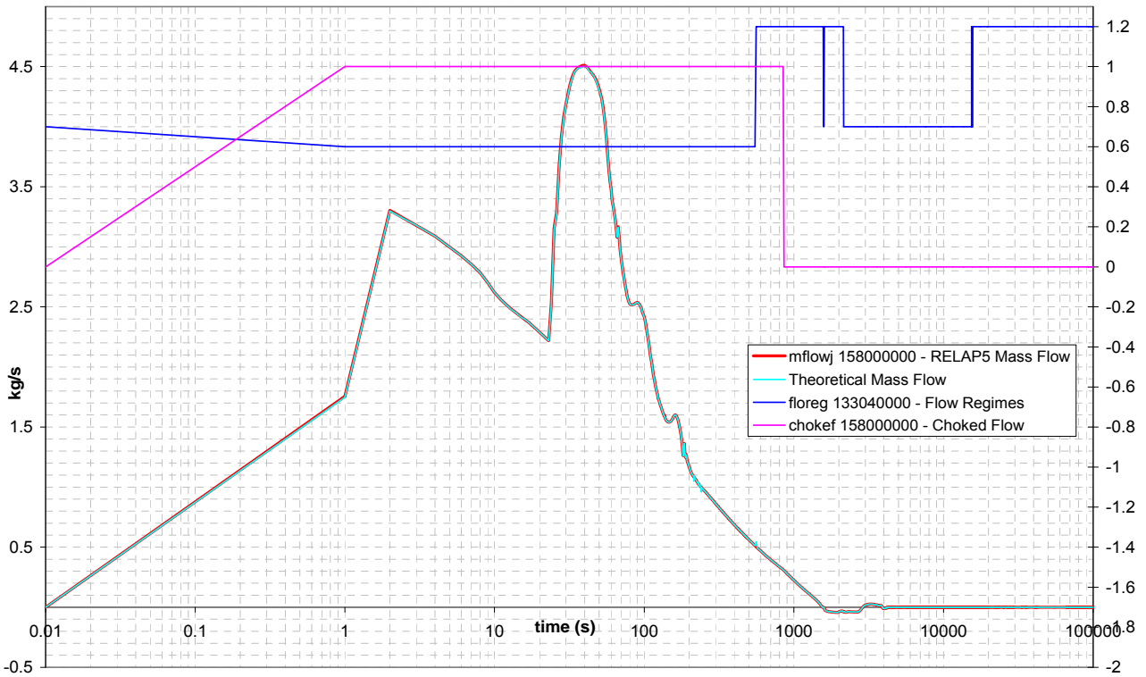
Figure 5.15: Comparison between the RELAP5 and theoretical mass flow, flow regimes and presence of critical flow in ADS SPLIT beak line, ADS Test
