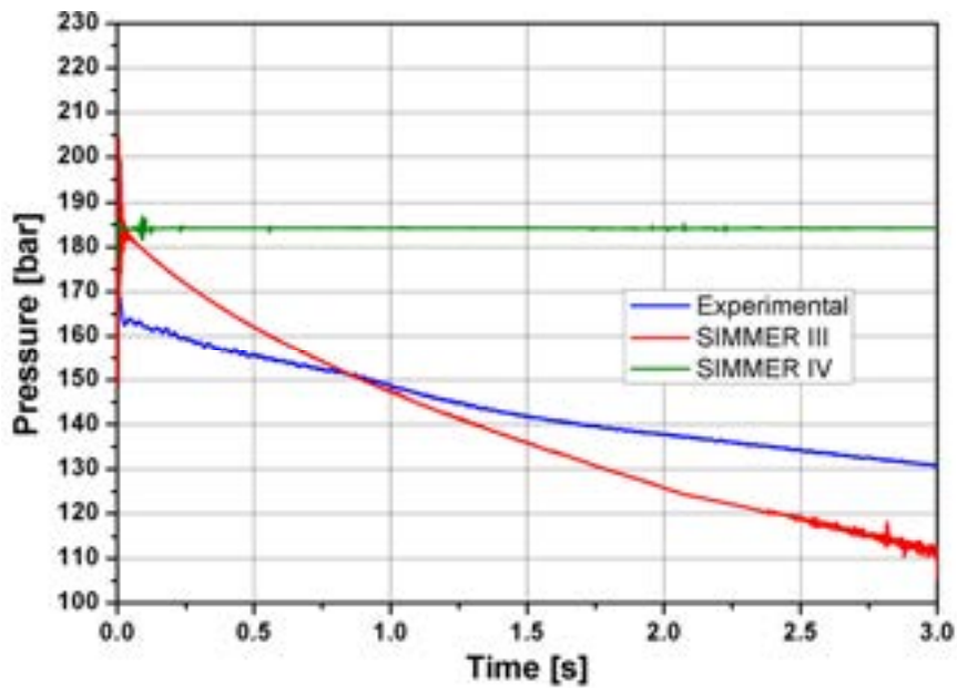
Figure 20 Pressure time trends for simulated and experimental data in PT2 location
