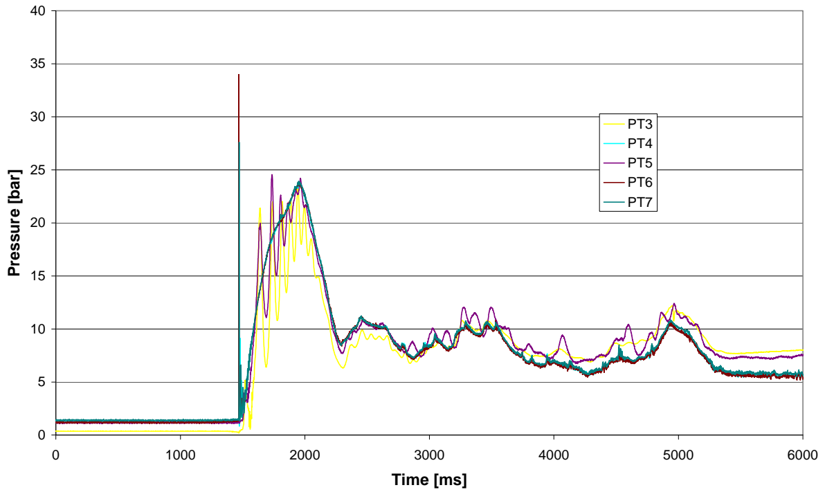
Figure 7 Experimental pressure behaviours in S1
