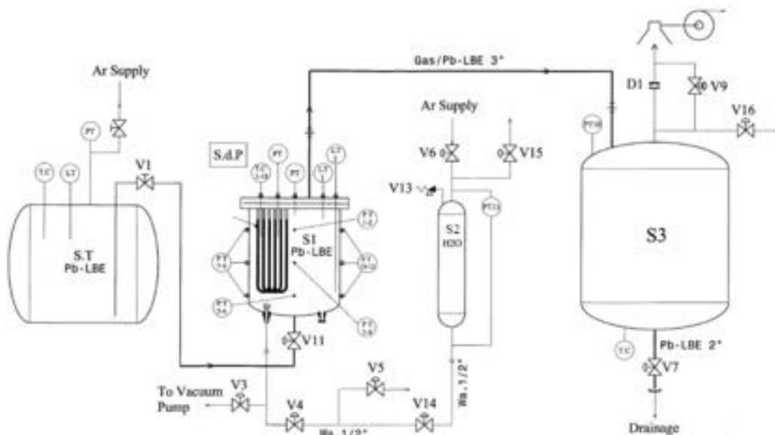
Figure 4 New LIFUS 5 layout
