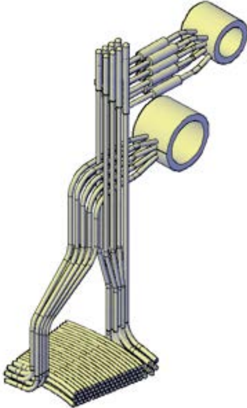
Figure 2 Scheme of the tubes-headers connection [2]
