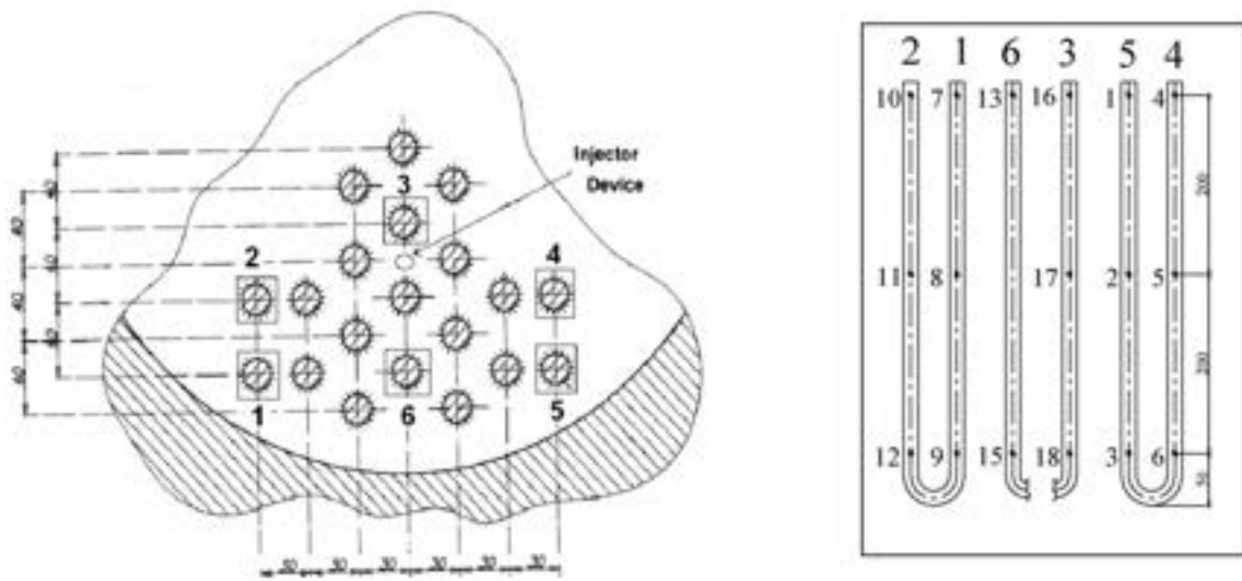
Figure 6 Thermocouples positioning
