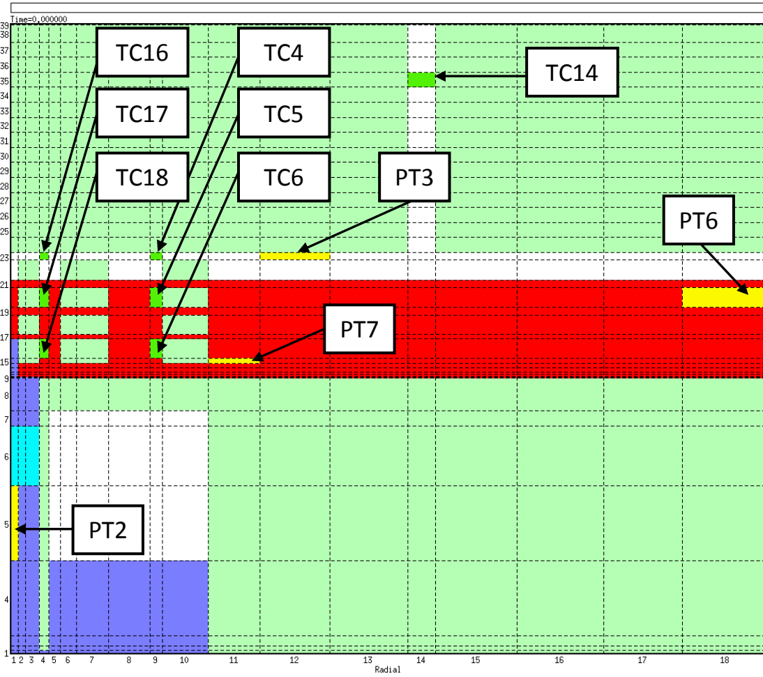
Figure 17 Two-dimensional domain with the position of temperature (green), pressure (yellow) and mass flow rate (cyan) monitoring cells
