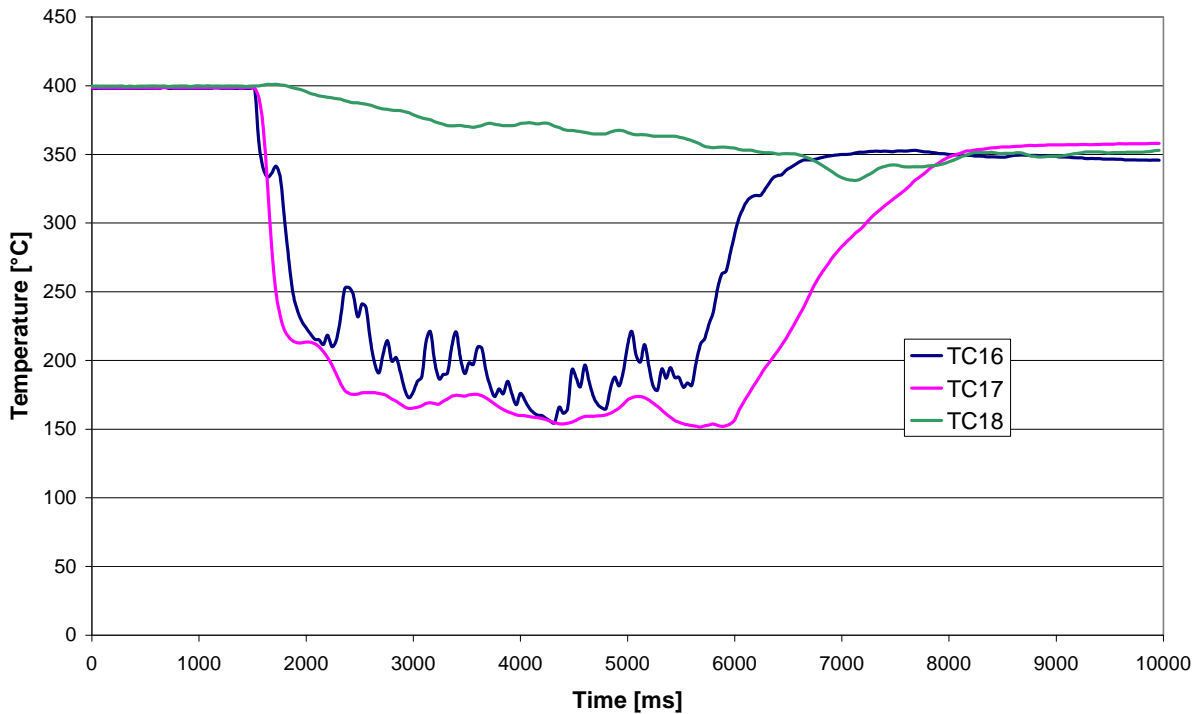
Figure 10 Experimental temperature behaviour at different heights as detected by TC16, TC17 and TC18 in the tube n.3 of the bundle (refer to Fig. 6)
