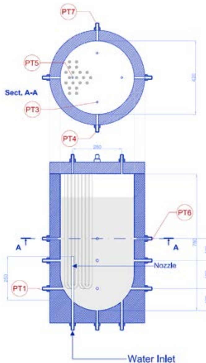
Figure 5 Pressure transducers positioning
