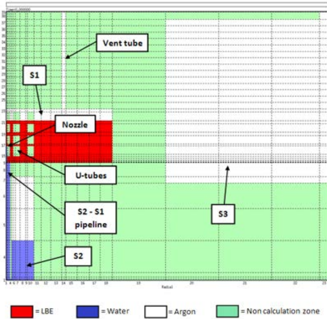
Figure 12 Two-dimensional model of LIFUS 5 used by SIMMER III code
