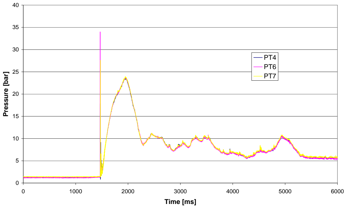
Figure 8 Experimental pressure behaviours in LBE
