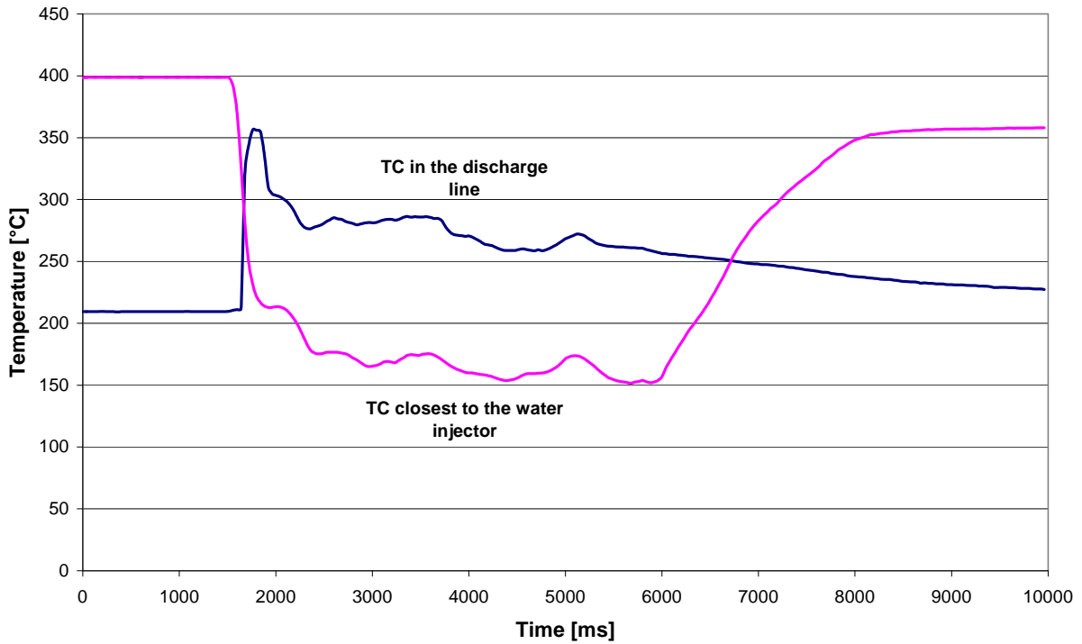
Figure 11 Experimental temperature behaviour in the discharge tube and from the TC closest to the water injector (TC17)
