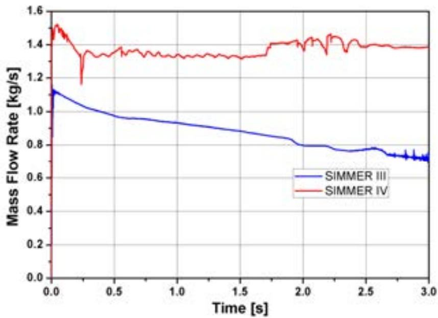
Figure 24 Mass flow rate time simulated data
