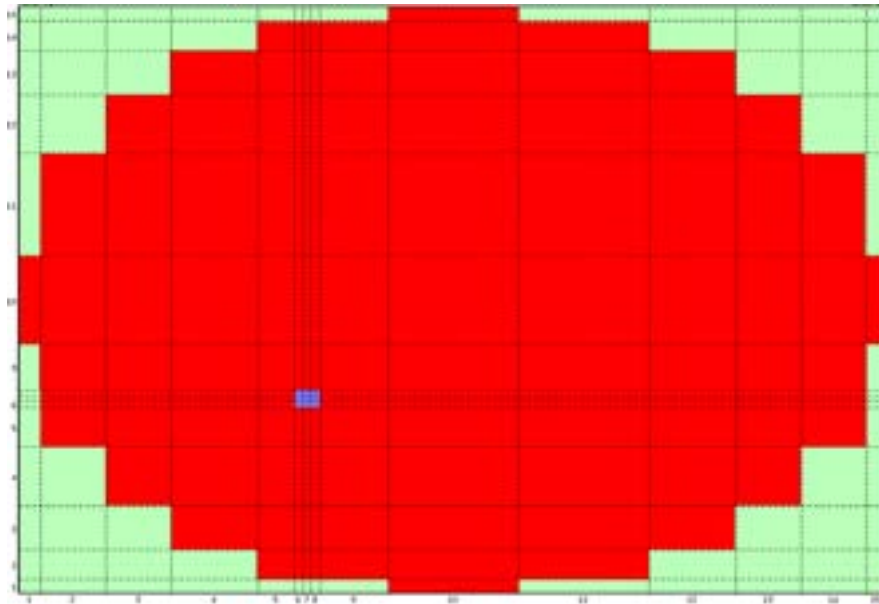
Figure 14 Three-dimensional model of LIFUS 5 facility (horizontal section of S1 vessel)
