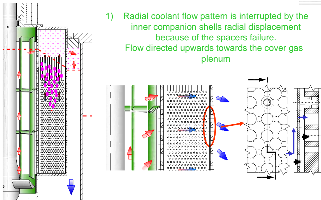
Figure 3 Upwards flow in case of SGTR accident [2]
