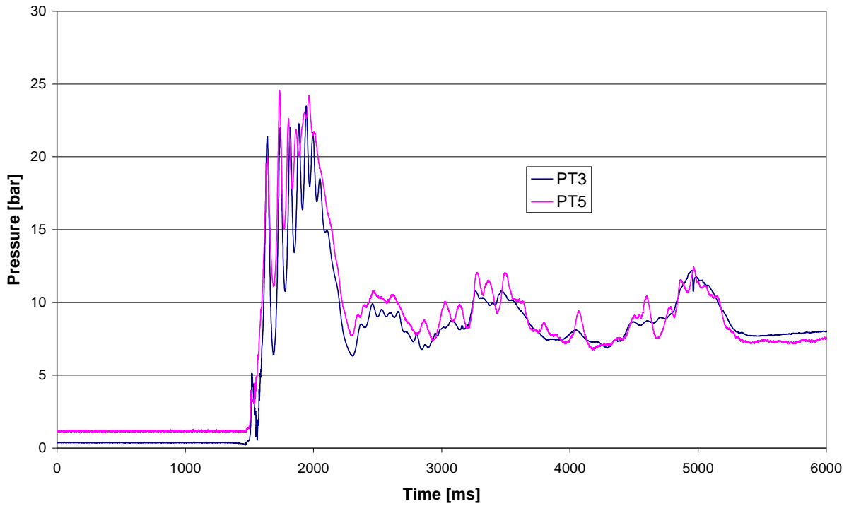
Figure 9 Experimental pressure behaviours in the cover gas
