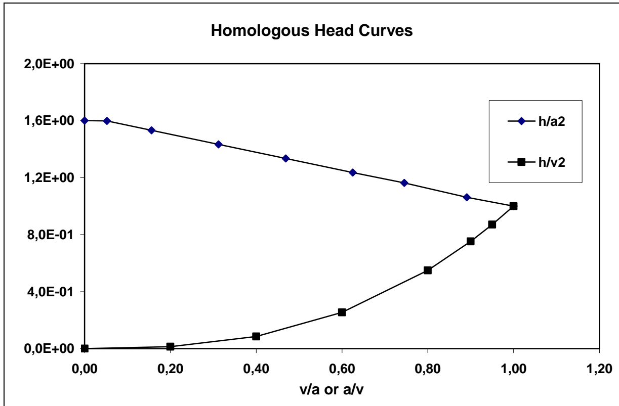
. 3.4 – RELAP Homologous Head Curve
