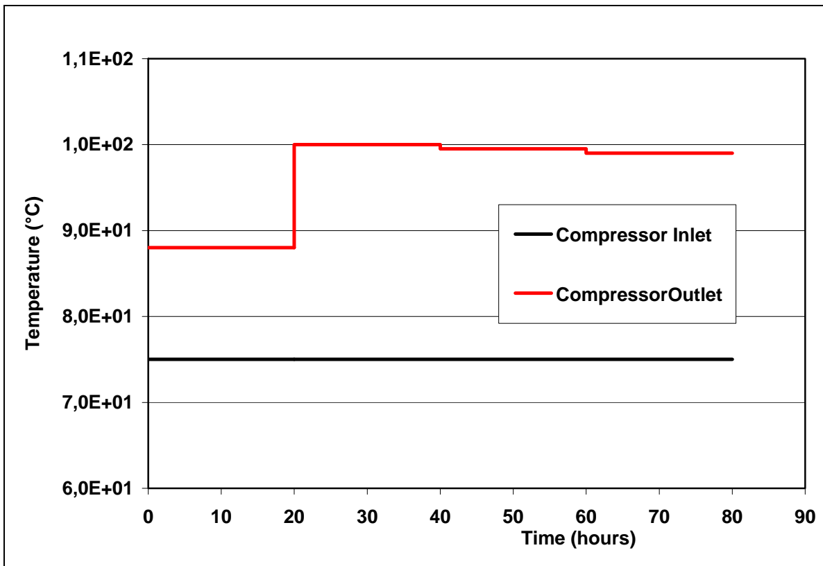
Fig. 4.5 – Inlet and Outlet Compressor Temperatures
