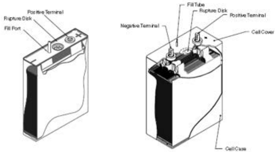
FIGURE 35.35 Schematic view showing the header and electrodes of 7 Ah (case negative) and 40 Ah (case neutral) flat plate prismatic Li-ion cells. (Courtesy of Yordney Technical Products, Inc.)
