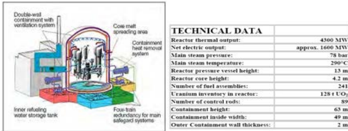
Fig. 4.3 - EPR reactor
