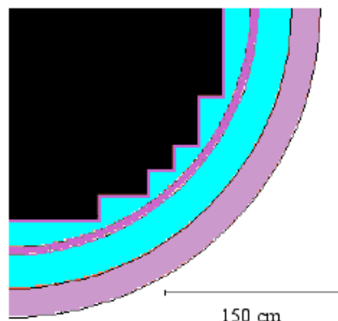
Fig. 2. 1/4 Section of Core with 1 inch Thick Baffle
