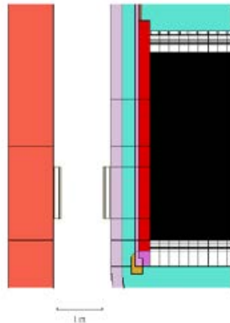
Fig. 6. Vertical Section showing 2 Possible Positions of Neutron Detectors
