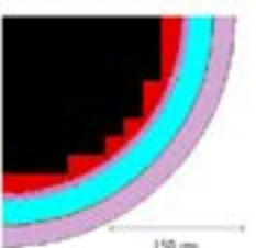
1/4 Section of Core with thick Steel Reflector
