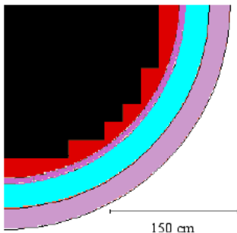
Fig. 1. 1/4 Section of Core with Thick Steel Reflector
