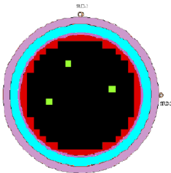
Fig. 8. Positions of the Assemblies with the Sb-Be Start-Up Sources
