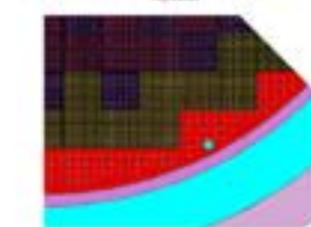
1/4 Section of Core showing the Water Lattice in the Steel Reflector
