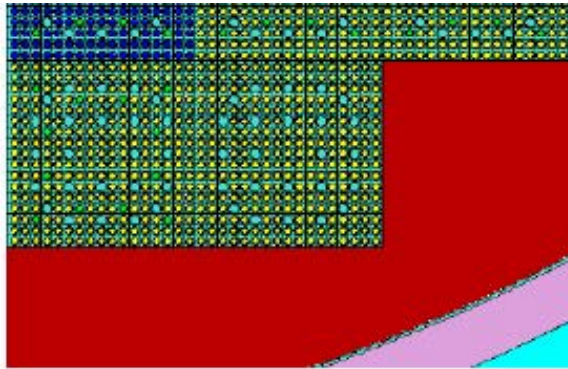
Fig. 3. Segment of Outer Core Assemblies showing Pin-by-Pin Model
