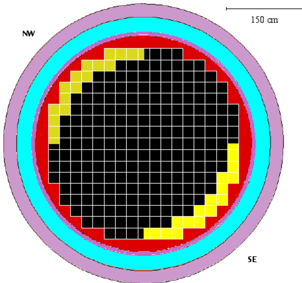
Fig. 1: Assemblies defining the change in water density that may be a factor in inducing the flux tilt.
