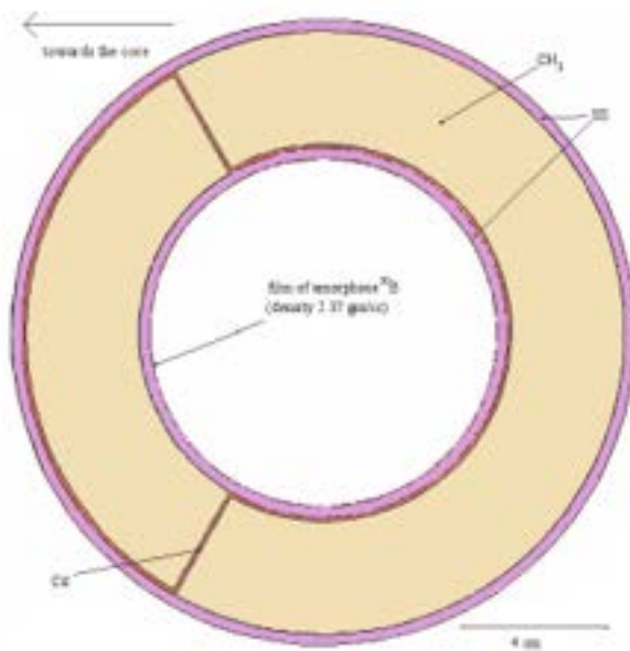
Fig. 5. Model of Ex-Core Neutron Detector (horizontal section of cylinder)
