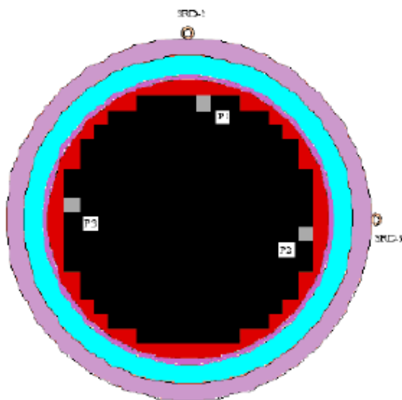
Fig. 7. Positions of the Assemblies with the ^{252}\text{Cf} Start-Up Sources
