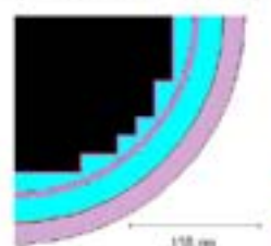
1/4 Section of Core with 1 inch thick Steel Baffle
