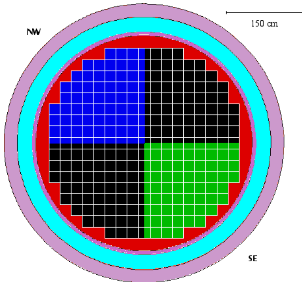
Fig. 2: Assemblies defining the flux tilt
