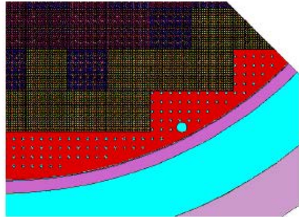
Fig. 4. 1/8 segment of the Core showing the Water Lattice in the Steel Reflector
