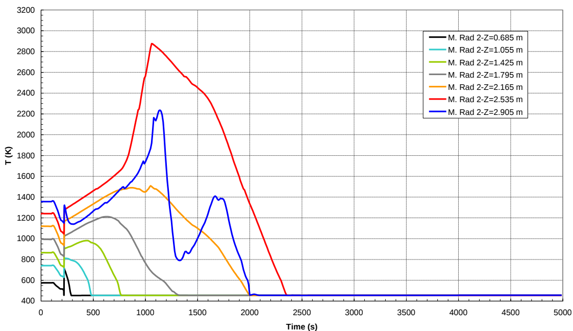
Coarse meshing. Clad-Debris bed temperatures at different axial locations. Ring 2 ( 0.81\text{m} < R < 1.35\text{m} )
