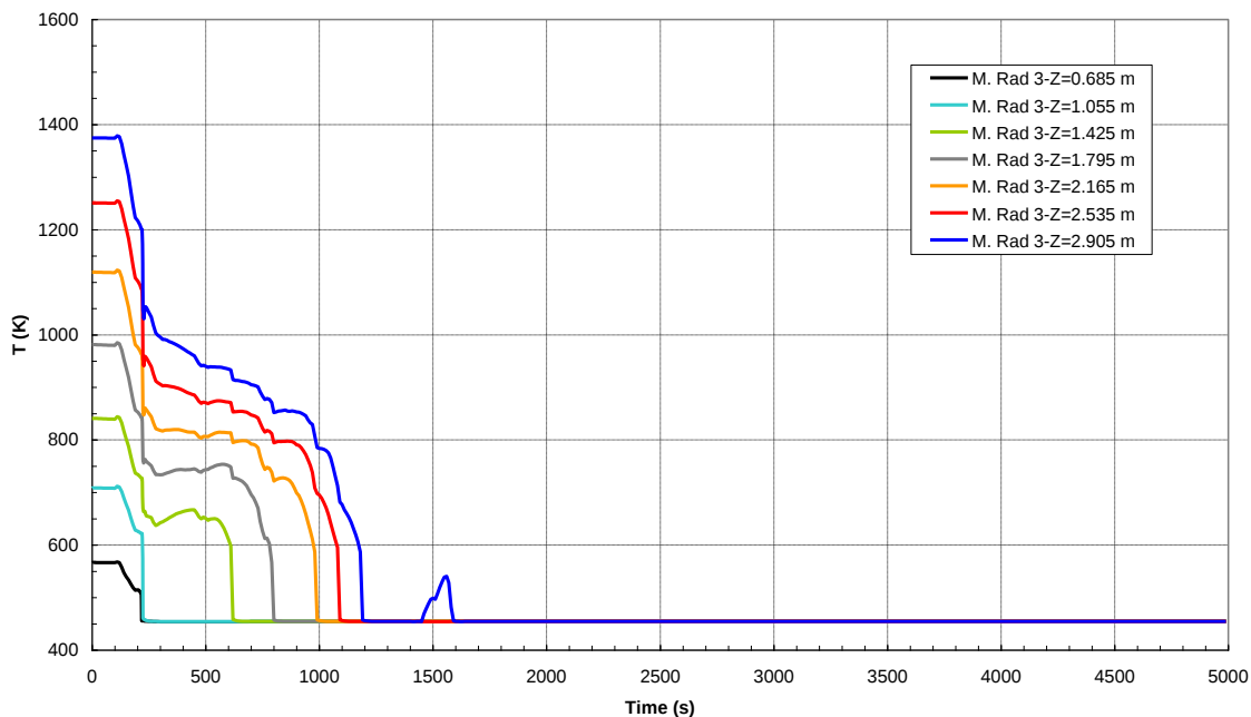
Coarse meshing. Intact fuel clad temperatures at different axial locations. Ring 3 ( 1.35\text{m} < R < 1.62\text{m} )
