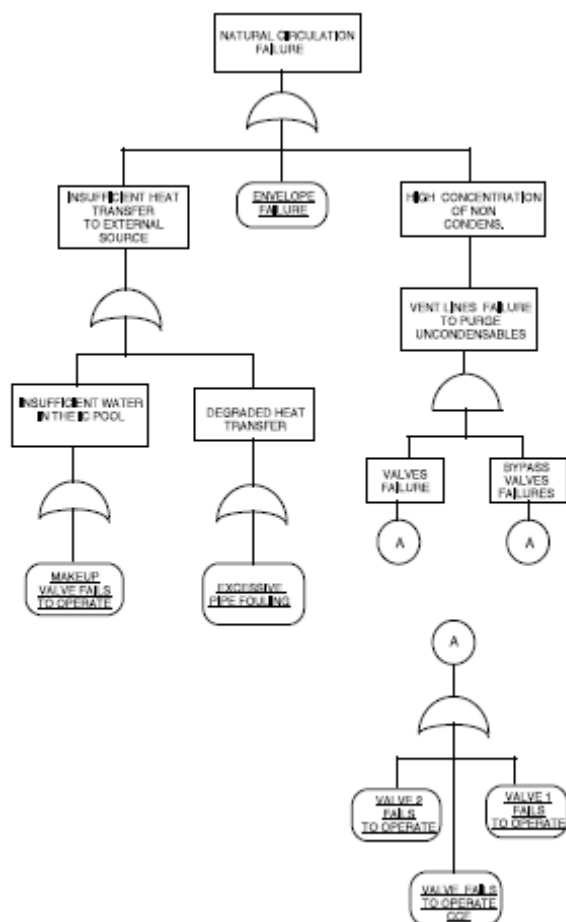
Fig. 4.8. The natural circulation fault tree.
