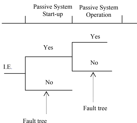
Figure 4.4 Event tree development
