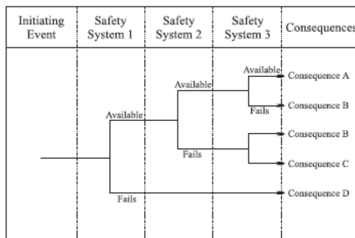
Figure 4.1. Example of an event tree
