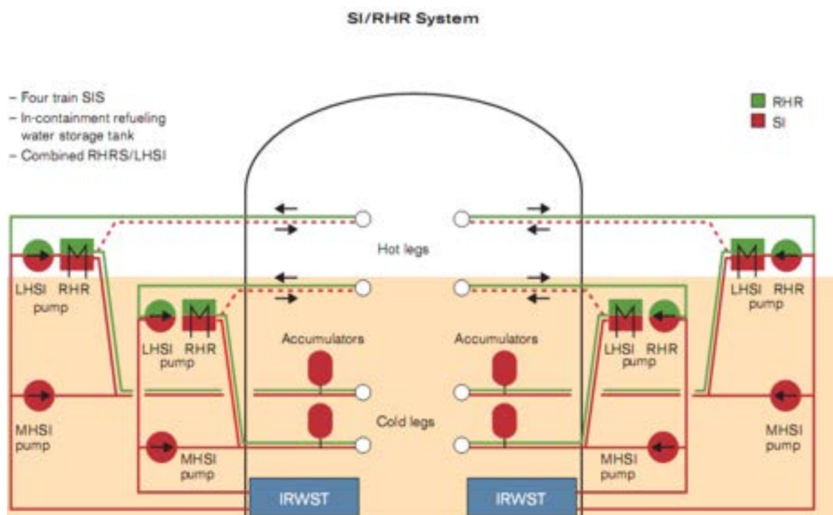
Figure 6.1 EPR's ECCS
