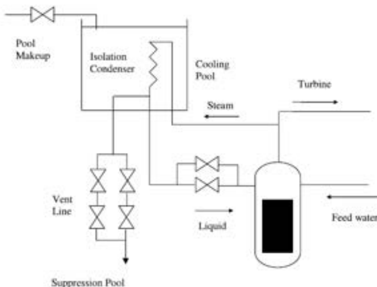
Fig.4.6 Isolation Condenser of a BWR
