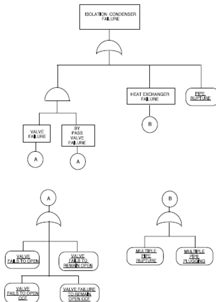
Fig 4.7 The IC fault tree.
