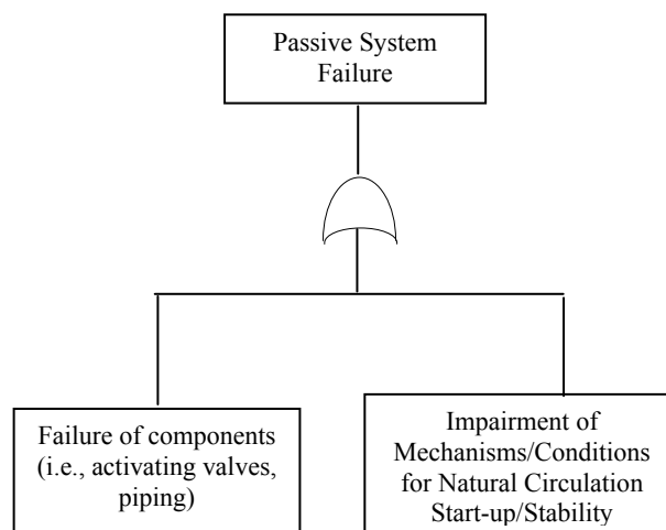
Figure 4.5 Fault tree model
