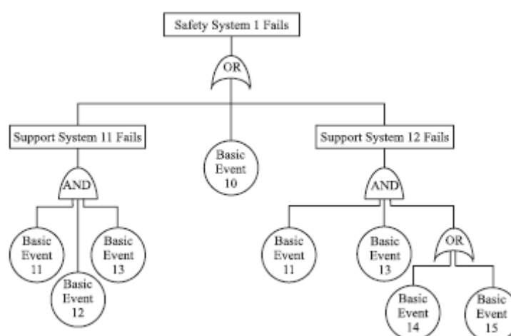
Figure 4.2 Example of a fault tree
