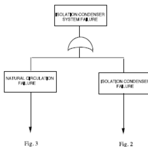
Fig. 4.9 The IC system fault tree.
