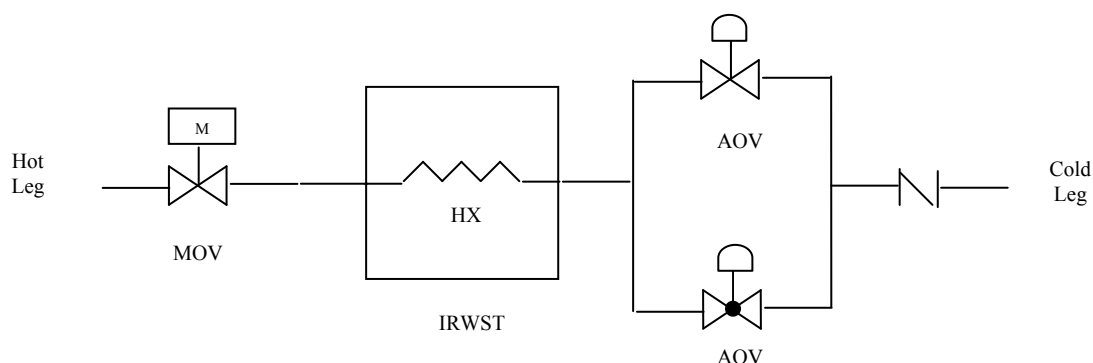
Figure 5.2 Passive system configuration
