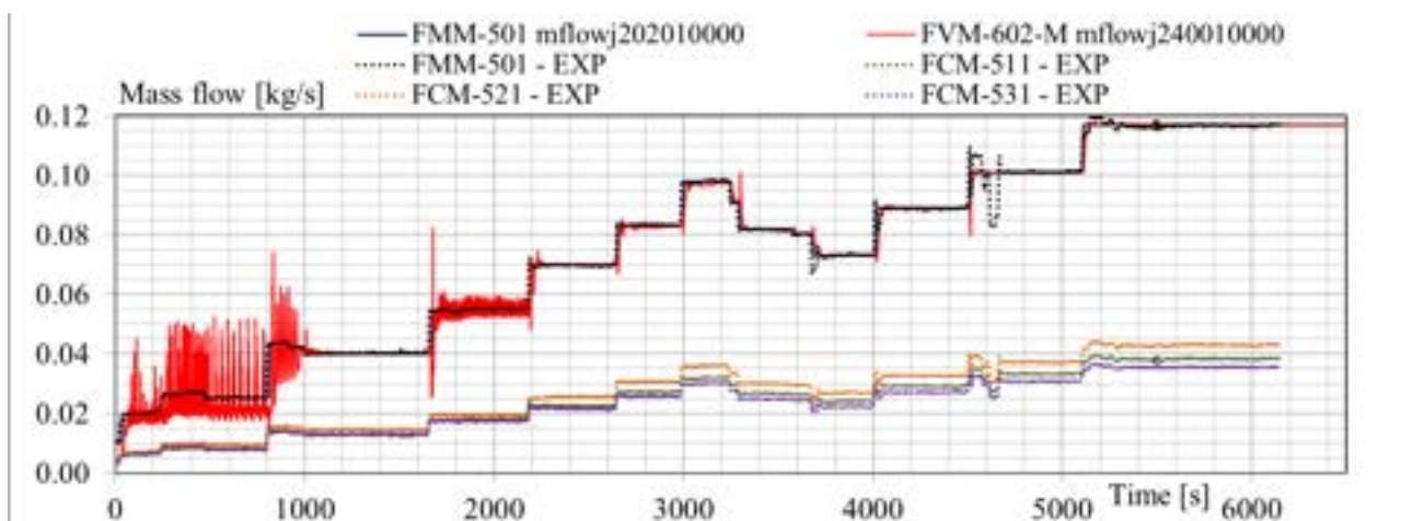
Fig. 5.10 – Test SP3, blind pretest vs. experimental results: FW total mass flow rate, FW inner/central and outer tubes (experimental trends) mass flow rate and SG outlet (calculated value) mass flow rate
