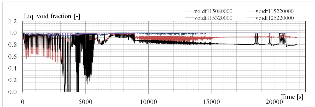
Fig. 5.7 – Test SP2, blind pretest: liquid void fraction core outlet, riser bottom, riser top, SG outlet
