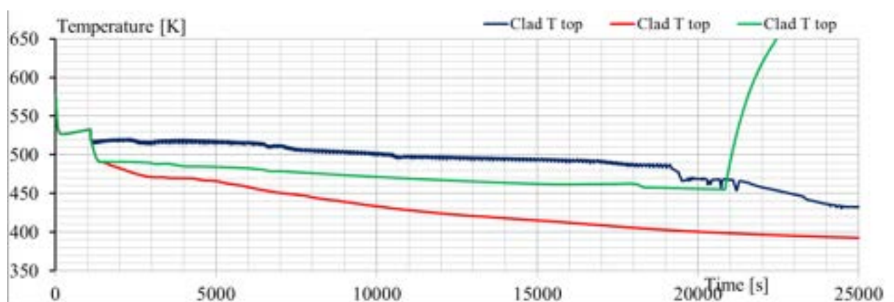
Fig. 6.19 – Sensitivity analysis RUN 1 vs. RUN 4 vs. RUN5: cladding temperature at top of the electrical core (blue “01a”; red “021a”, green “022a”)
