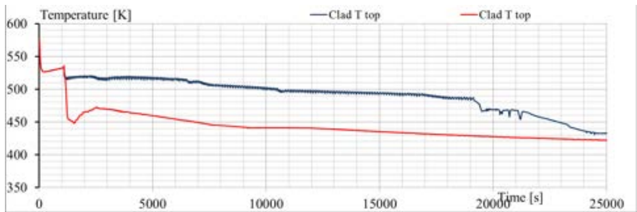
Fig. 6.26 – Sensitivity analysis RUN 1 vs. RUN 7: cladding temperature at top of the electrical core (blue “01a”; red “082a”)
