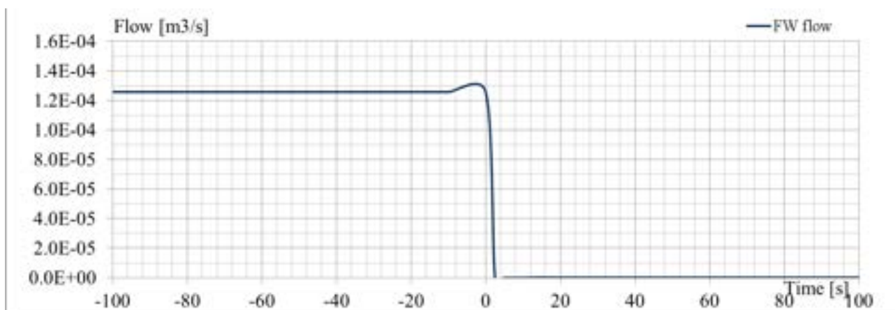
Fig. 6.1 – Simulation of SBO transient: main FW flow
