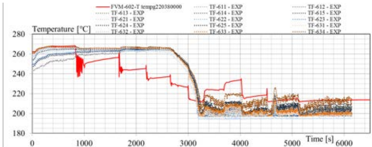
Fig. 5.12 – Test SP3, blind pretest vs. experimental results: calculated steam temperature at SG outlet and SG tubes outlet fluid temperatures
