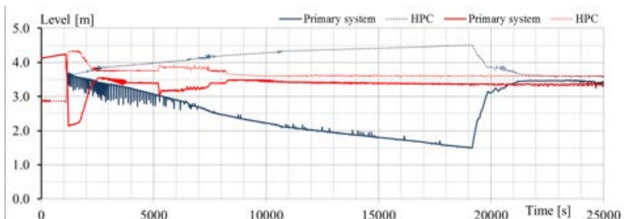
Fig. 6.21 – Sensitivity analysis RUN 1 vs. RUN 6: primary and HPC levels (blue “01a”; red “03a”)
