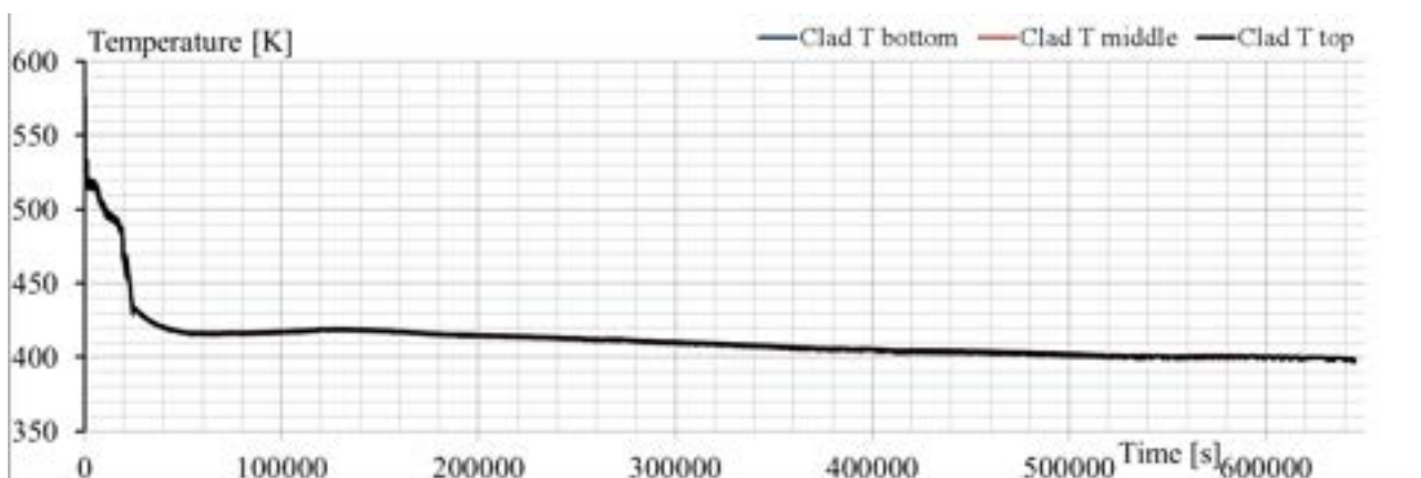
Fig. 6.3 – Simulation of SBO transient: cladding temperature
