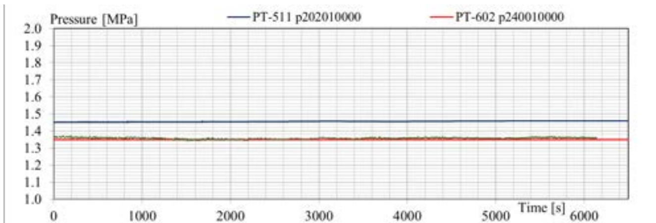
Fig. 5.9 – Test SP3, blind pretest vs. experimental results: steam generator inlet (only experimental) and outlet pressures
