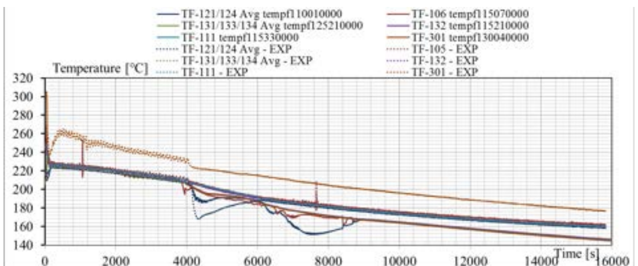
Fig. 5.3 – Test SP2, blind pretest vs. experimental results: primary system coolant temperatures, liquid phase (lower plenum, core outlet, SG outlet, riser, riser outlet and PRZ)
