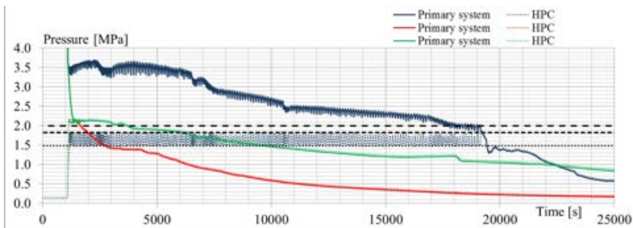
Fig. 6.16 – Sensitivity analysis RUN 1 vs. RUN 4 vs. RUN5: primary and HPC pressures (blue “01a”; red “021a”, green “022a”)
