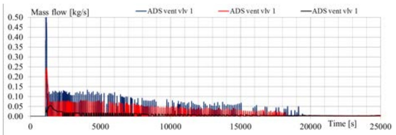
Fig. 6.12 – Sensitivity analysis RUN 1 vs. RUN 2 vs. RUN3: ADS vent valve 1 mass flow rate (blue “01a”; red “01a_vlv05”, black “01a_vlv01”)
