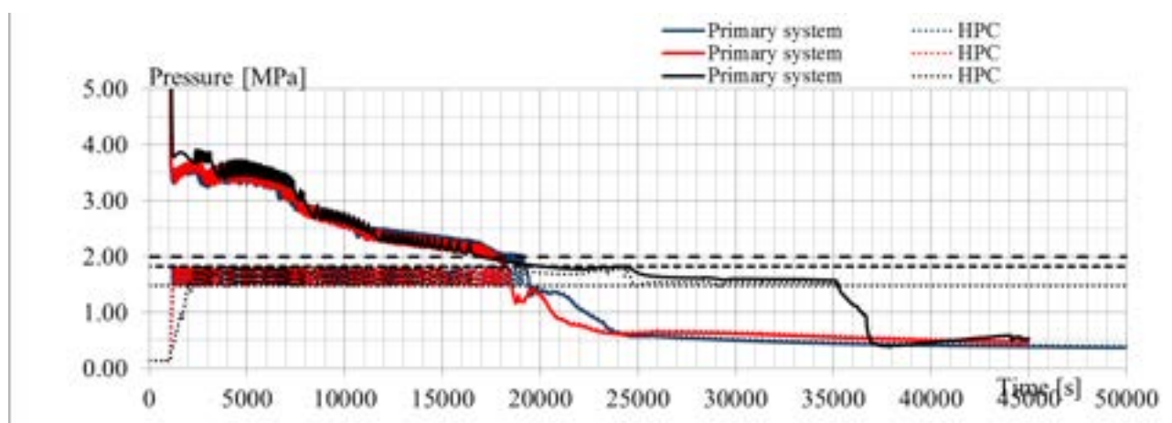
Fig. 6.13 – Sensitivity analysis RUN 1 vs. RUN 2 vs. RUN3: primary system and HPC pressures (blue “01a”; red “01a_vlv05”, black “01a_vlv01”)
