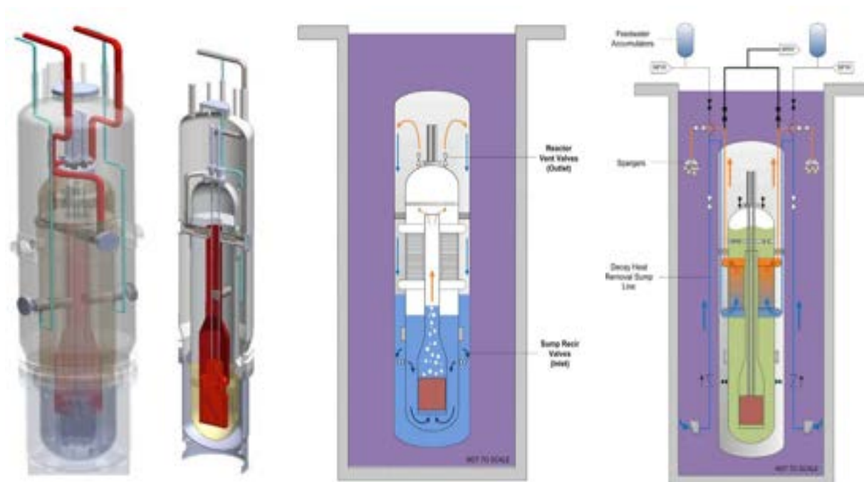
(a) High Pressure Containment Vessel and Reactor Pressure Vessel
