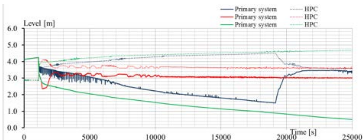
Fig. 6.17 – Sensitivity analysis RUN 1 vs. RUN 4 vs. RUN5: primary and HPC levels (blue “01a”; red “021a”, green “022a”)
