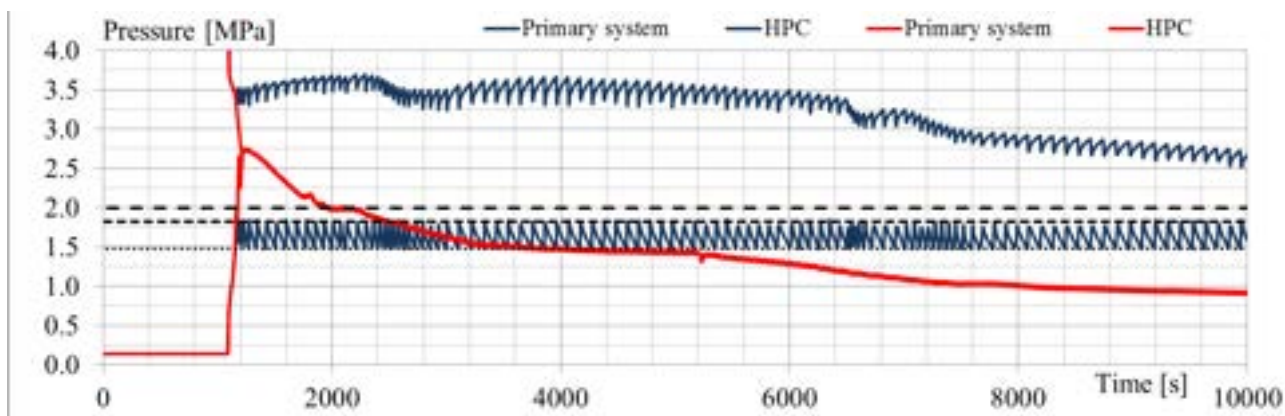
Fig. 6.20 – Sensitivity analysis RUN 1 vs. RUN 6: primary and HPC pressures (blue “01a”; red “03a”)
