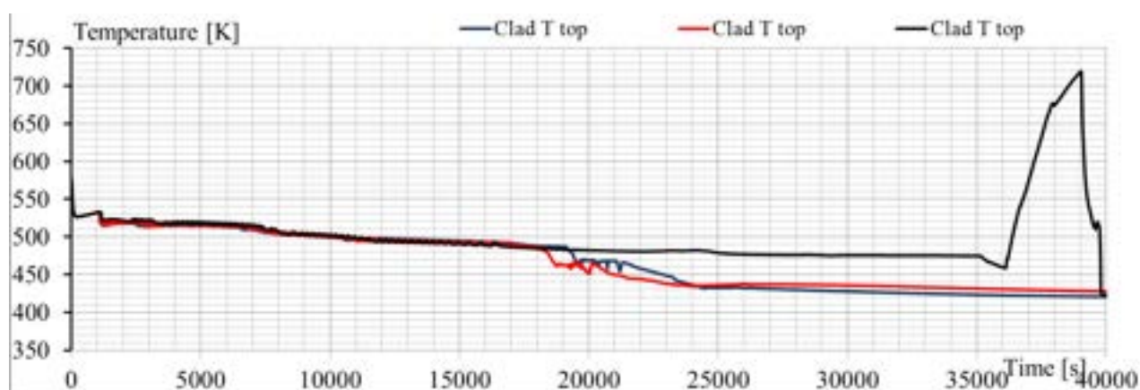
Fig. 6.15 – Sensitivity analysis RUN 1 vs. RUN 2 vs. RUN3: cladding temperature at top of the electrical core (blue “01a”; red “01a_vlv05”, black “01a_vlv01”)
