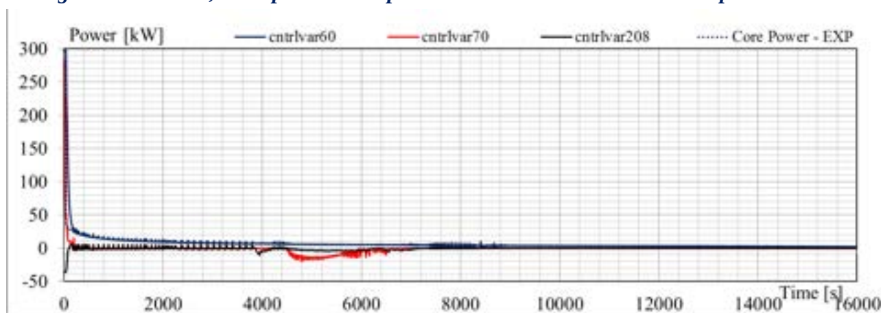
Fig. 5.6 – Test SP2, blind pretest vs. experimental results: core power (transfer to fluid for the code result and electrical power for the experimental trend) – cntrlvar60, SG power – cntrlvar70, power exchanged across the chimney – cntrlvar208.
