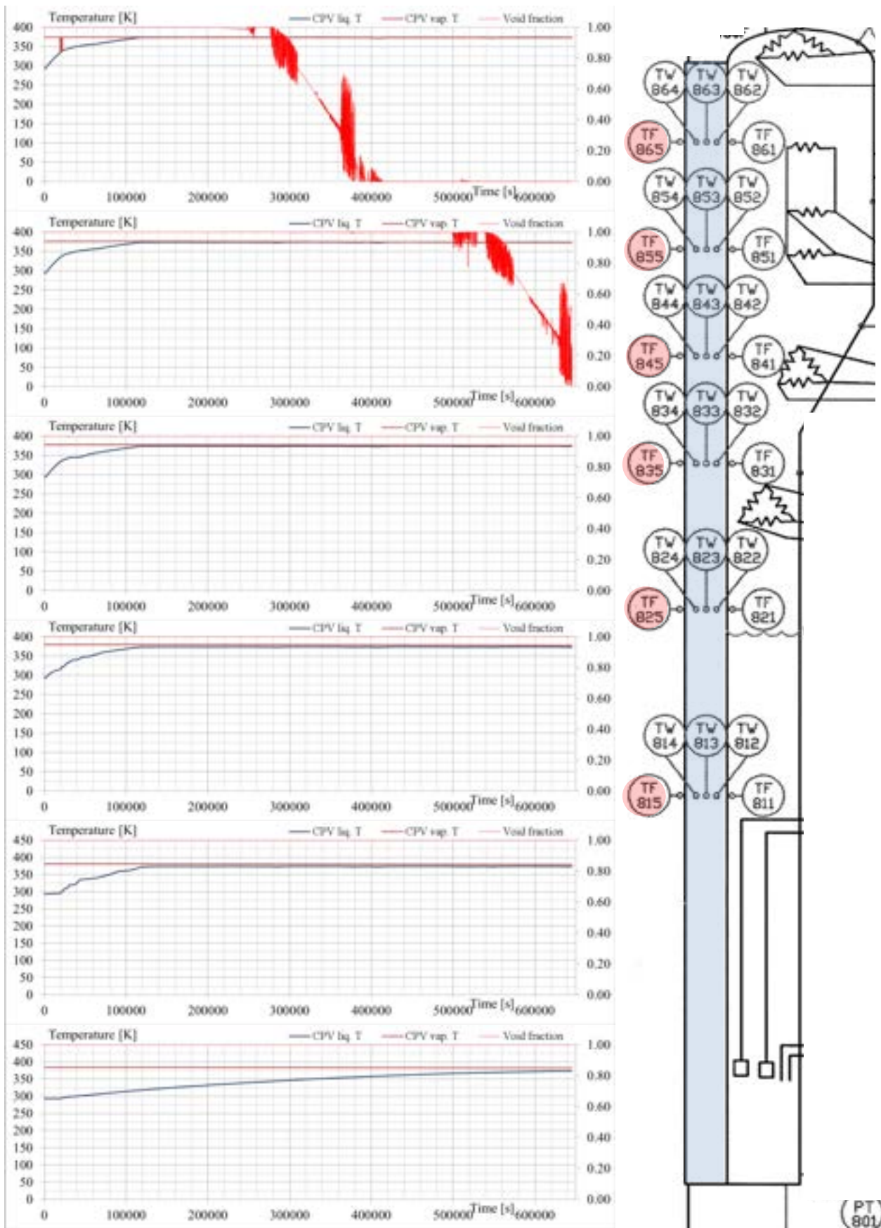
Fig. 6.10 – Simulation of SBO transient: CPV coolant temperatures
