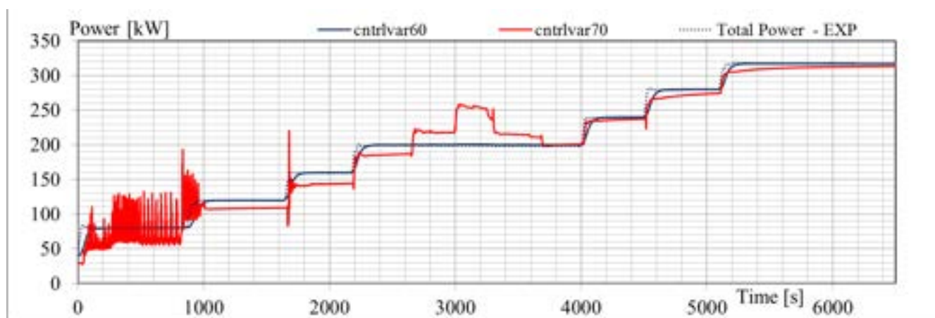
Fig. 5.15 – Test SP3, blind pretest vs. experimental results: calculated core power - cntrlvar60 (transfer to fluid), calculated SG power cntrlvar70, experimental electrical power
