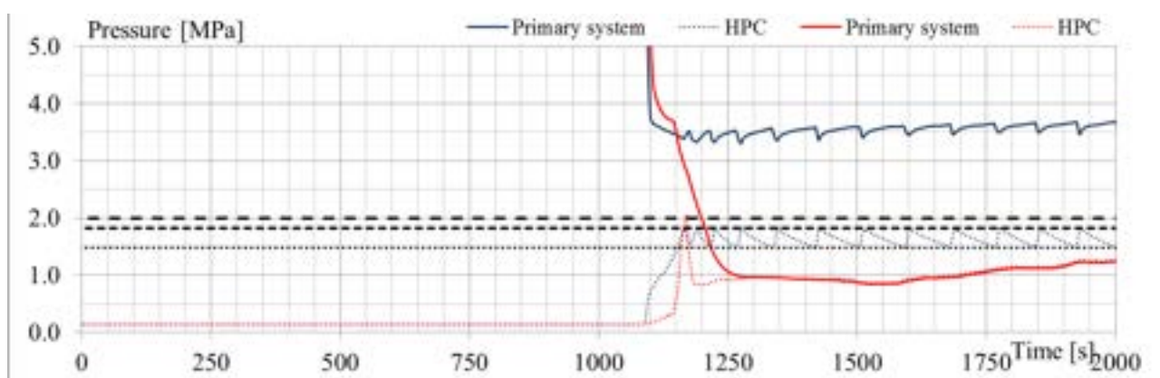
Fig. 6.24 – Sensitivity analysis RUN 1 vs. RUN 7: primary and HPC pressures (blue “01a”; red “082a”)
