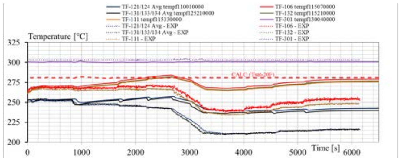
Fig. 5.13 – Test SP3, blind pretest vs. experimental results: primary system coolant temperature, liquid phase (lower plenum, core outlet, SG outlet, riser, riser outlet and PRZ)
