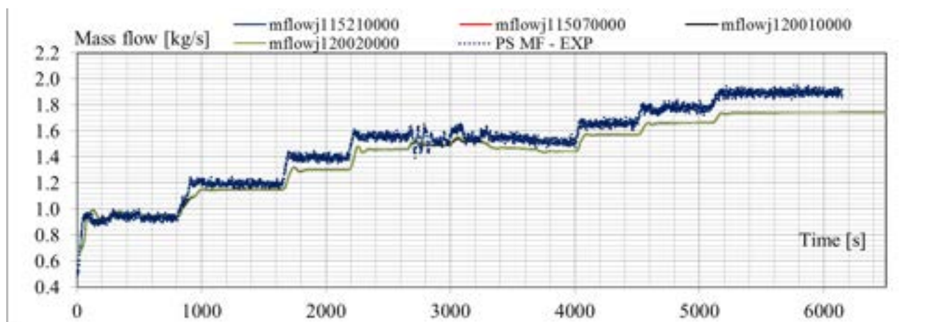
Fig. 5.14 – Test SP3, blind pretest vs. experimental results: primary system mass flow rate (core inlet, outlet chimney outlet SG inlet)
