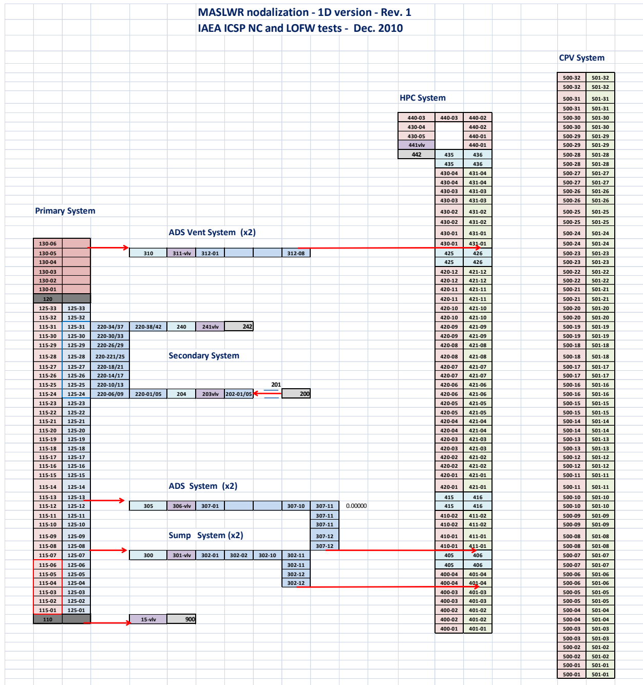
Fig. 4.1 – ENEA nodalization: overall sketch
