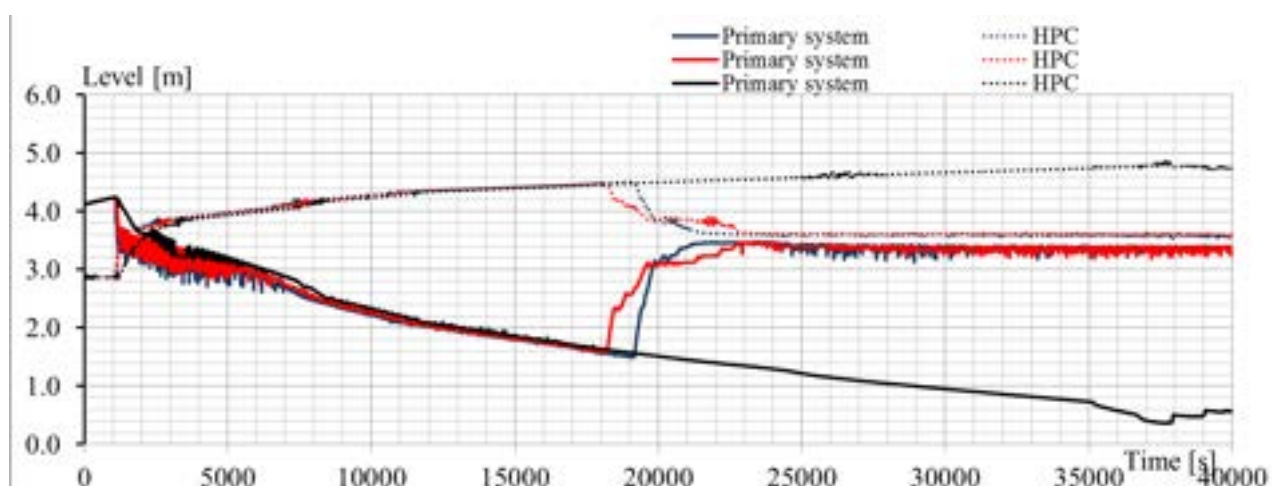
Fig. 6.14 – Sensitivity analysis RUN 1 vs. RUN 2 vs. RUN3: primary system and HPC levels (blue “01a”; red “01a_vlv05”, black “01a_vlv01”)
