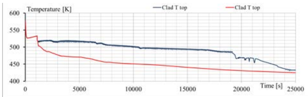
Fig. 6.22 – Sensitivity analysis RUN 1 vs. RUN 6: cladding temperature at top of the electrical core (blue “01a”; red “03a”)
