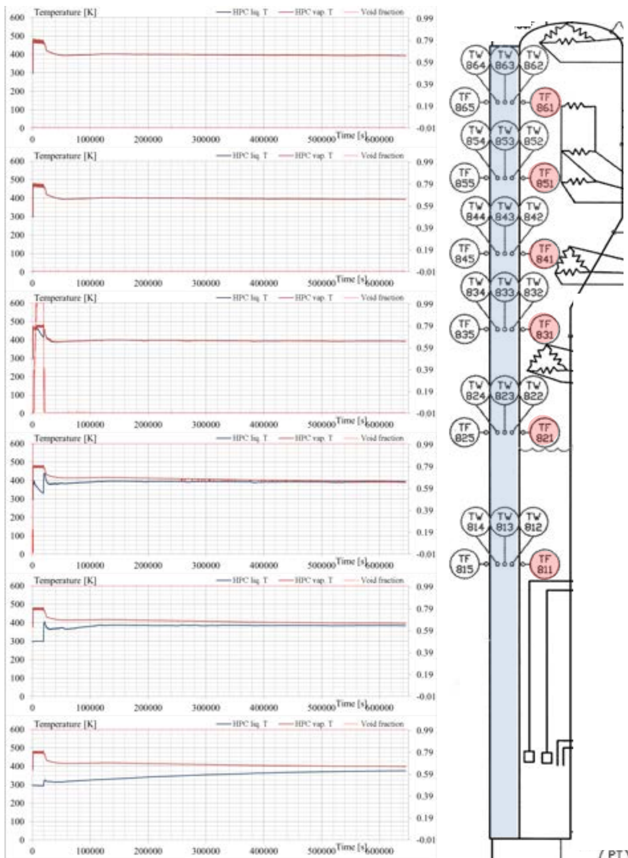
Fig. 6.9 – Simulation of SBO transient: HPC coolant temperatures
