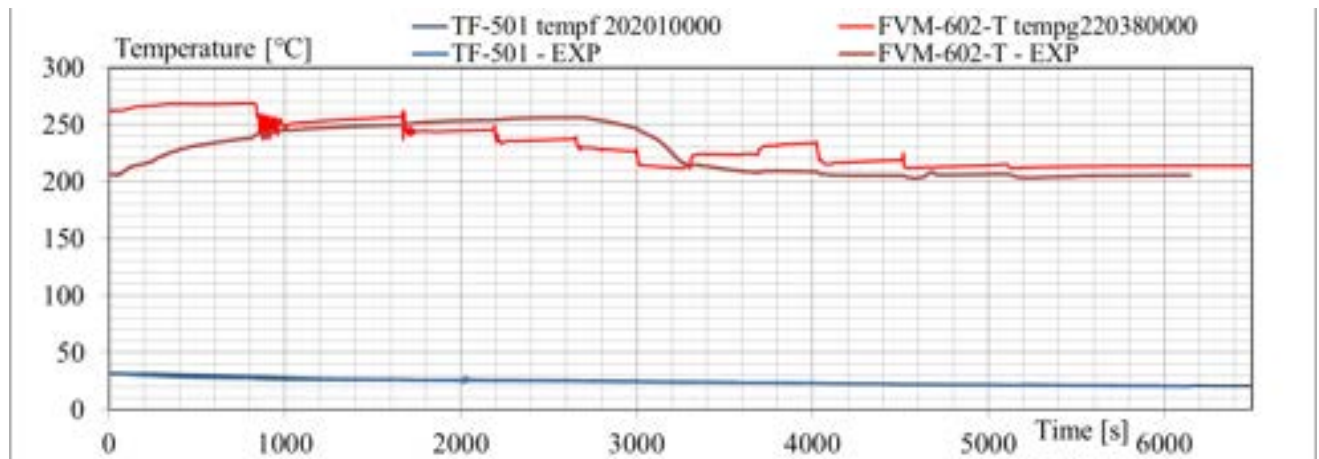
Fig. 5.11 – Test SP3, blind pretest vs. experimental results: FW and steam line temperatures
