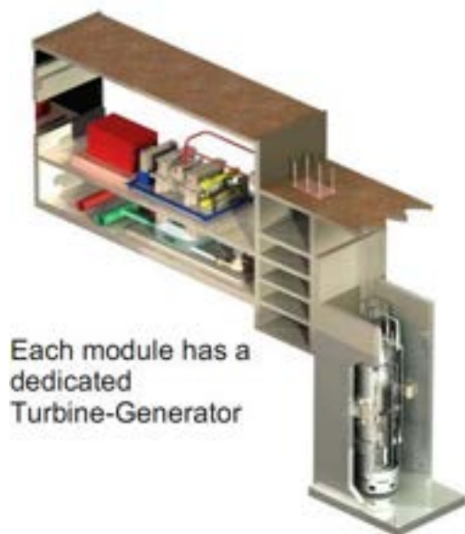
(a) Schematic of the MASLWR exterior cooling pool and turbine generator set
