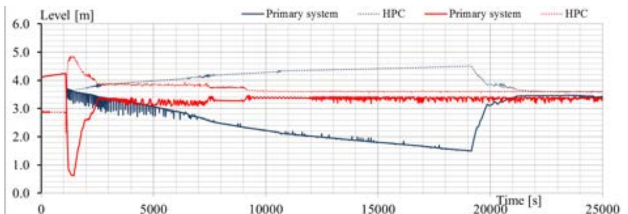
Fig. 6.25 – Sensitivity analysis RUN 1 vs. RUN 7: primary and HPC levels (blue “01a”; red “082a”)
