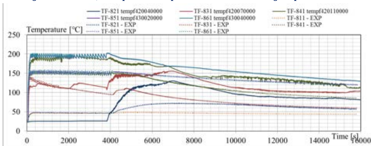
Fig. 5.5 – Test SP2, blind pretest vs. experimental results: HPC coolant temperatures
