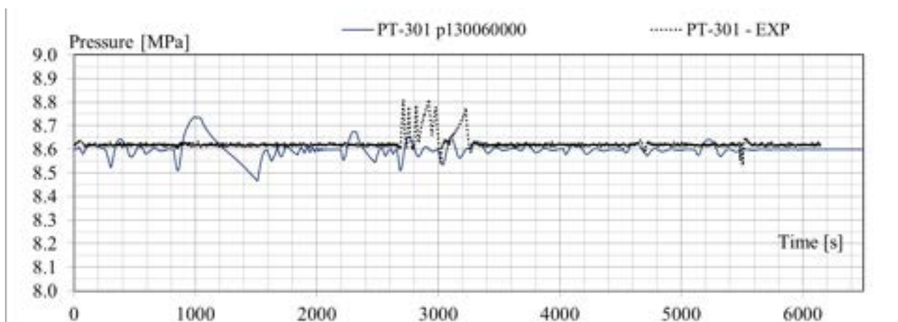
Fig. 5.8 – Test SP3, blind pretest vs. experimental results: PS pressure
