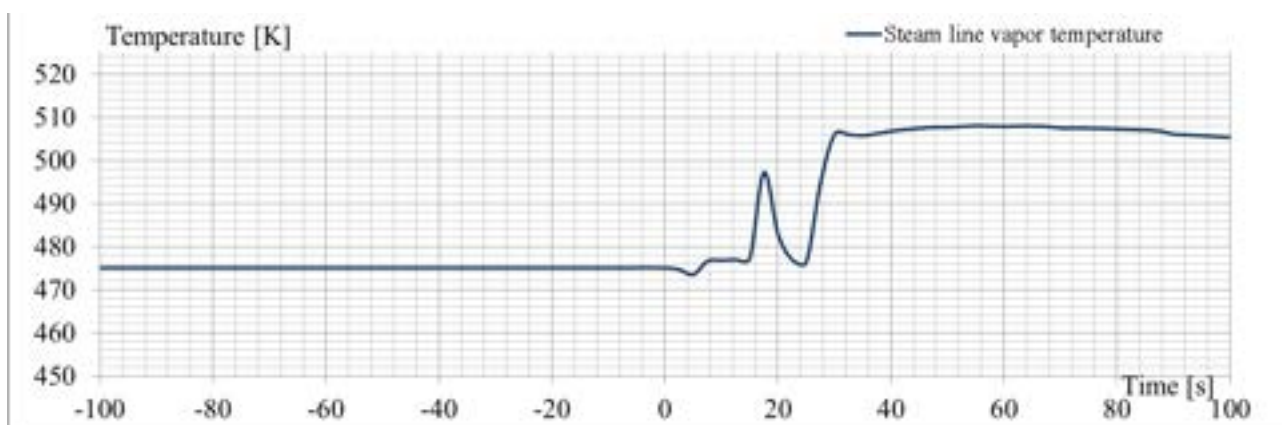
Fig. 6.2 – Simulation of SBO transient: steam line coolant temperature
