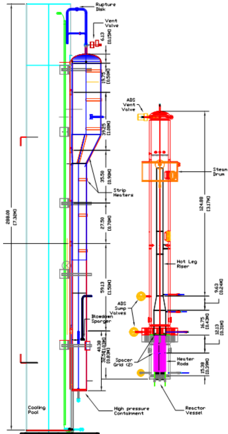
Fig. 3.3 – OSU MASLWR Test Facility: overall schematization
