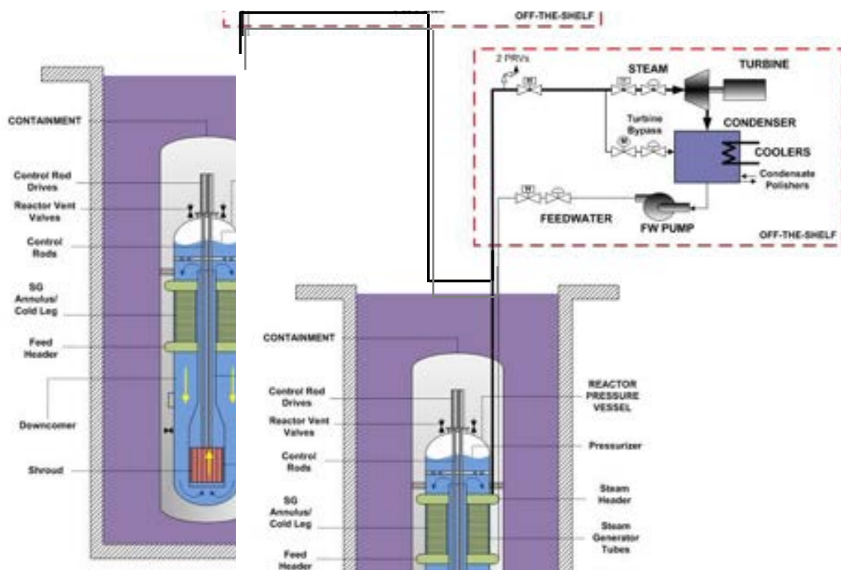
Fig. 2.1 – MASLWR layout
