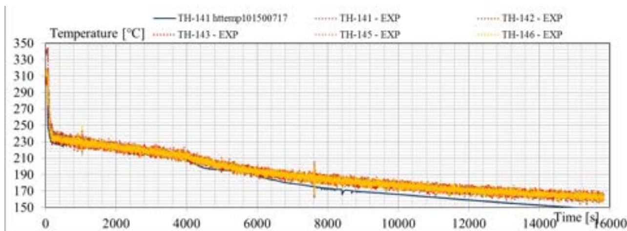
Fig. 5.4 – Test SP2, blind pretest vs. experimental results: cladding temperatures
