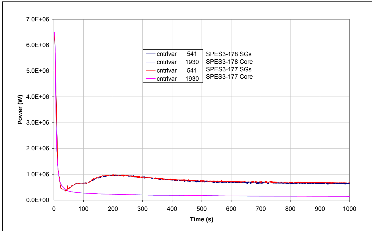
Fig.8. 13 – SPES3-178 and SPES3-177 Core and SG total power (window)
