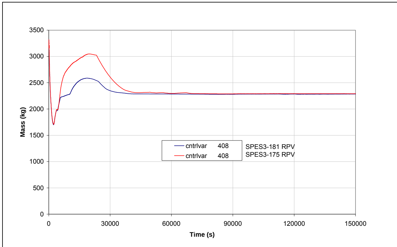
Fig.7. 33 - SPES3-181 and SPES3-175 RPV mass
