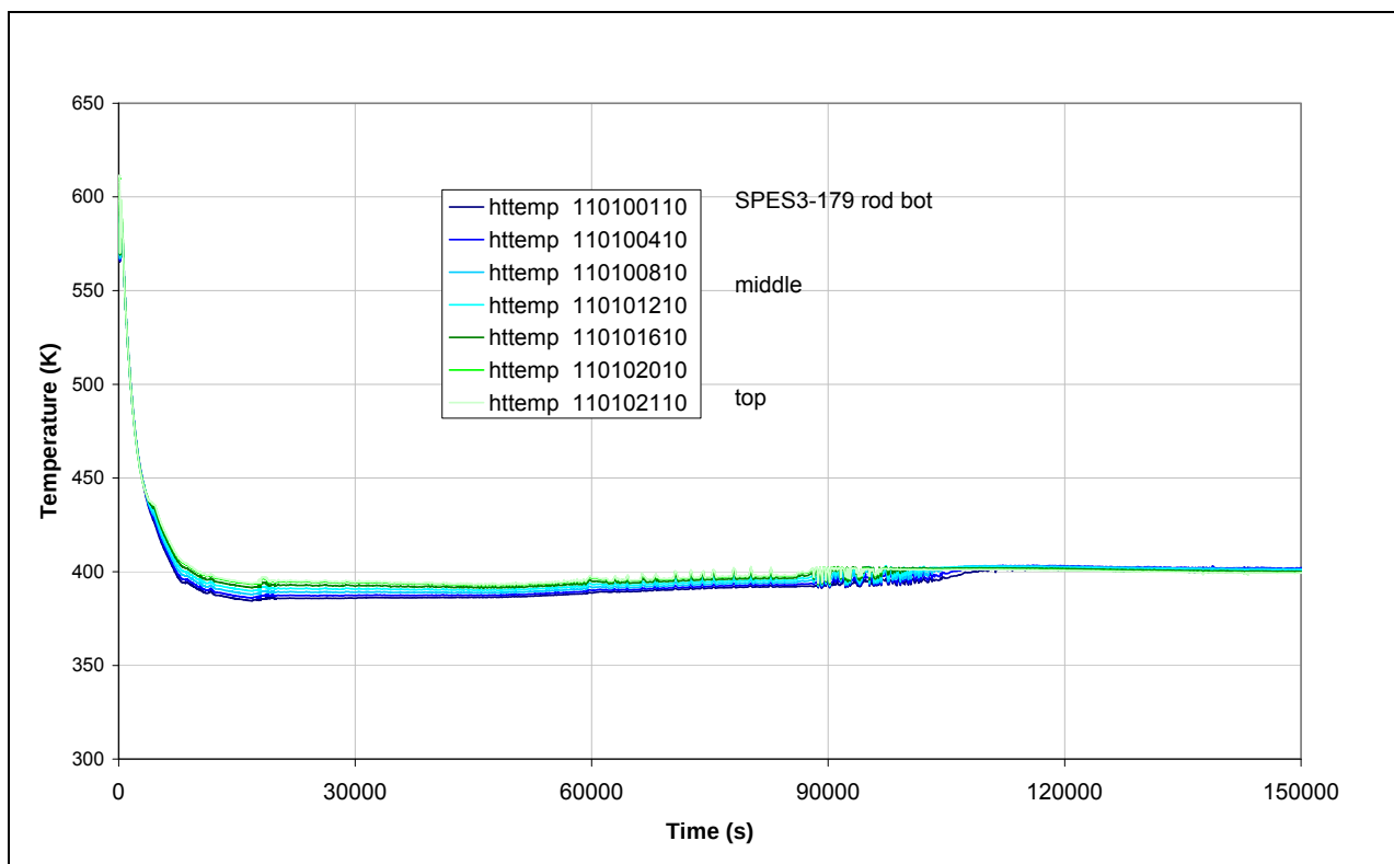
Fig.5. 60 - SPES3-179 Core heater rod surface temperature –normal rod
