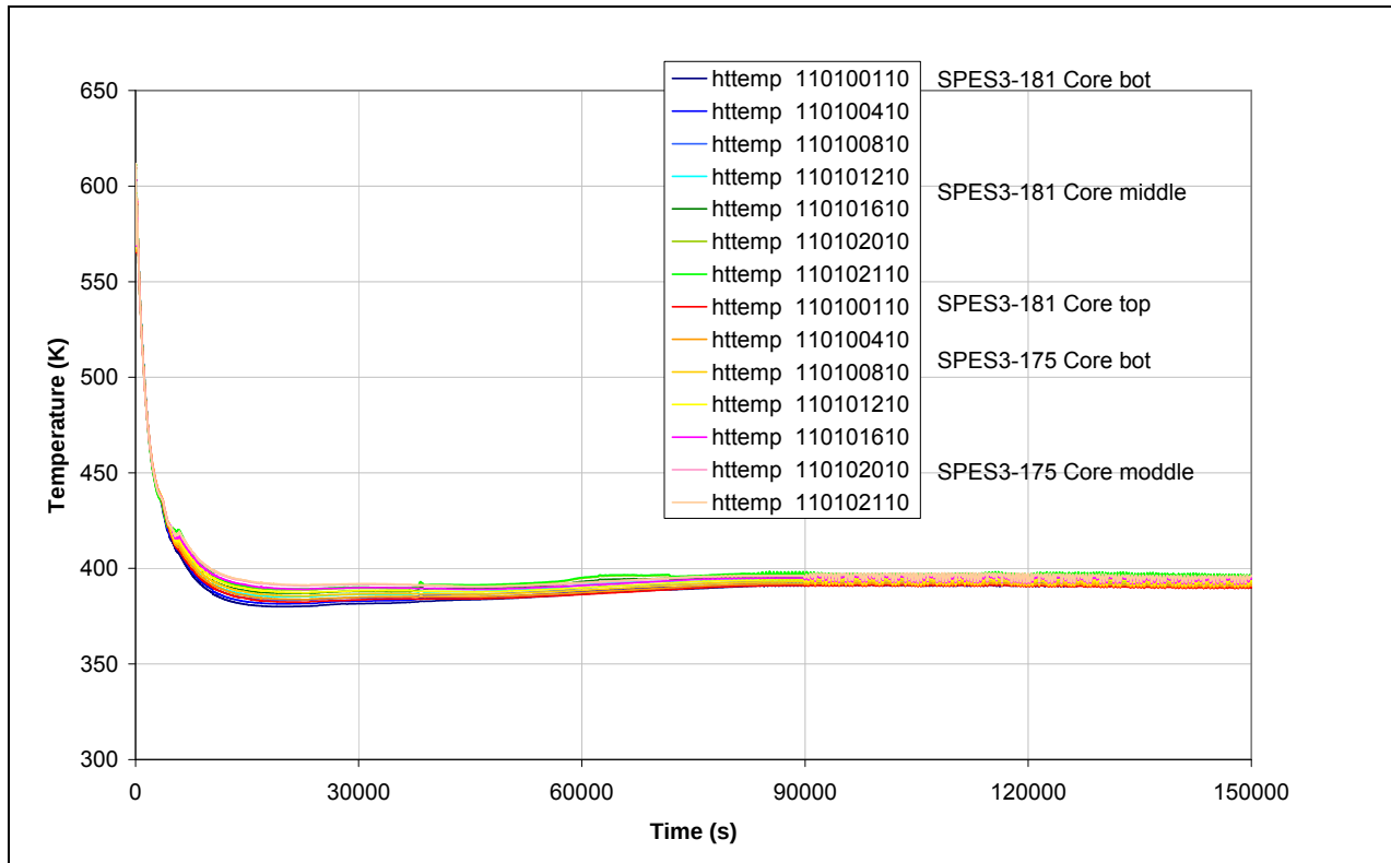
Fig.7. 43 - SPES3-181 and SPES3-175 Core heater rod surface temperature –normal rod
