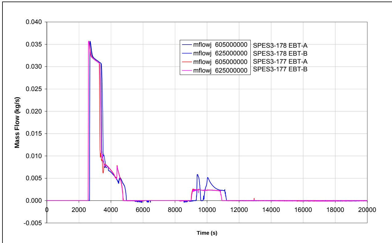
Fig.8. 37 – SPES3-178 and SPES3-177 EBT injection mass flow (window)
