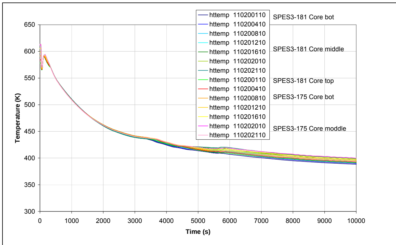
Fig.7. 44 - SPES3-181 and SPES3-175 Core heater rod surface temperature –hot rod (window)
