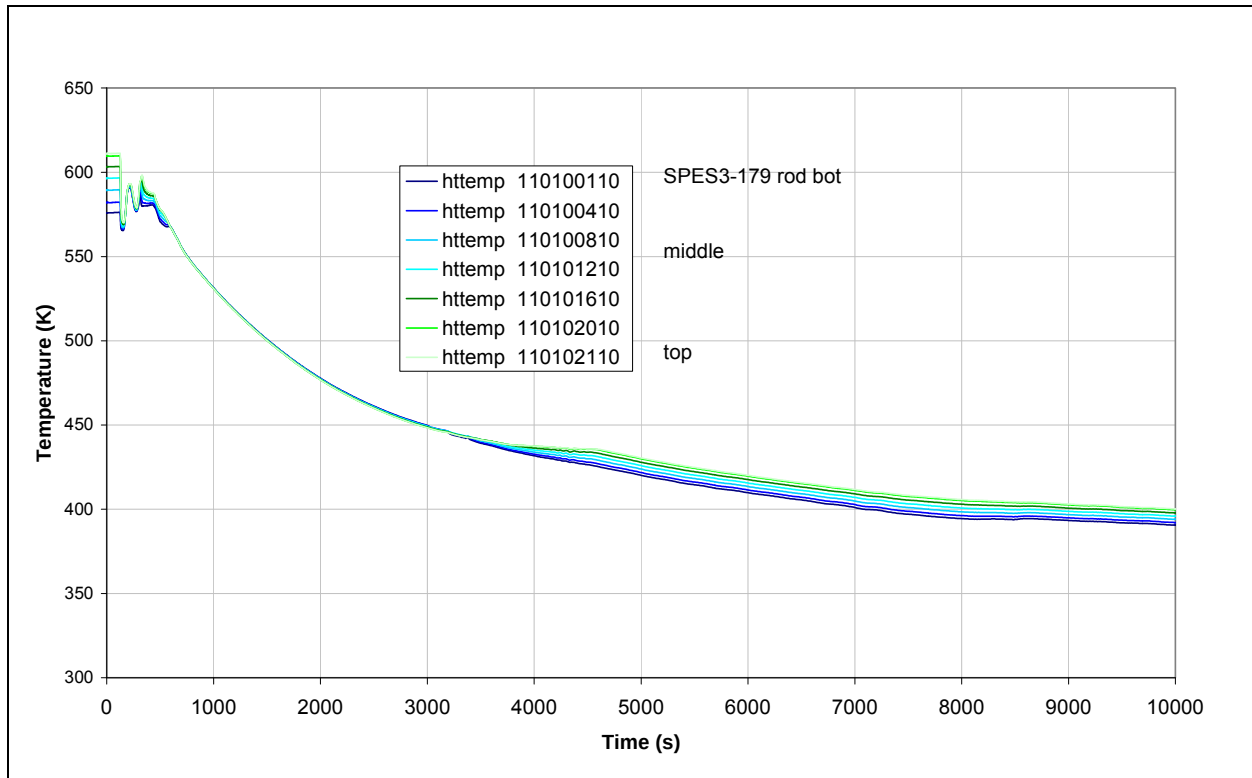
Fig.5. 59 - SPES3-179 Core heater rod surface temperature –normal rod (window)
