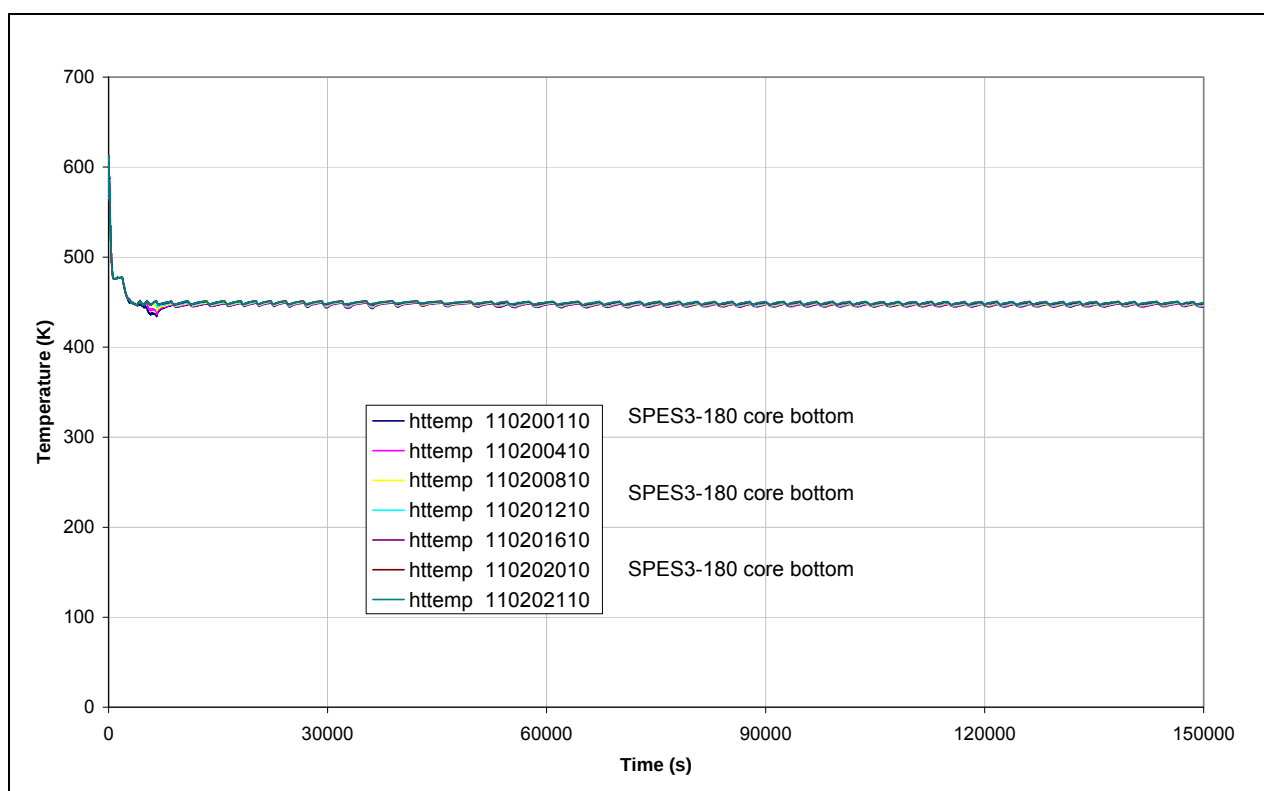
Fig.4.50 – SPES3-180 Core heater rod clad surface temperatures (hot rods)
