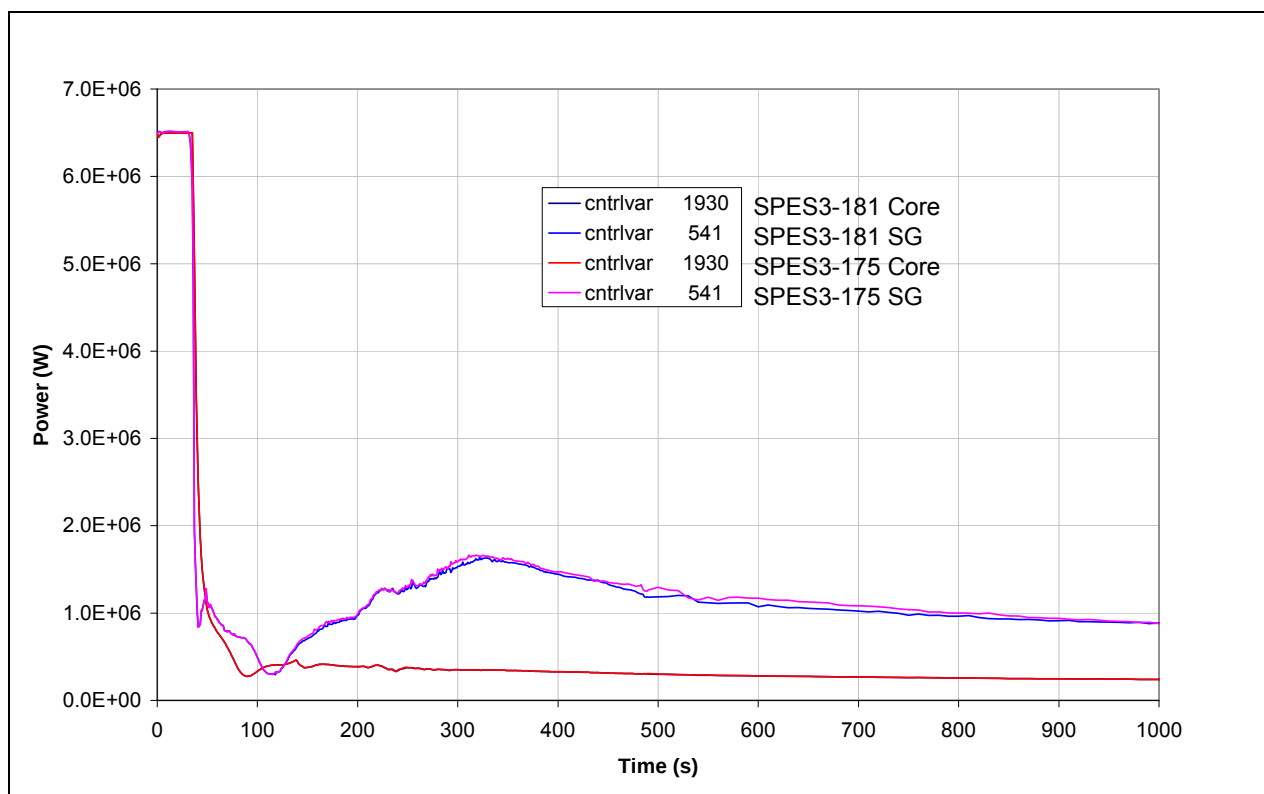
Fig.7. 15 - SPES3-181 and SPES3-175 Core and SG power (window)
