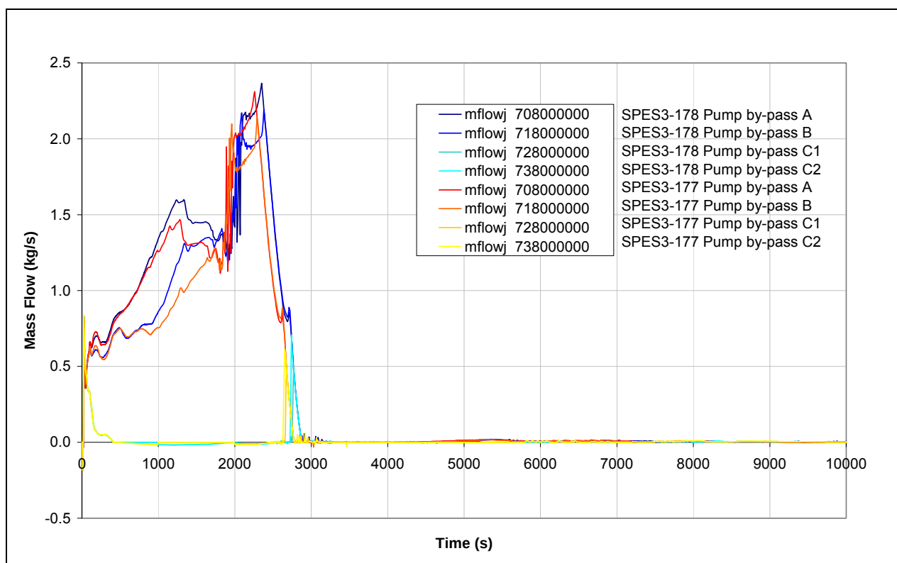
Fig.8. 7 – SPES3-178 and SPES3-177 Pump by-pass mass flow (window)
