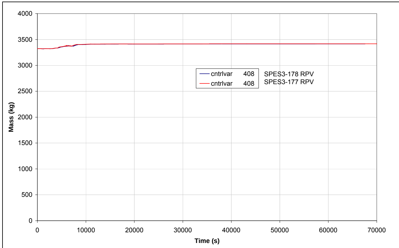
Fig.8. 41 – SPES3-178 and SPES3-177 RPV mass
