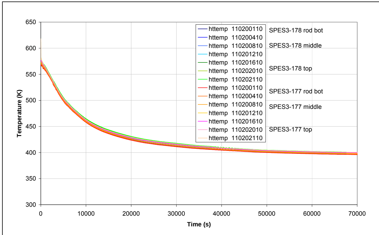
Fig.8. 45 – SPES3-178 and SPES3-177 Core heater rod surface temperature –hot rod
