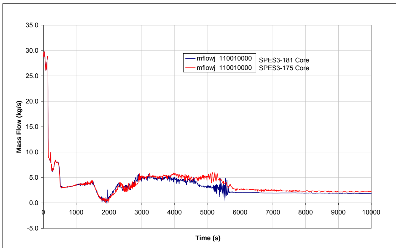
Fig.7. 28 - SPES3-181 and SPES3-175 Core inlet mass flow (window)
