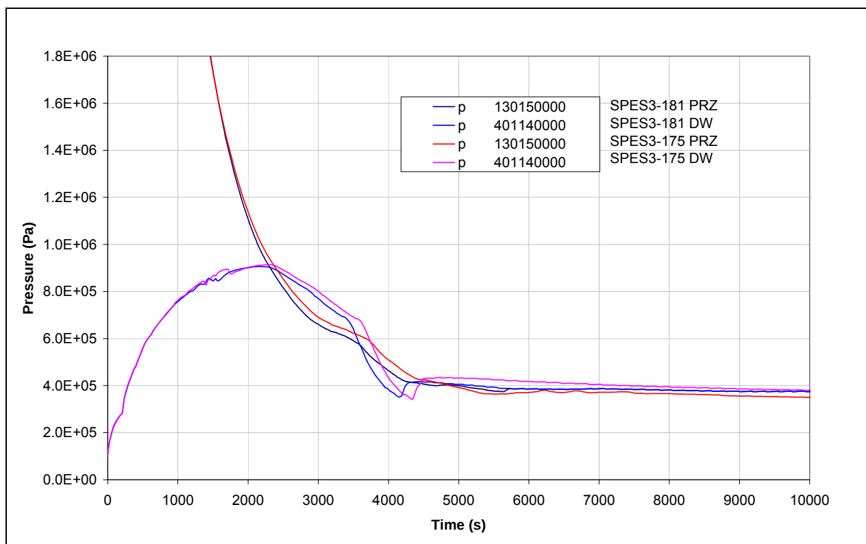
Fig.7. 9 - SPES3-181 and SPES3-175 PRZ and DW pressures (window)
