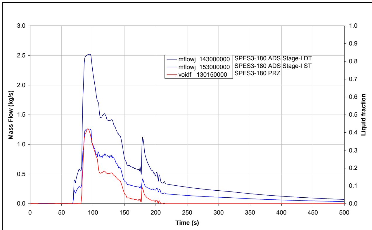
Fig.4.36 – SPES3-180 ADS Stage-I mass flow and PRZ liquid fraction (window)
