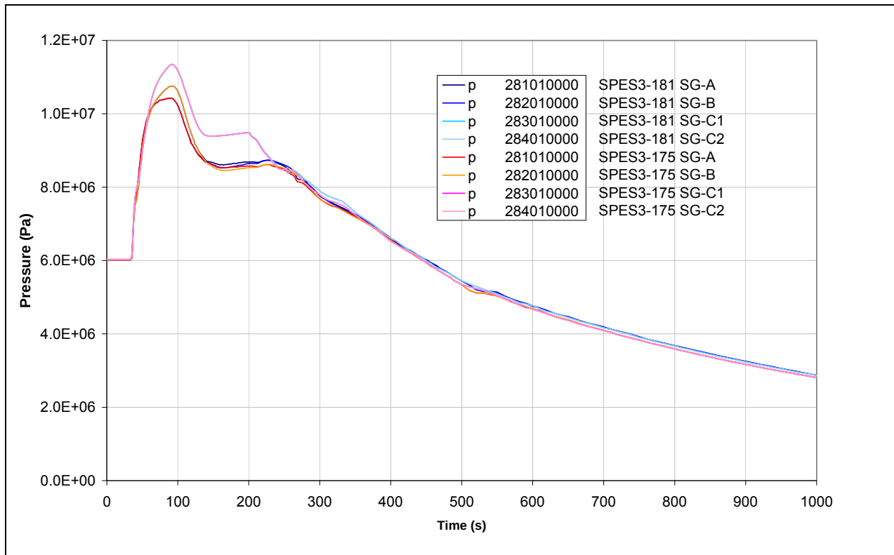
Fig.7. 23 - SPES3-181 and SPES3-175 SG ss outlet pressure (window)
