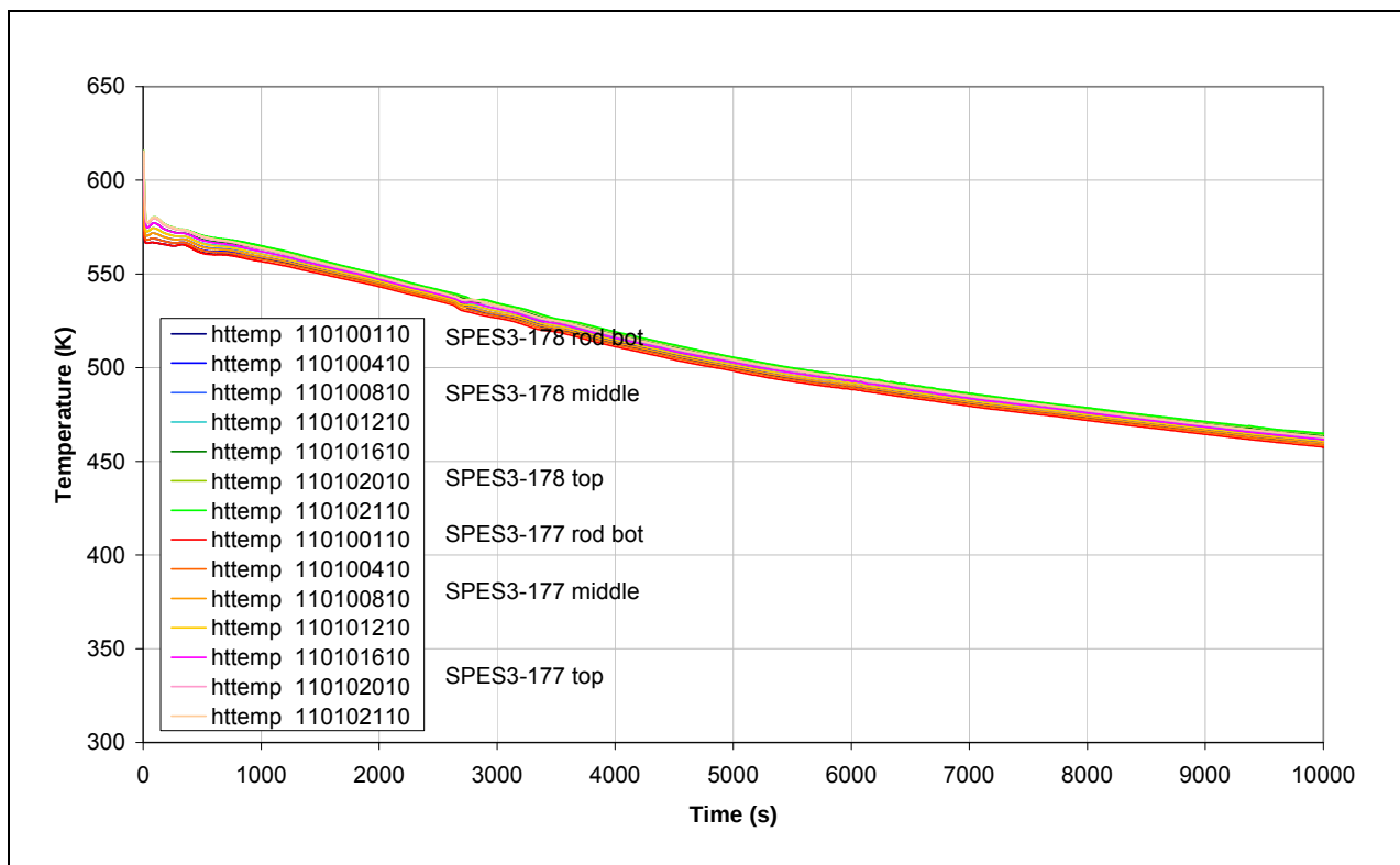
Fig.8. 42 – SPES3-178 and SPES3-177 Core heater rod surface temperature –normal rod (window)
