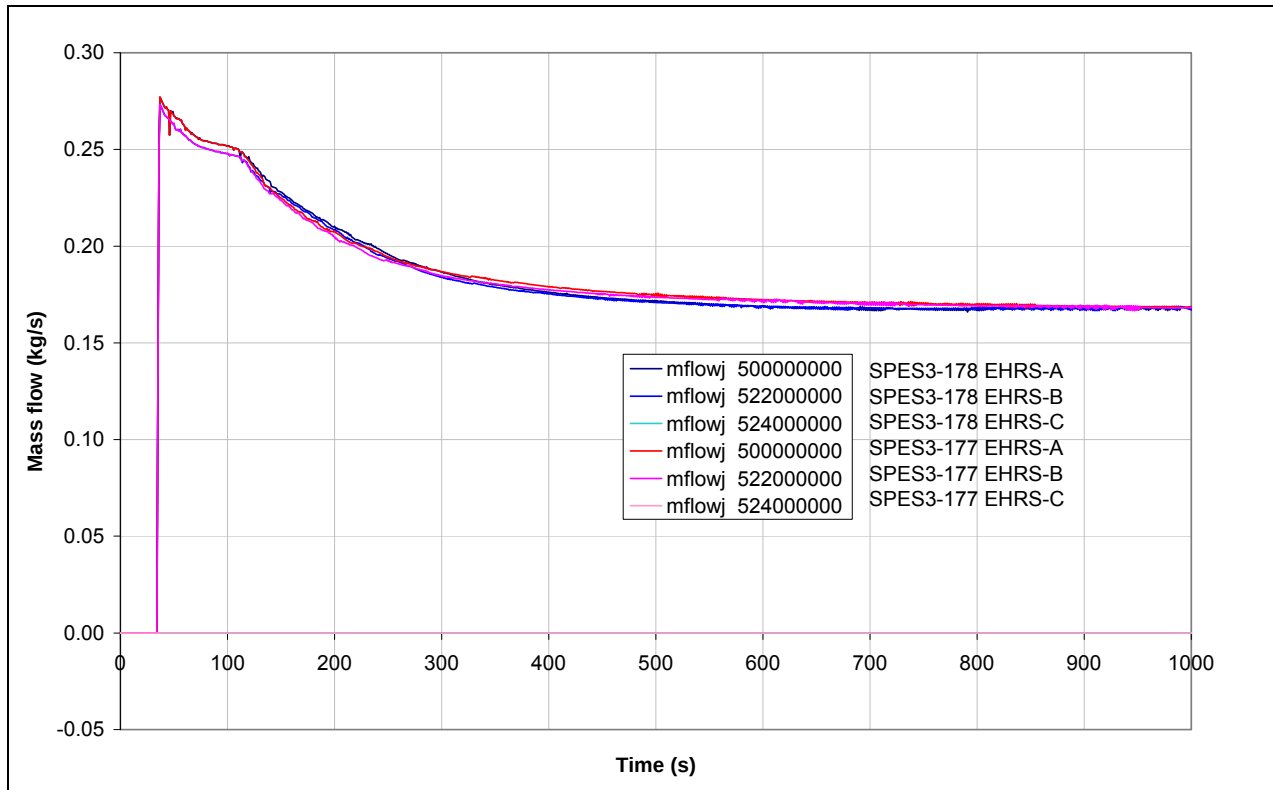
Fig.8. 19 – SPES3-178 and SPES3-177 EHRs cold leg mass flow (window)
