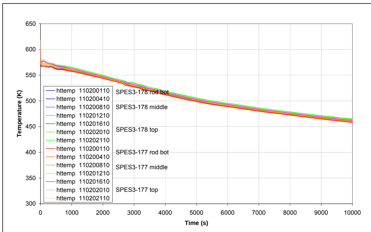
Fig.8. 44 – SPES3-178 and SPES3-177 Core heater rod surface temperature –hot rod (window)
