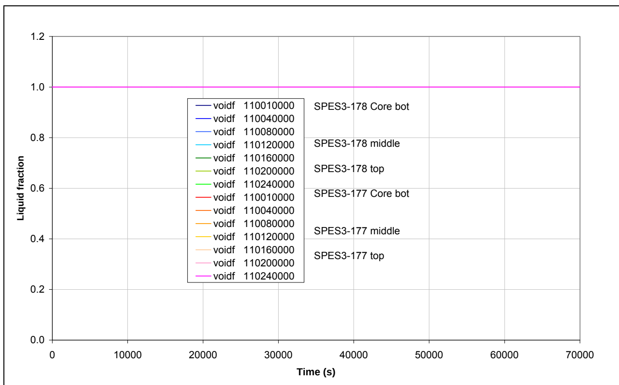
Fig.8. 34 – SPES3-178 and SPES3-177 Core liquid fraction
