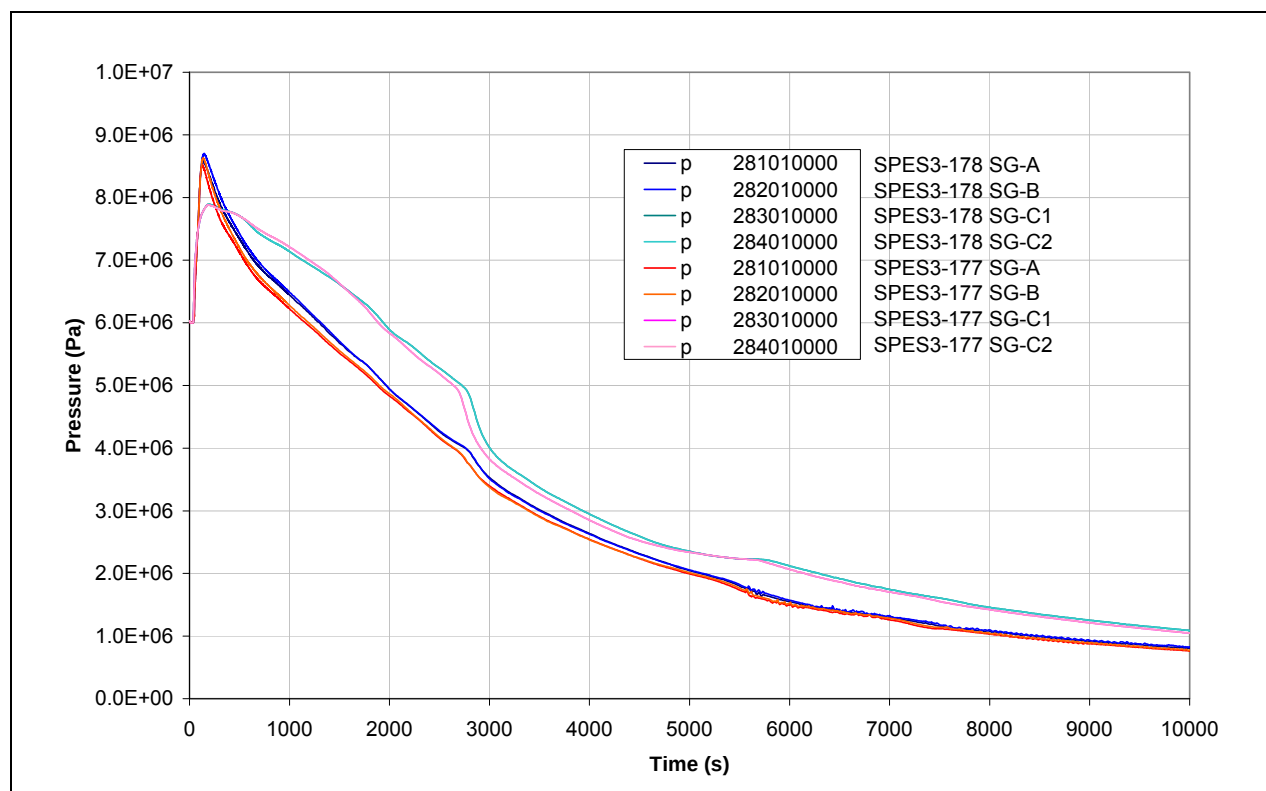
Fig.8. 28 – SPES3-178 and SPES3-177 SG secondary side outlet pressure (window)
