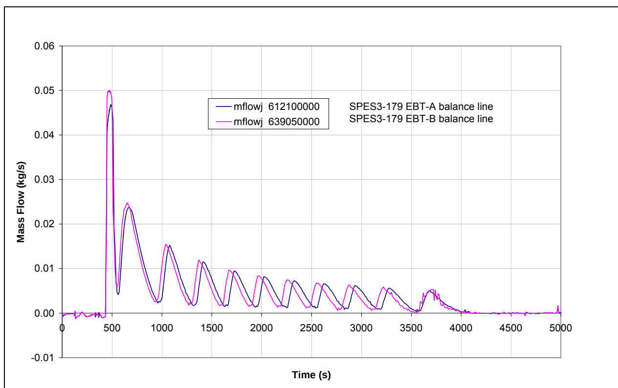
Fig.5. 56 - SPES3-179 EBT to RPV balance line mass flow (window)
