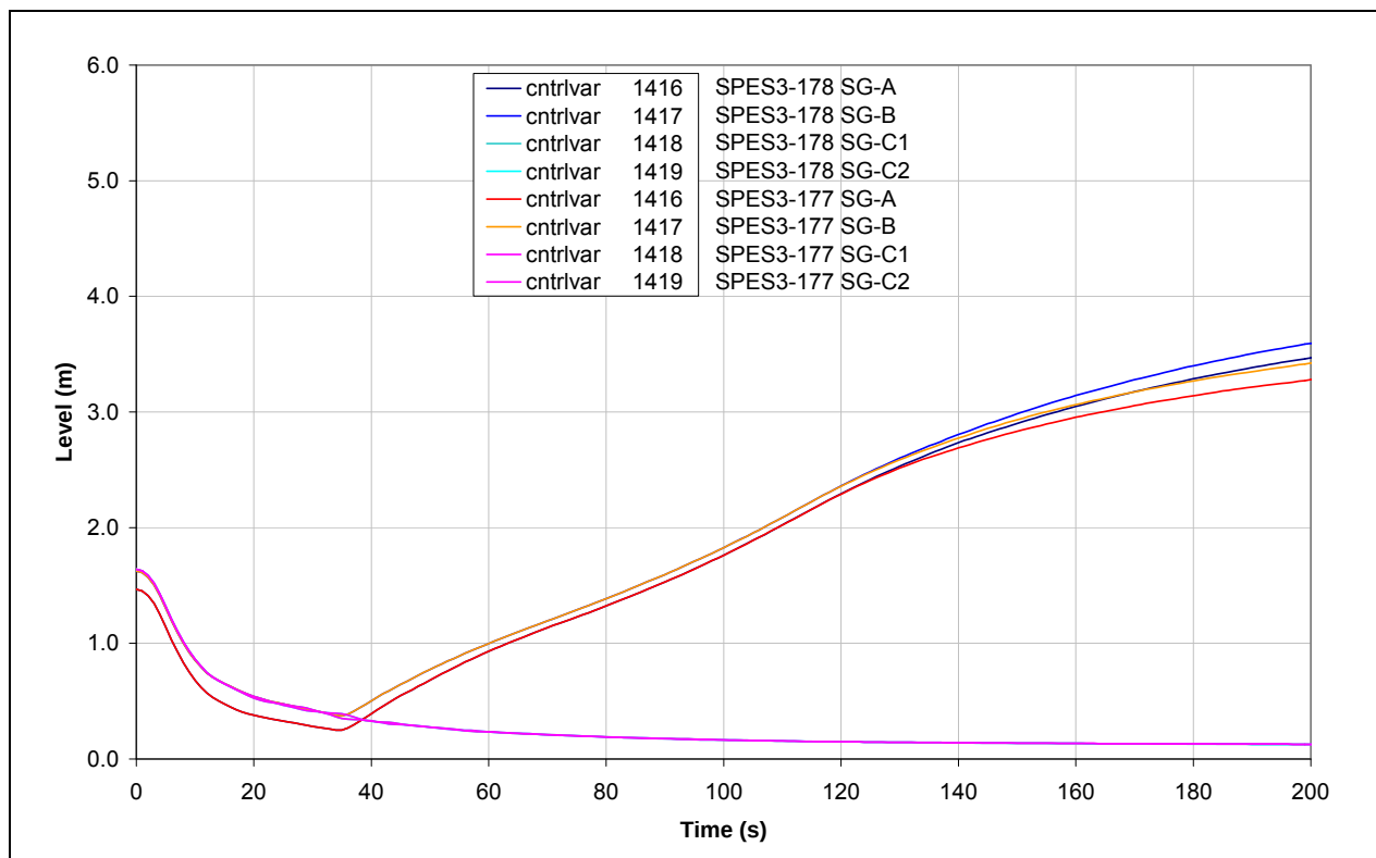
Fig.8. 16 – SPES3-178 and SPES3-177 SG secondary side collapsed level (window)
