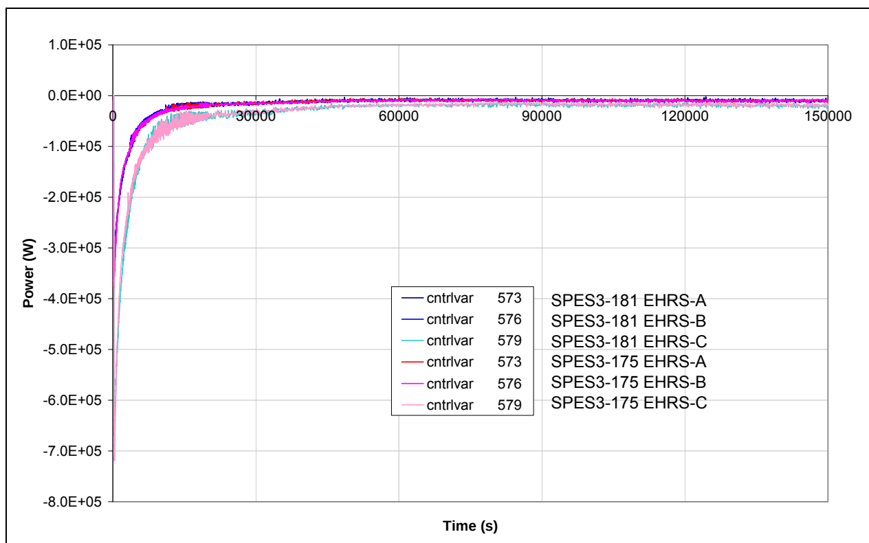
Fig.7. 22 - SPES3-181 and SPES3-175 EHRS power
