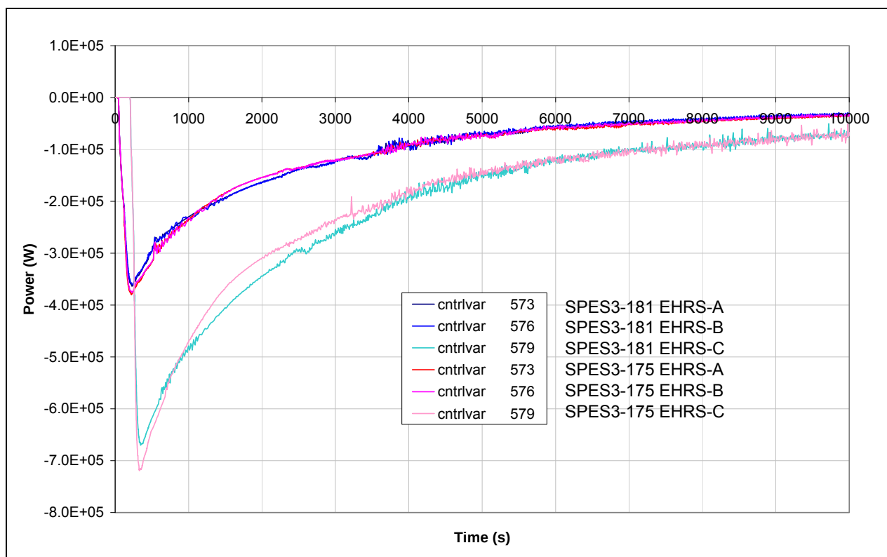
Fig.7. 21 - SPES3-181 and SPES3-175 EHRS power (window)
