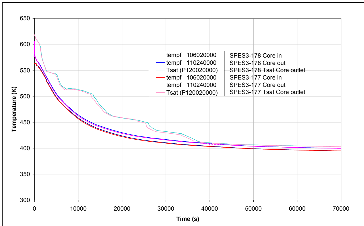
Fig.8. 33 – SPES3-178 and SPES3-177 Core inlet, outlet and saturation temperature
