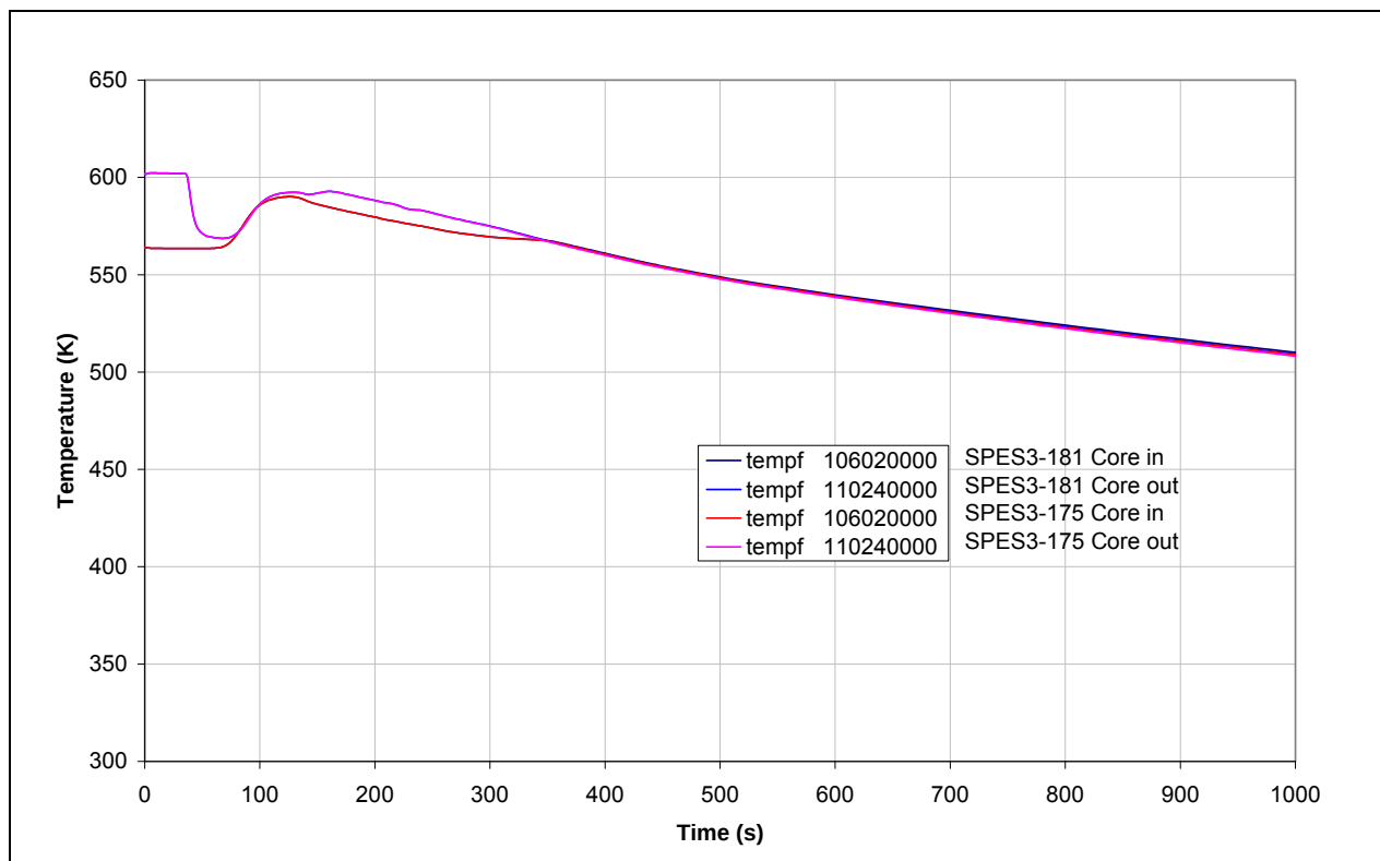
Fig.7. 40 - SPES3-181 and SPES3-175 Core inlet and outlet fluid temperature (window)
