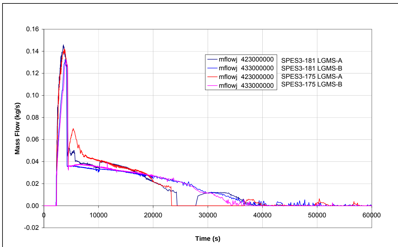
Fig.7. 46 - SPES3-181 and SPES3-175 LGMS injection mass flow (window)
