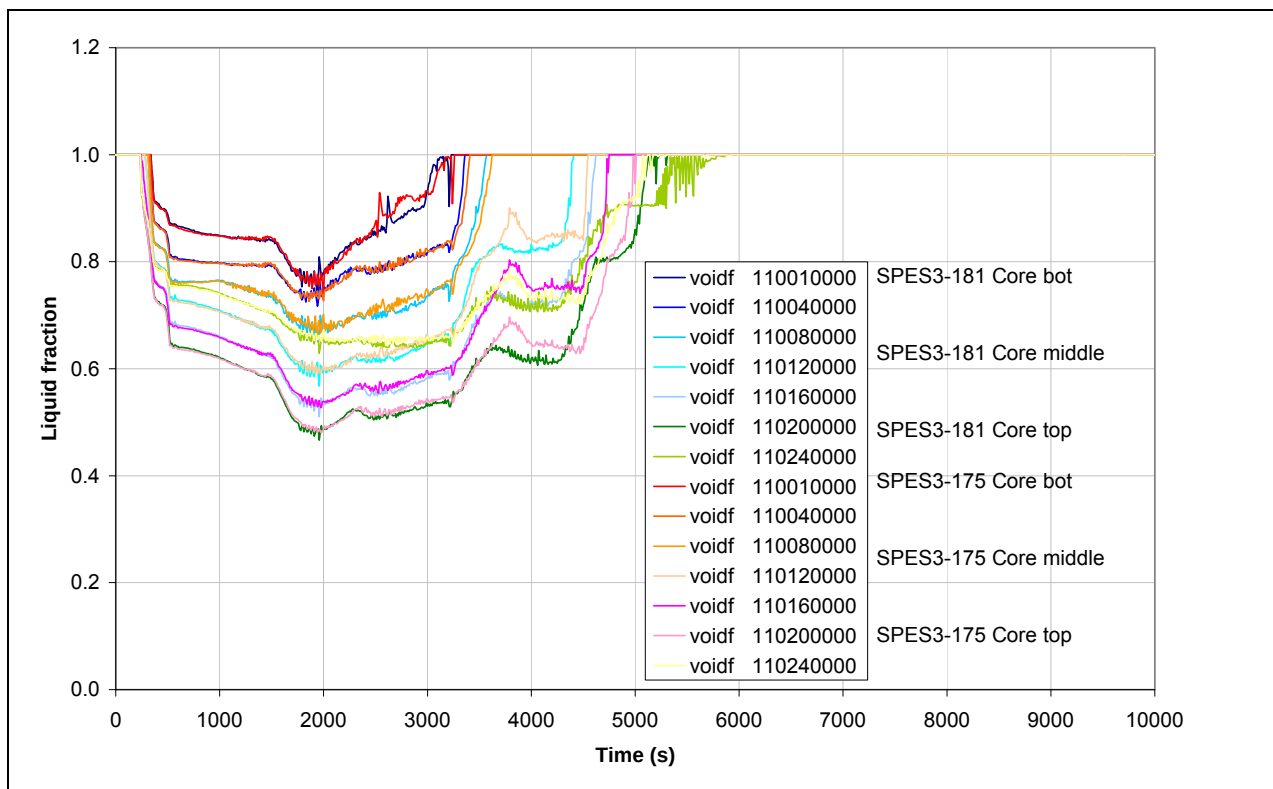
Fig.7. 34 - SPES3-181 and SPES3-175 Core liquid fraction (window)
