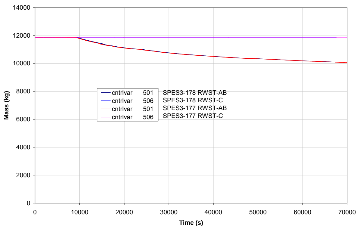
Fig.8. 24 – SPES3-178 and SPES3-177 RWST mass
