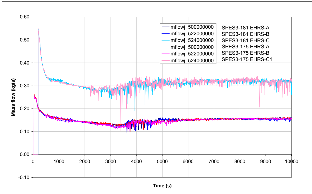
Fig.7. 19 - SPES3-181 and SPES3-175 EHRS cold leg mass flow (window)
