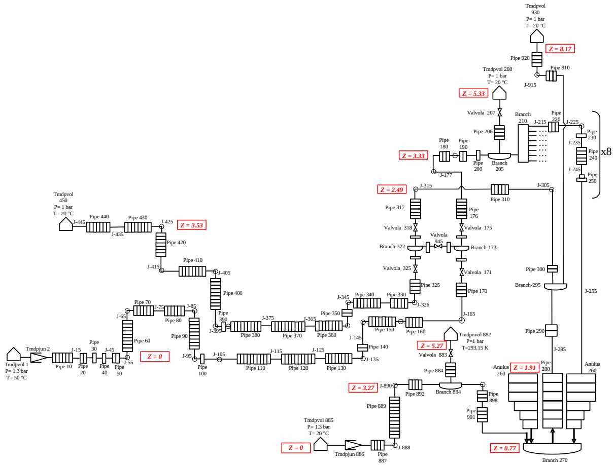
Figure 3.1: RELAP5 Nodalization.
