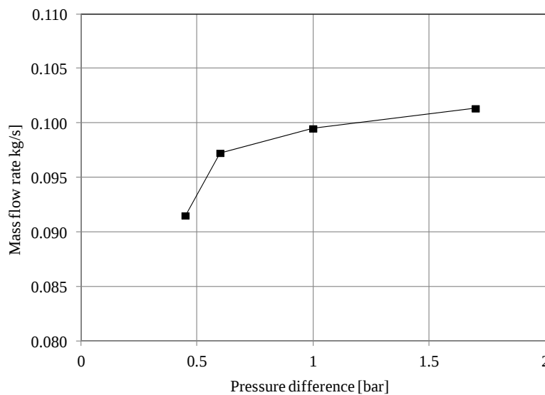
Figure 2.6: Calibration curve obtained for the DVI flow rate regulator.
