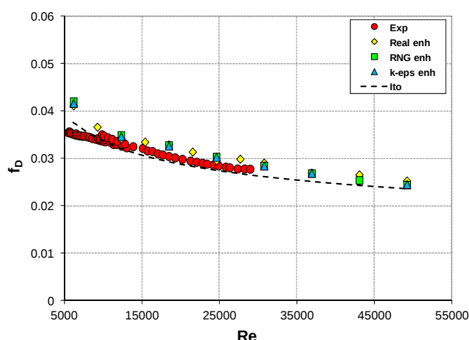
Figure 10 - Comparison between experimental data, Ito correlation and k-\varepsilon models with enhanced wall treatment for the SIET pipe.
