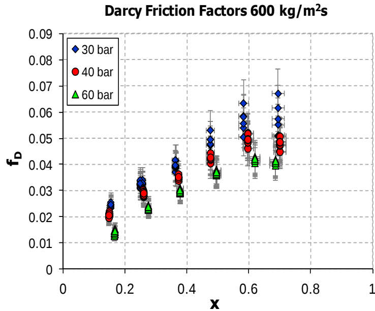
Fig. 6. Experimental friction coefficients at 600 kg/m 2 s.
