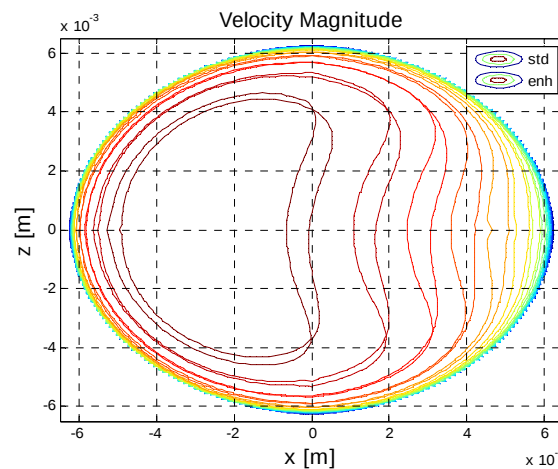
Figure 14 - Velocity magnitude profiles calculated with the realizable k-\varepsilon model with enhanced wall treatment and standard wall function.
