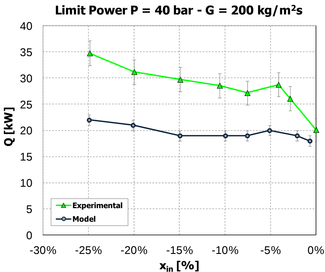
Fig. 24. Comparison between theoretical model and experiment in terms of limit power [ P = 40 bar; G = 200 kg/m 2 s].
