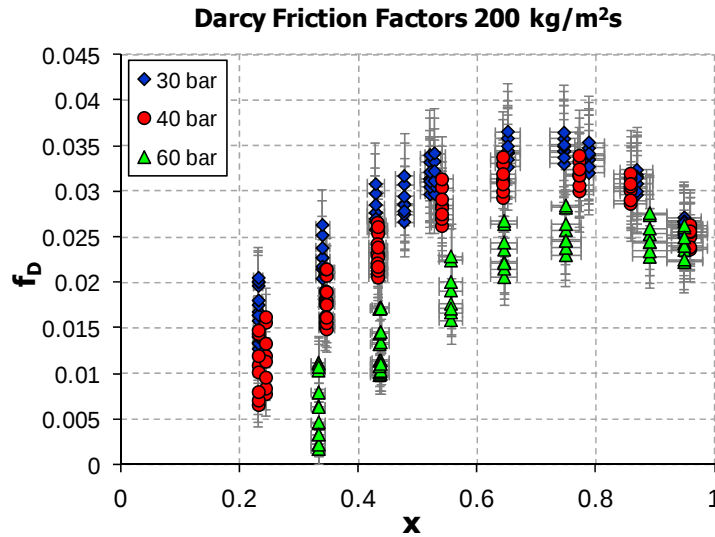
Fig. 4 Experimental friction coefficients at 200 kg/m²s.
