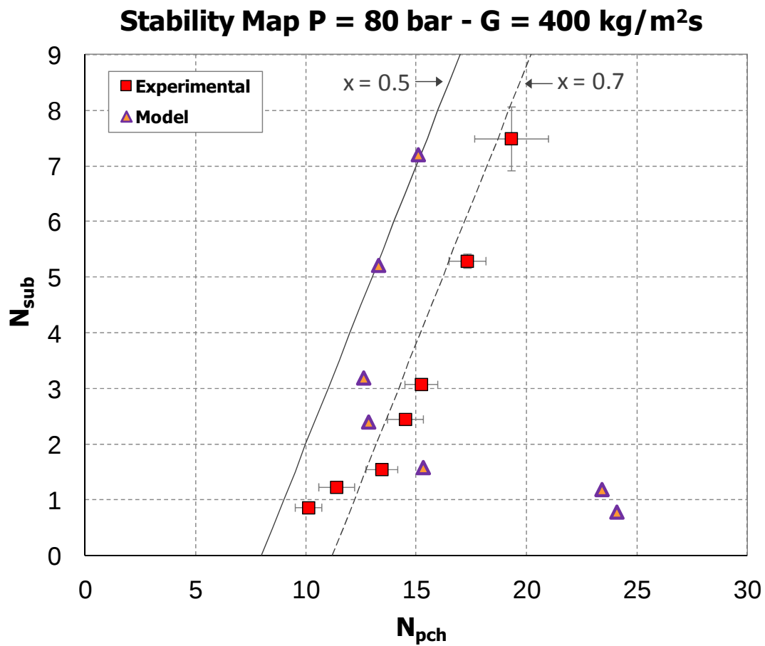
Fig. 22. Comparison between theoretical model and experiment in terms of stability map [ P = 80 bar; G = 400 kg/m 2 s].
