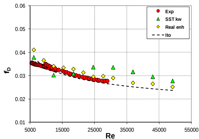
Figure 12 - Comparison between experimental data, Ito correlation, realizable k-\varepsilon model with enhanced wall treatment and SST k-\omega model for the SIET pipe.
