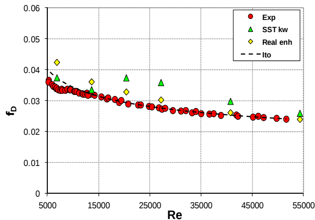
Figure 13 - Comparison between experimental data, Ito correlation, realizable k-\varepsilon model with enhanced wall treatment and SST k-\omega model for Coil6.
