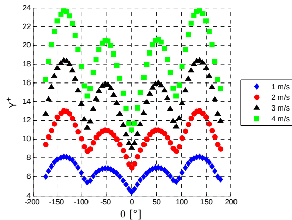
Figure 18 – Circumferential y^+ profile for the realizable k-\varepsilon model with standard wall function.
