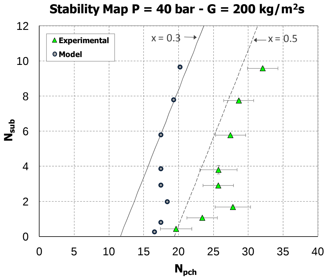
Fig. 21. Comparison between theoretical model and experiment in terms of stability map [ P = 40 bar; G = 200 kg/m 2 s].
