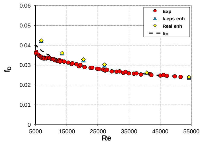
Figure 11 - Comparison between experimental data, Ito correlation, standard k-\varepsilon model and realizable k-\varepsilon model with enhanced wall treatment for Coil6.
