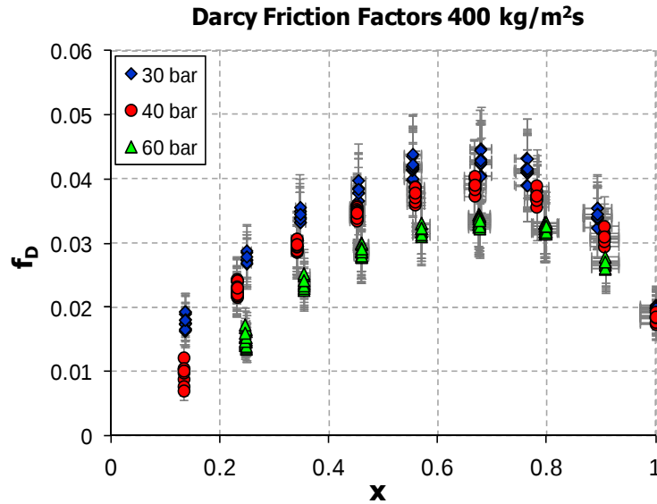
Fig. 5. Experimental friction coefficients at 400 kg/m²s.
