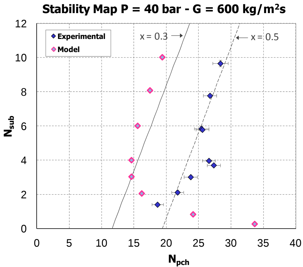
Fig. 20. Comparison between theoretical model and experiment in terms of stability map [ P = 40 bar; G = 600 kg/m 2 s].
