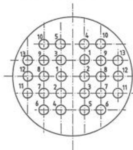
Fig.3. 28 – SPES-2 Steam Generator U-tubes
