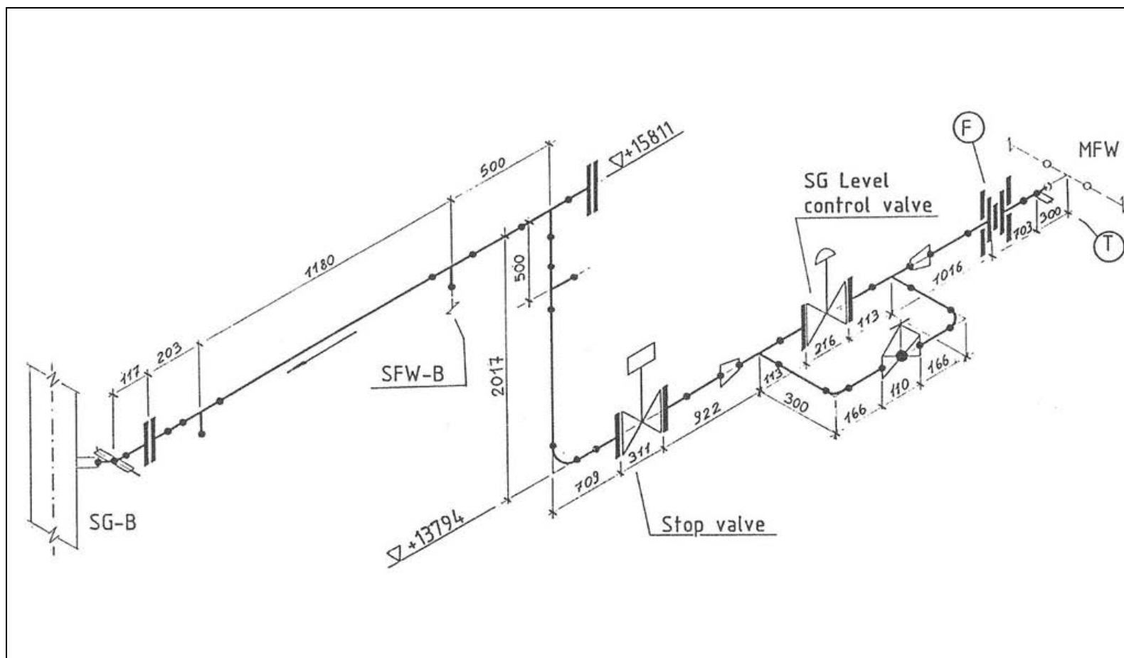
Fig.3. 33 – SPES-2 Main feedwater line-B
