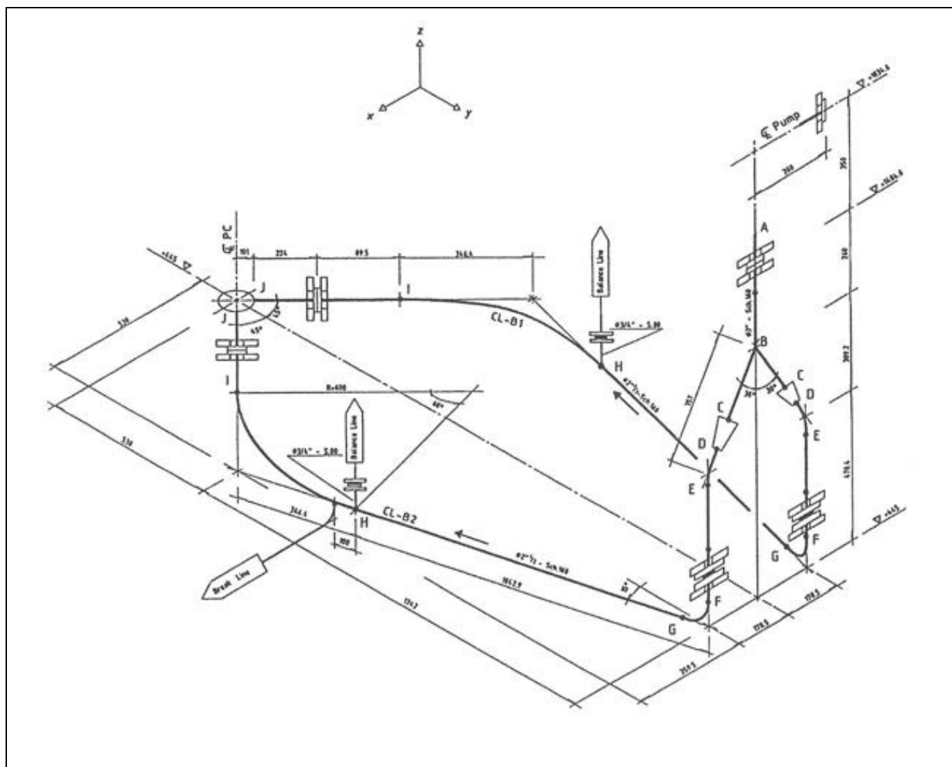
Fig.3. 19 – SPES-2 Cold Leg-B layout
