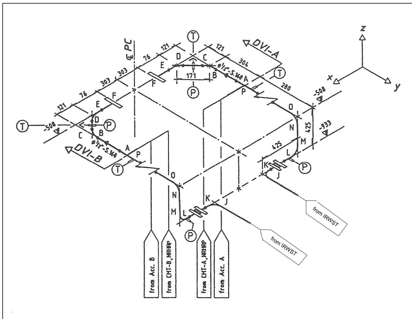
Fig.3. 23 – SPES-2 DVI-A and DVI-B line layout
