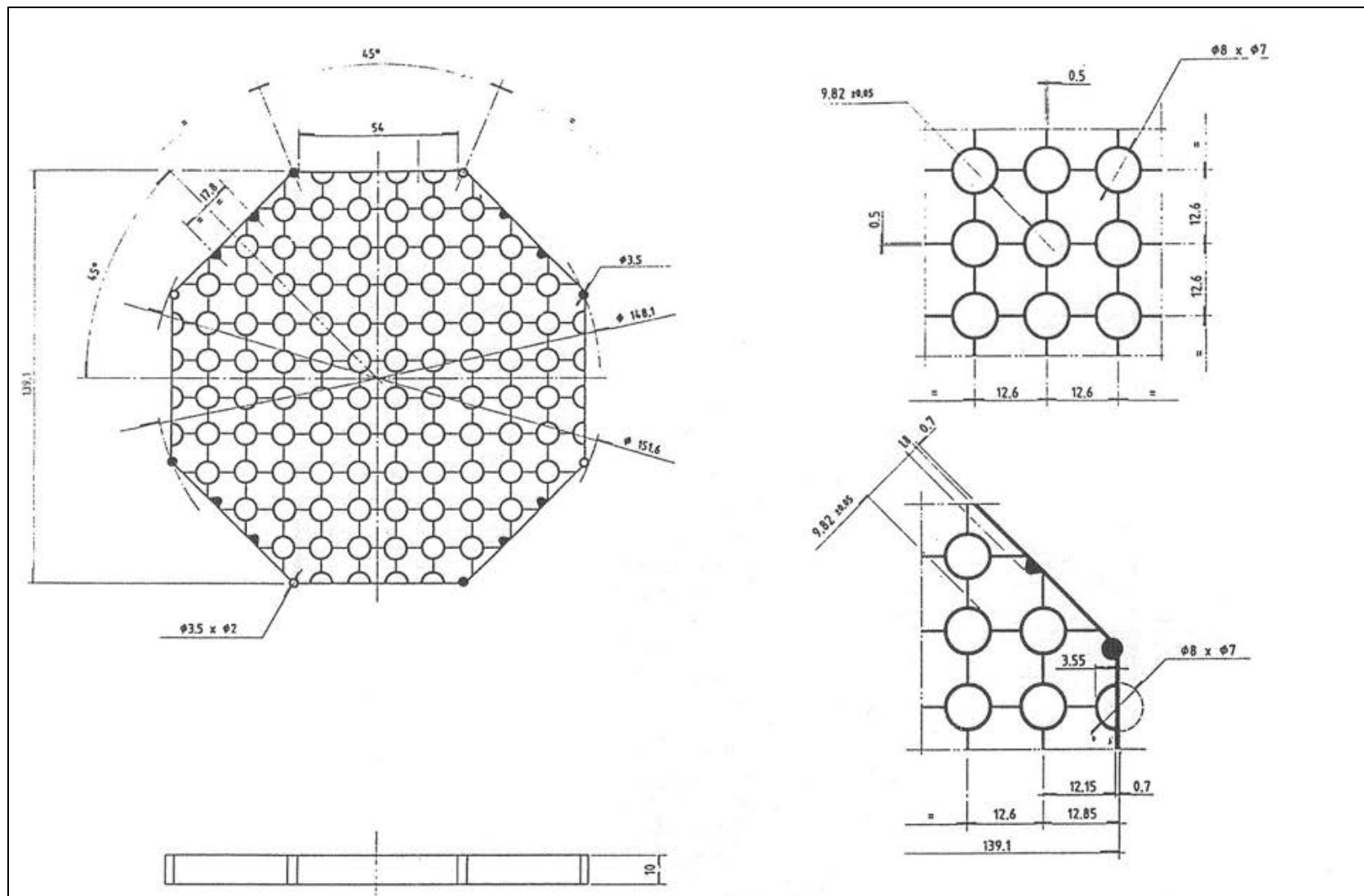
Fig.3. 15 – SPES-2 power channel: rod bundle spacer grid
