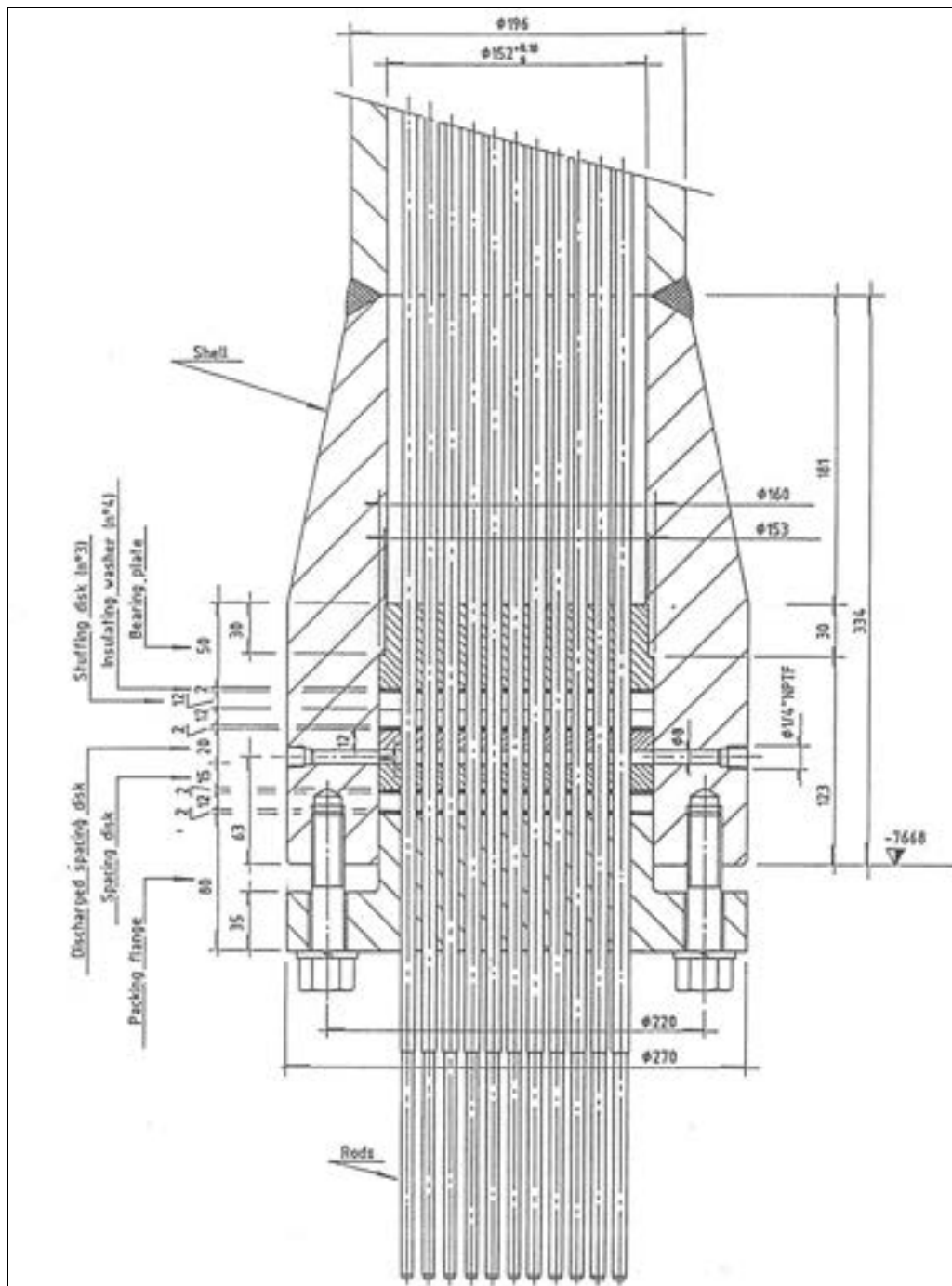
Fig.3. 9 – SPES-2 power channel: lower plenum sealing system
