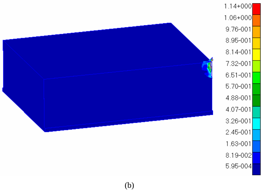
Figures 16 a, b: Penetration depth at the beginning of penetration (a) and perforation (b)
