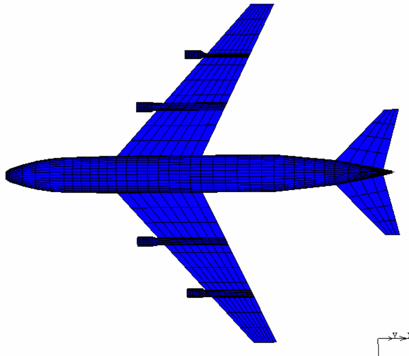
Figure 12 – View of the Boeing 747 FE model
