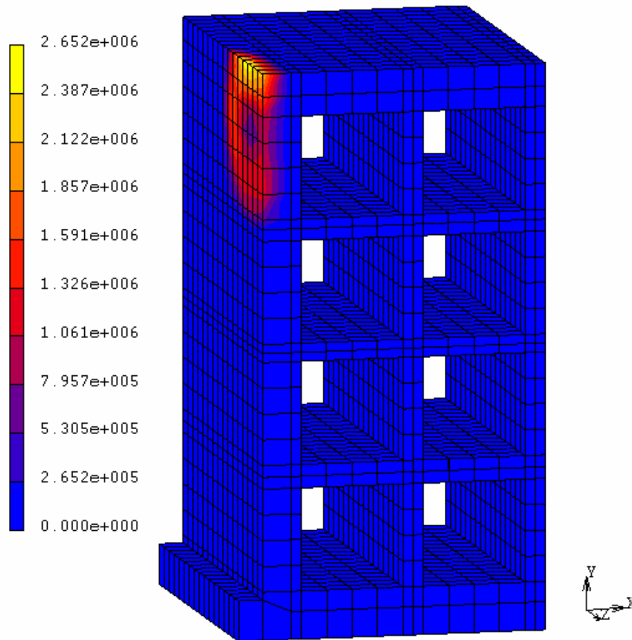
Figure 23: Von Mises stress distribution in the storage cell substructure after 5 s fire
