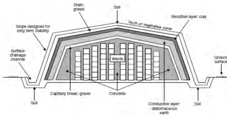
Figure 3: An engineered disposal mound based on the multi-barrier concept [26]
