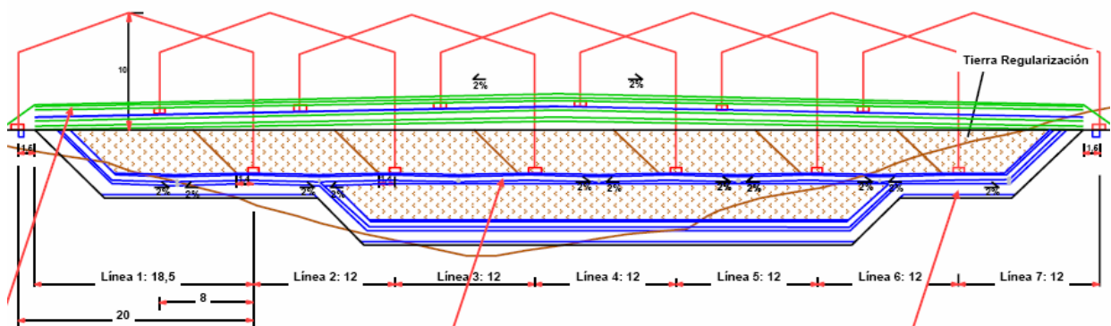
Figure 10: General scheme of platform [courtesy of ENRESA]
