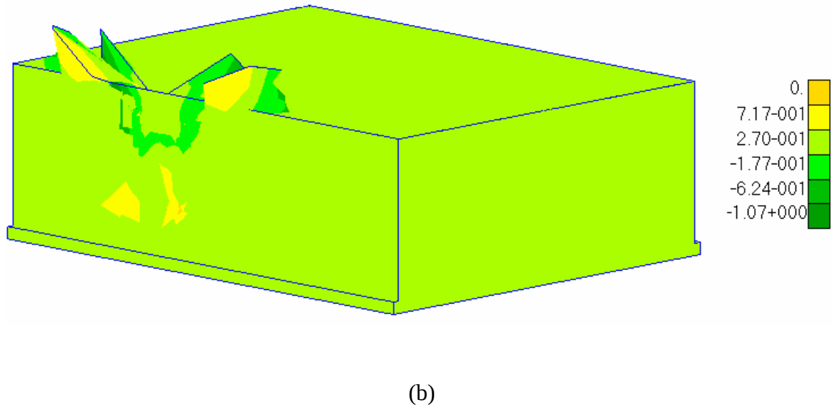
Figures 17 a, b: Penetration depth at the beginning of penetration (a) and perforation (b)
