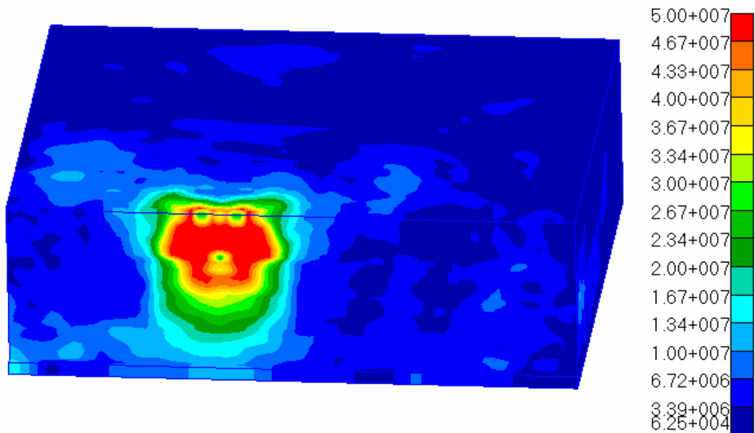
Figure 18: Von Mises stress distribution in the case of impact on the middle of RWsC cell
