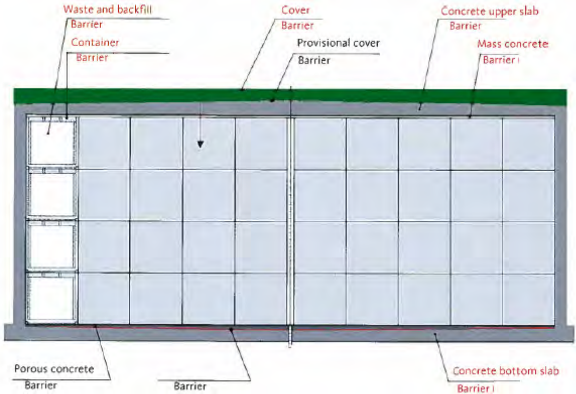
Figure 11: Scheme of the possible storage cell disposition [courtesy of ENRESA]
